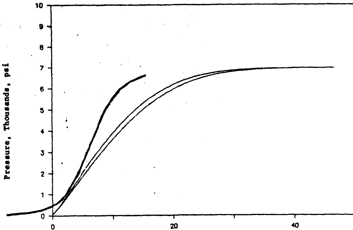
Figure 5a. Pressure as Function of Burning Time. Upper Curve - GOEX 75-44 Experimental Data, Middle Curve - Calculated Response of Five Spheres, and Lower Curve - Calculated Response of Five Ellipsoids
