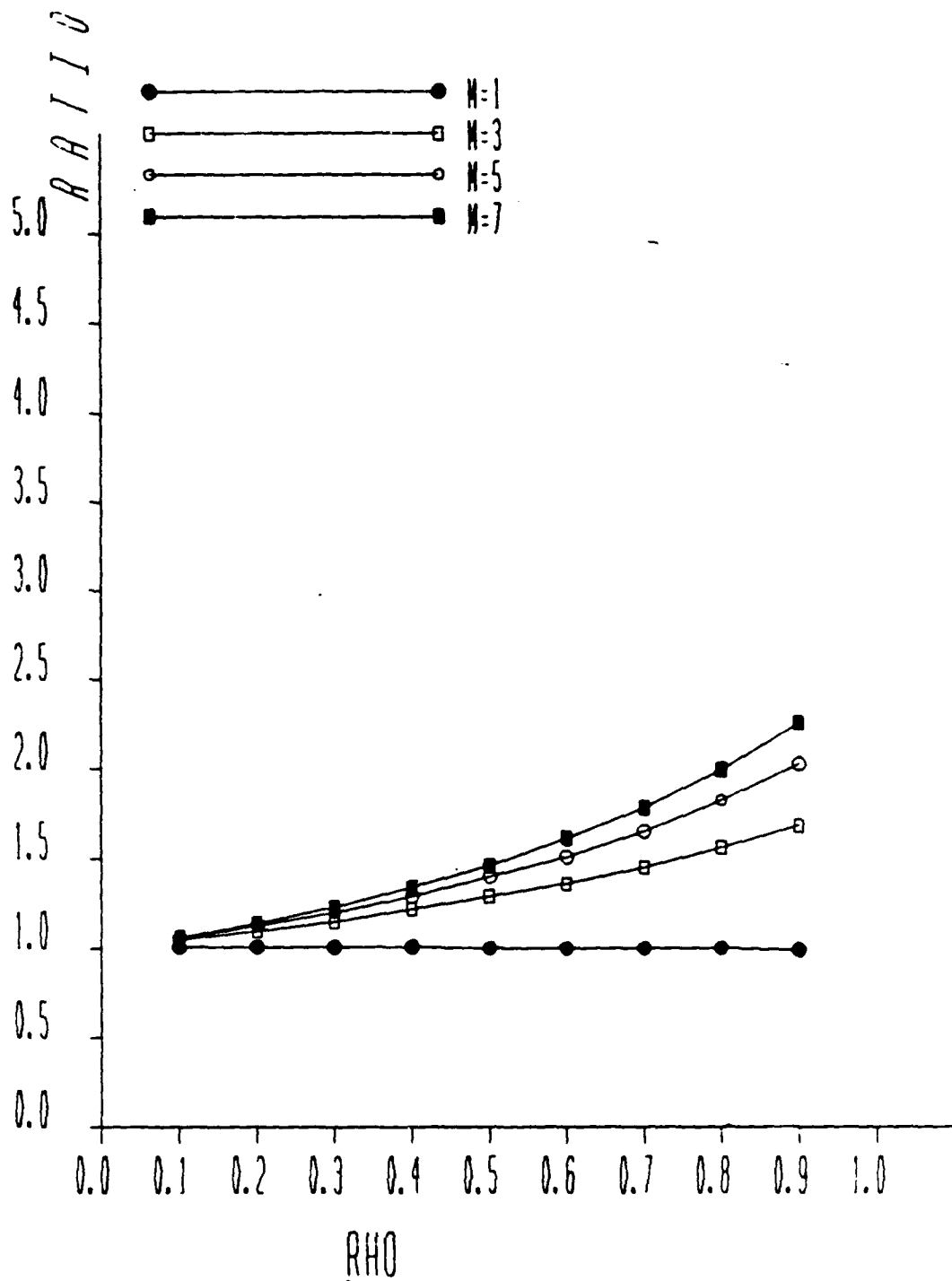
FIGURE 3 FCFS/TASK
