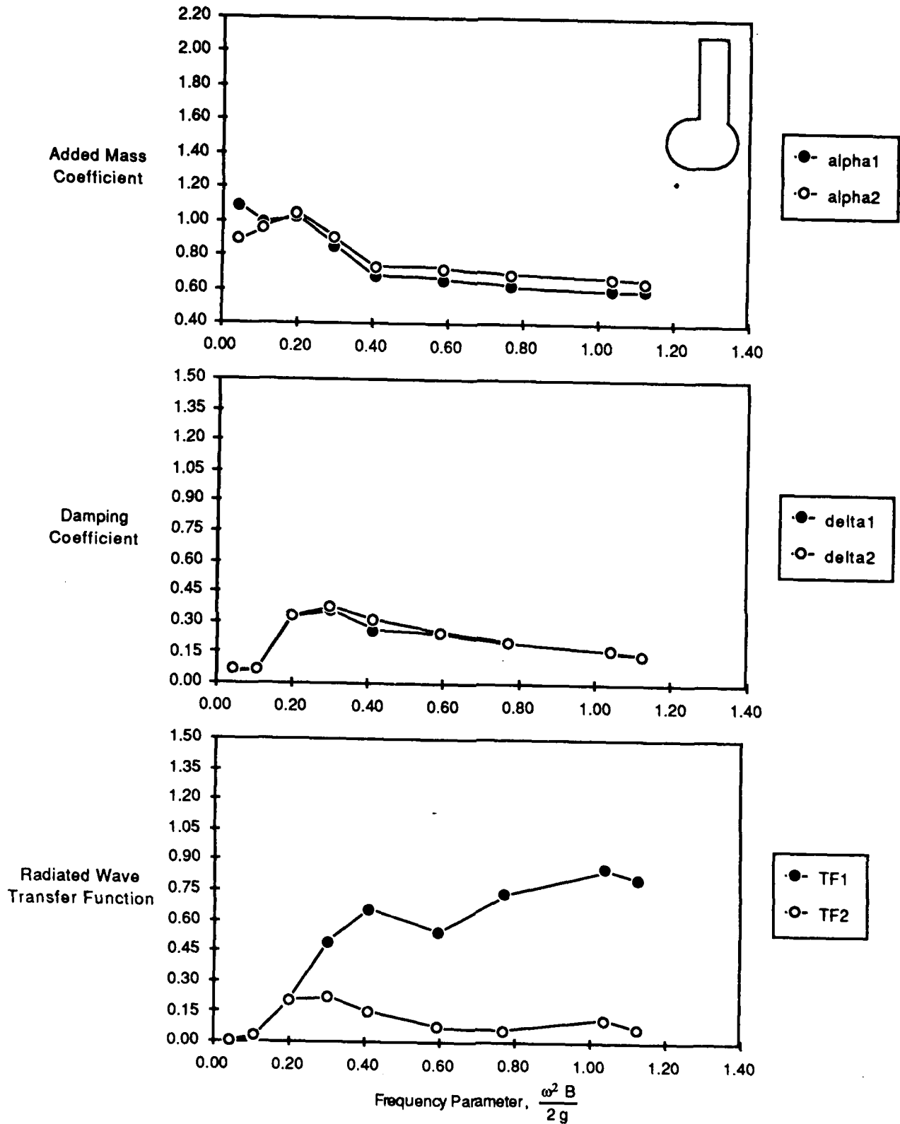
Fig. E2. Data for model E, half golf club at design draft, for 1 inch (2.54 cm) oscillation amplitude.
