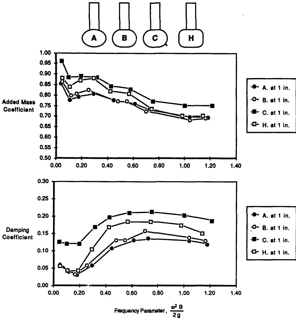
Fig. 7. Effects of lower hull shape and bilge keel on added mass and damping as shown by models A, B, C, and H at design draft, 1.0 inch (2.54 cm) oscillation amplitude.
