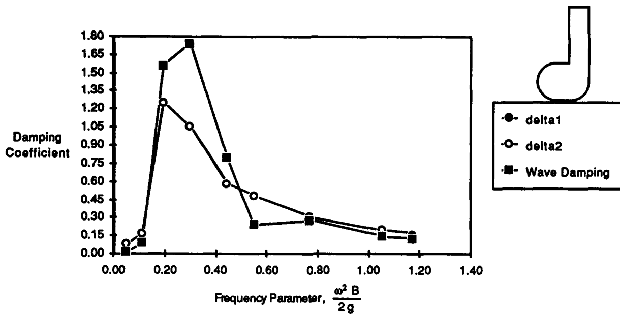
Fig. 17. Comparison of the damping coefficients calculated from the force measurements (delta1, delta2) and radiated waves ("Wave Damping") for model F, at design draft, and 1.0 inch (2.54 cm) amplitude.
