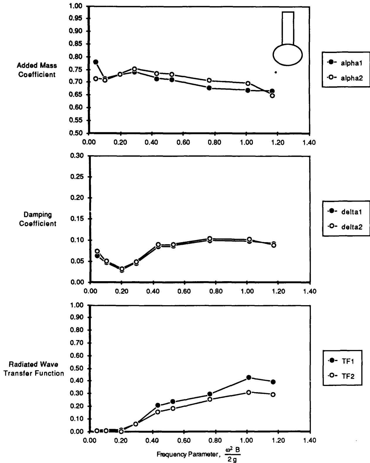
Fig. A4. Data for model A, true ellipse at deep draft, for 1 inch (2.54 cm) oscillation amplitude.
