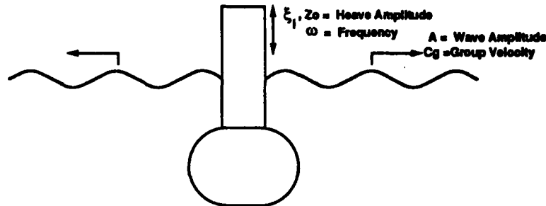
Fig. 10. Radiated waves from vertical oscillation of a two-dimensional body.
