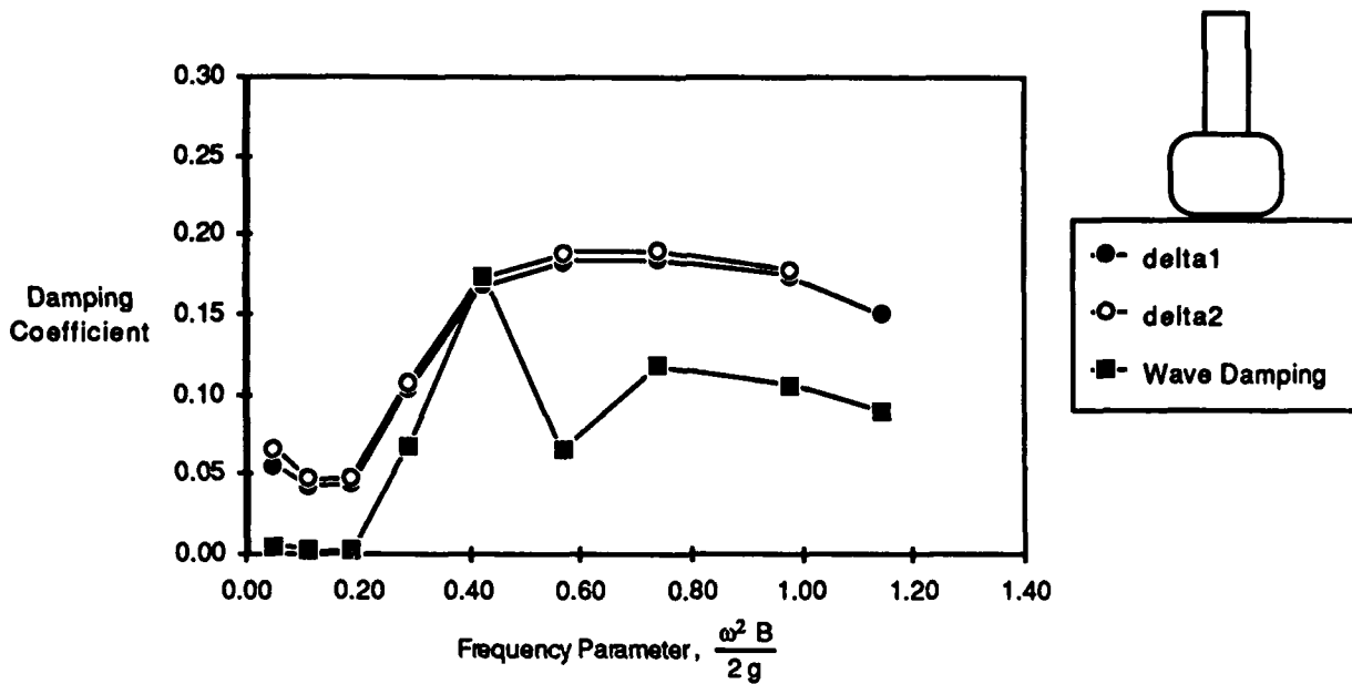
Fig. 18. Comparison of the damping coefficients calculated from the force measurements (delta1, delta2) and radiated waves ("Wave Damping") for model G, at design draft, and 1.0 inch (2.54 cm) amplitude.
