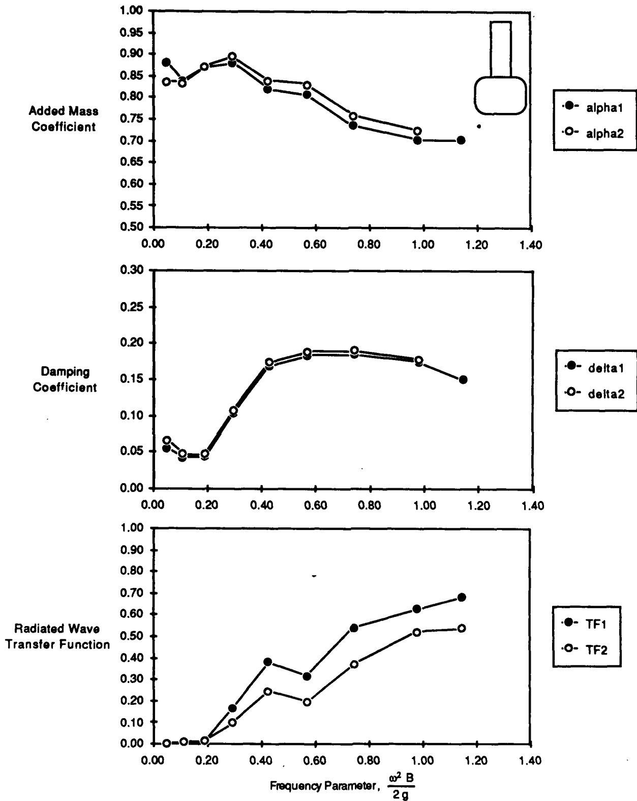
Fig. H2. Data for model H, raddised rectangle at design draft, for 1 inch (2.54 cm) oscillation amplitude.
