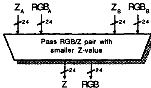
Figure 3. Z-comparator / multiplexing device
