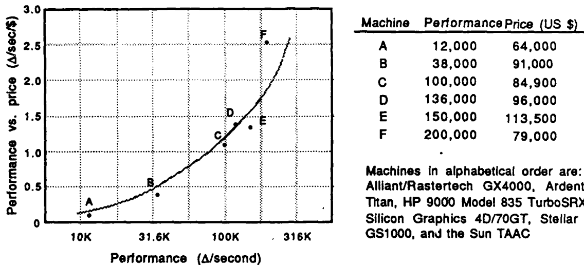
Figure 4. Performance/price ratios for representative systems 2
