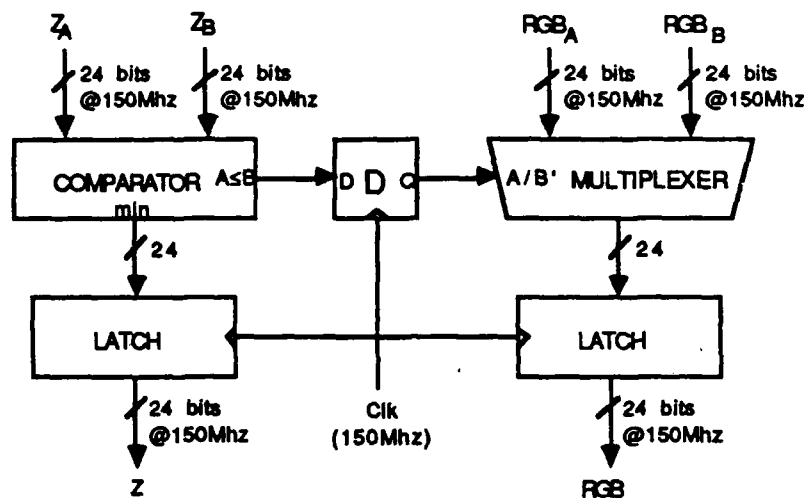
Figure 4. Pipelined Z-comparator / multiplexing device
