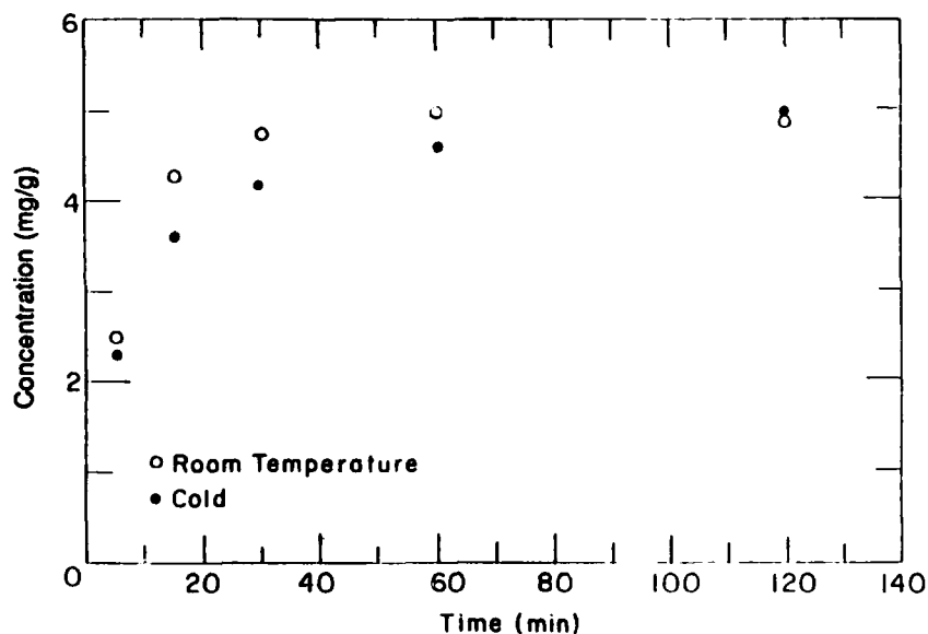
Figure 5. Kinetics study: Extraction of Minneapolis soil with methanol at room temperature and at 0°C.
