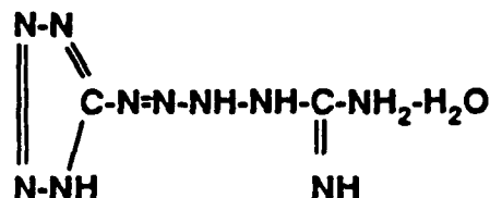
Figure 1. Structure of tetrazene.
