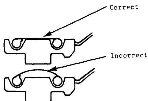
Figure A-20. Loading the film.
