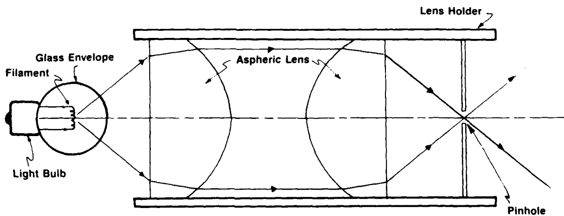
Figure 6. The condenser.
