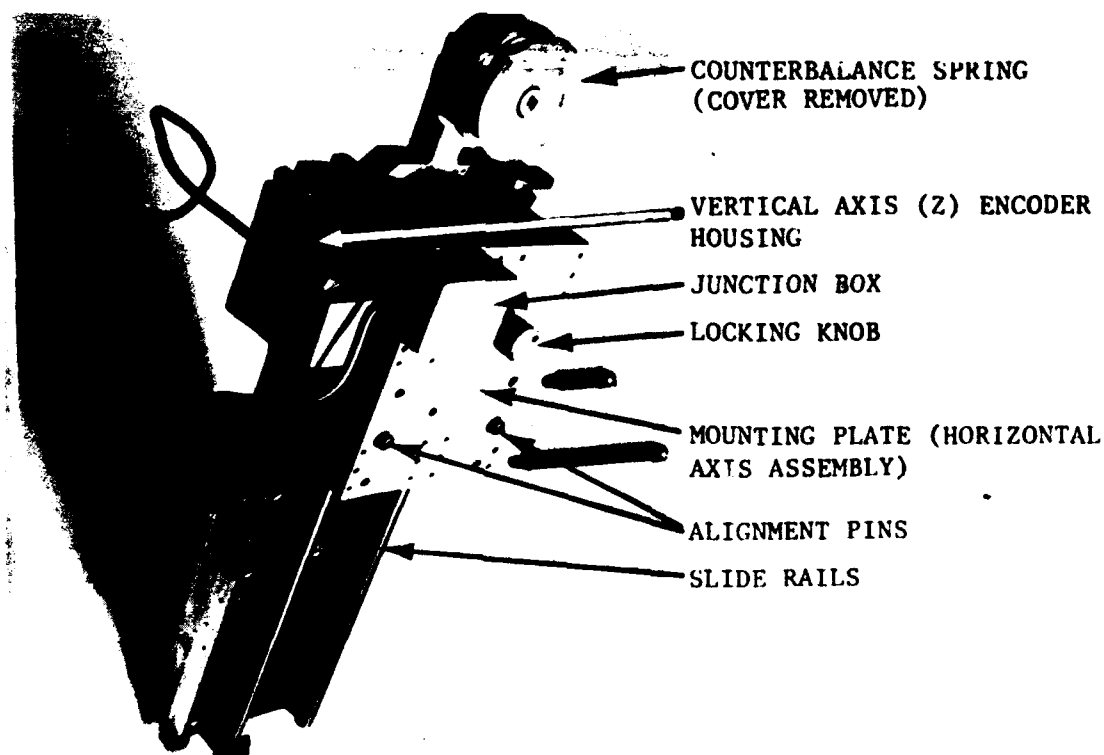
Figure D-7. The vertical axis assembly.
