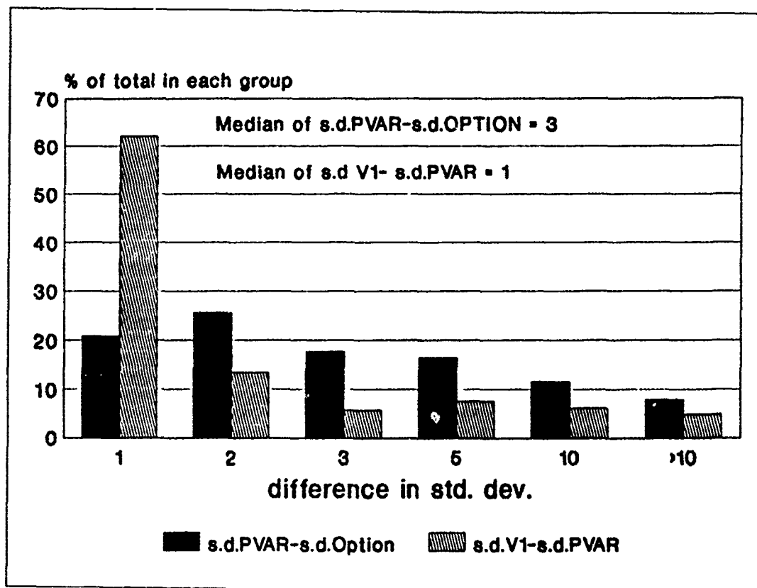
Figure 3 - Difference in standard deviations between variance formulae.
