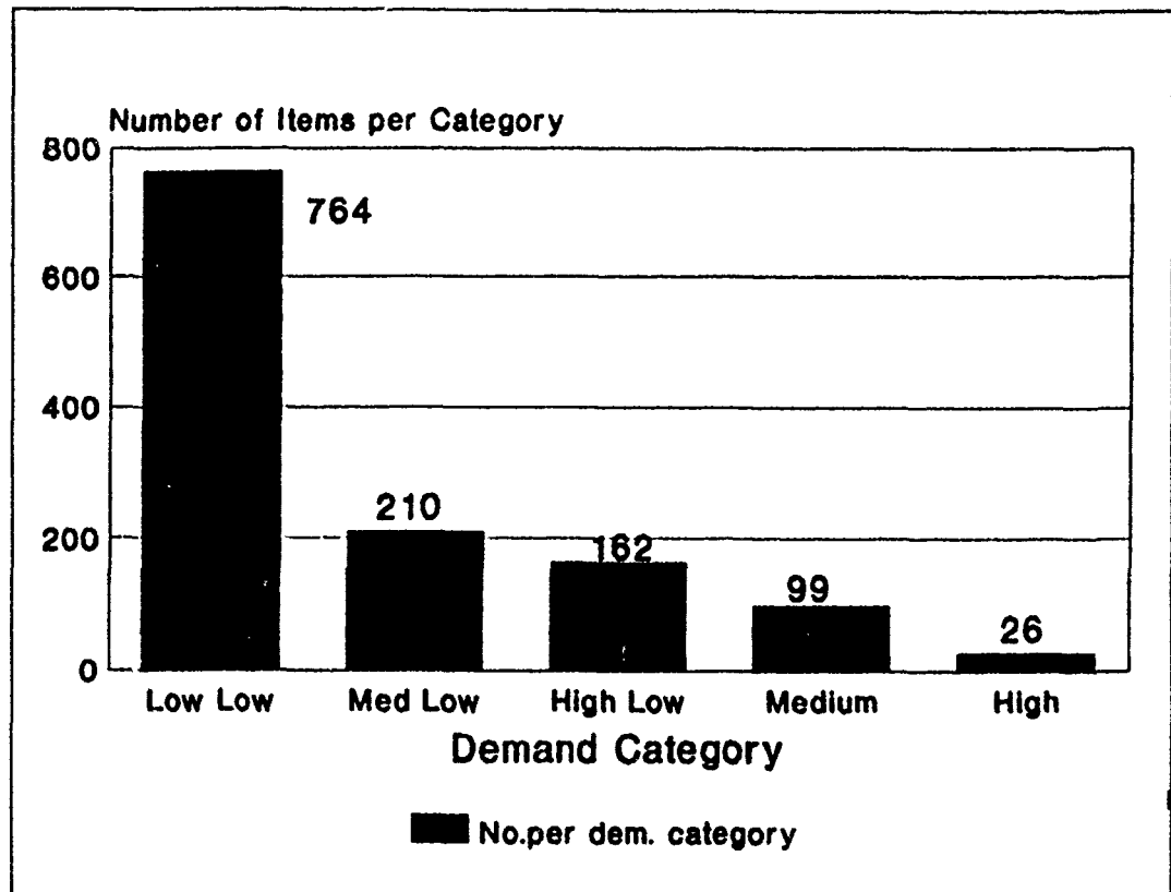
Figure 1 - Distribution of the 1261 items by quarterly demand category.
