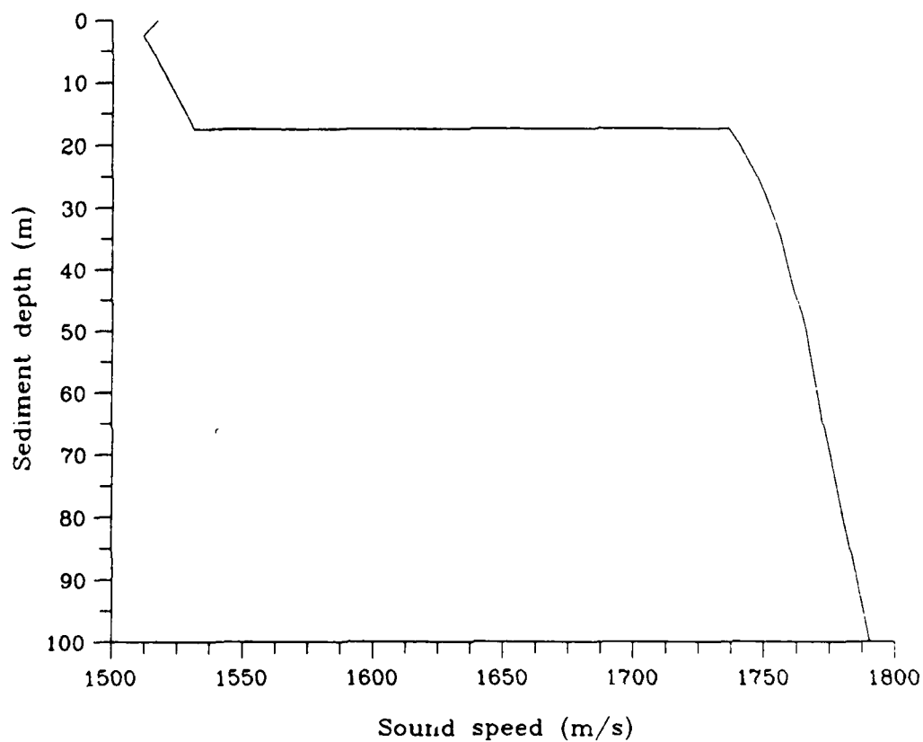
Figure 4-20: Sound speed profile for the Corpus Christi area based on geologic information.
