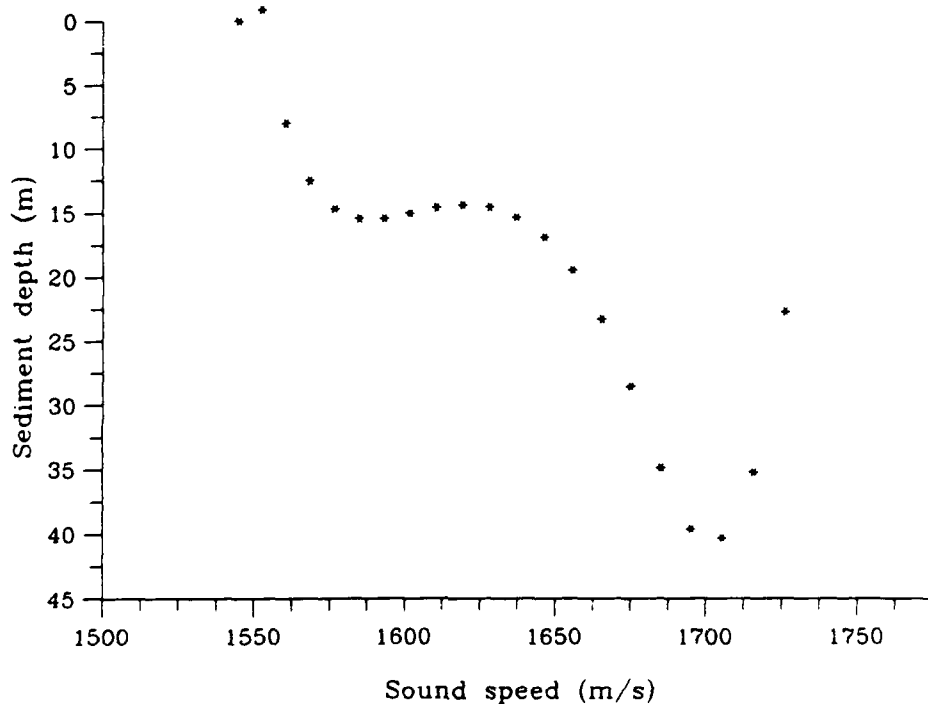
Figure 4-21: Corpus Christi area sediment sound speed profile obtained using all seven eigenvalues at 50 Hz and 140.05 Hz.
