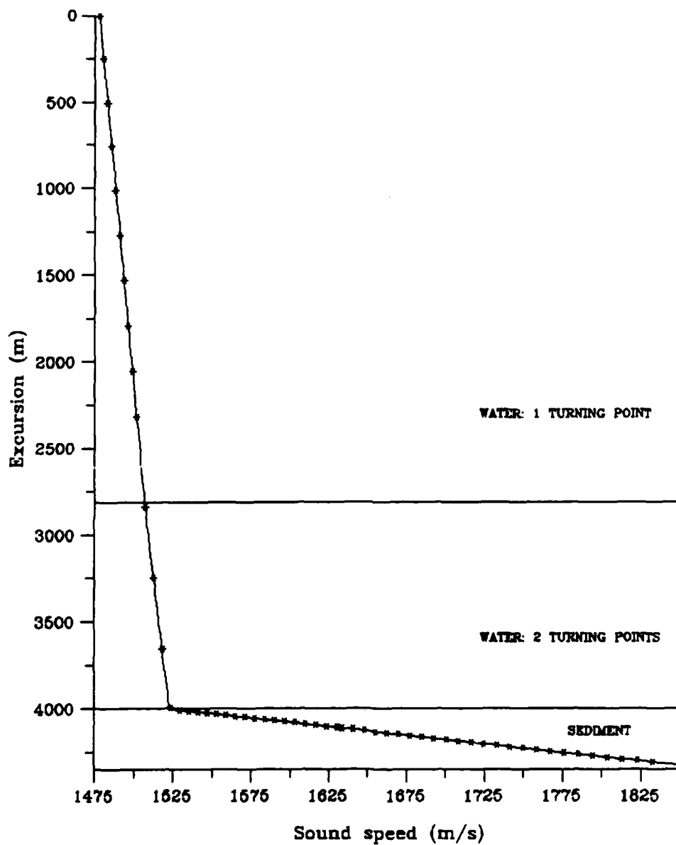
Figure 3-16: Excursion versus depth for the bilinear profile. Below 2813 meters this curve is the sound speed profile. A frequency of 140 Hz was used for this inversion to provide bottom interacting modes.
