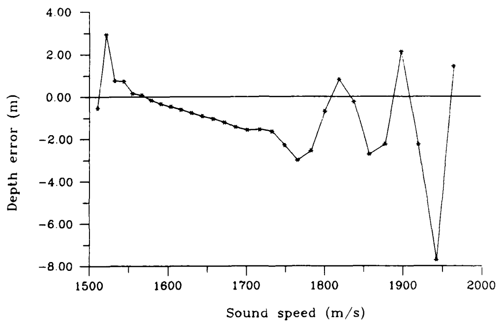
Figure 4-11: Depth error for inversion method 1 (least squares splines) applied to waveguide model 2.
