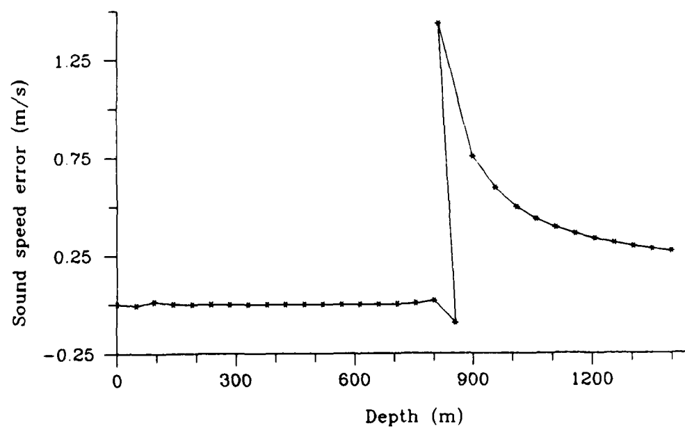
Figure 3-27: Sound speed error for the n^2(z) linear profile with mode 25 eigenvalue removed, and higher modes incorrectly identified.
