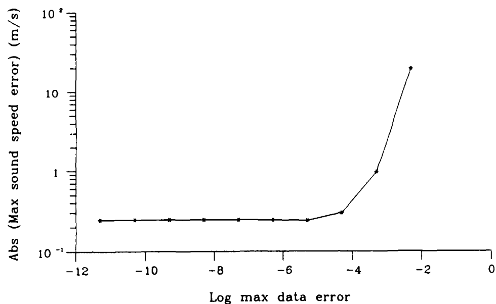
Figure 3-26: Absolute value of the maximum error for inversion method 2 using smoothing splines with noisy data.
