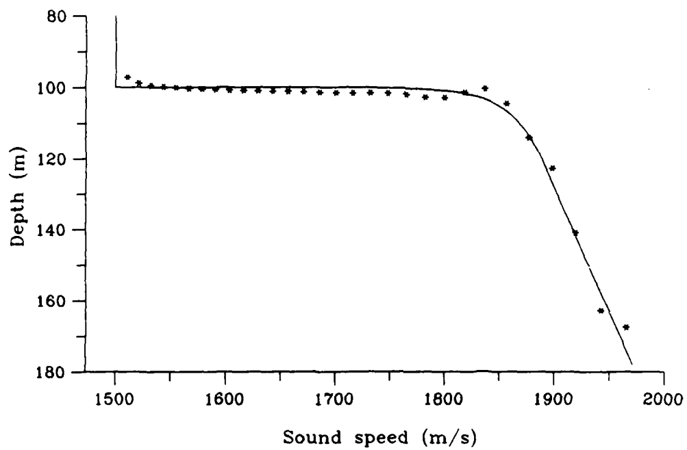
Figure 4-14: Inversion results for waveguide model 2 using inversion method 2 (least squares splines).
