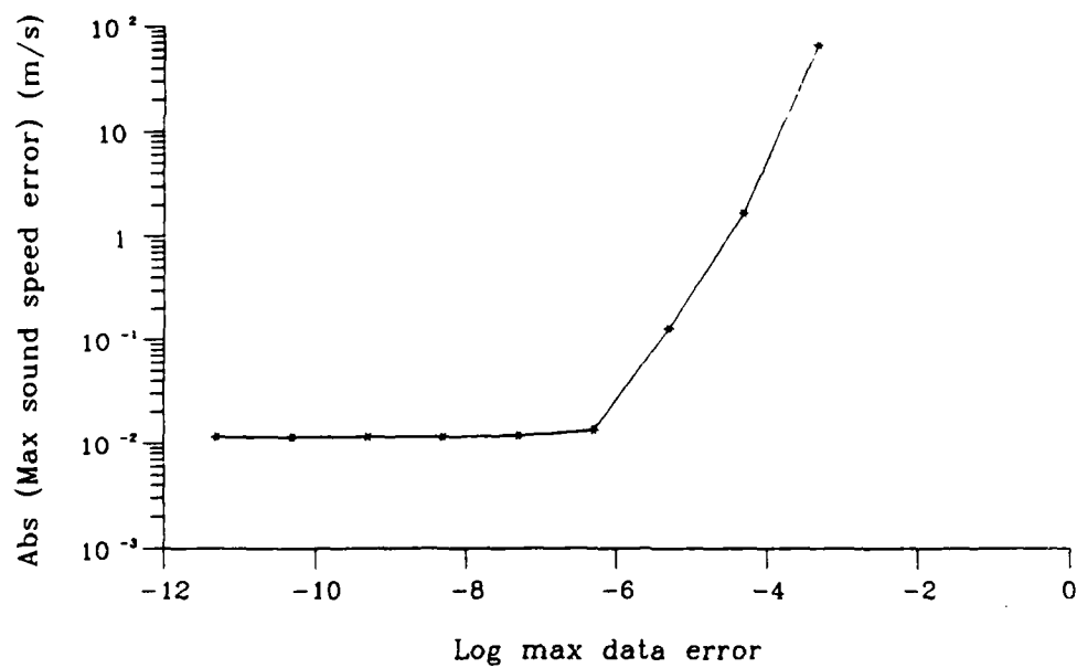
Figure 3-20: Absolute value of the maximum error for inversion method 1 using least squares basis splines with noisy data.
