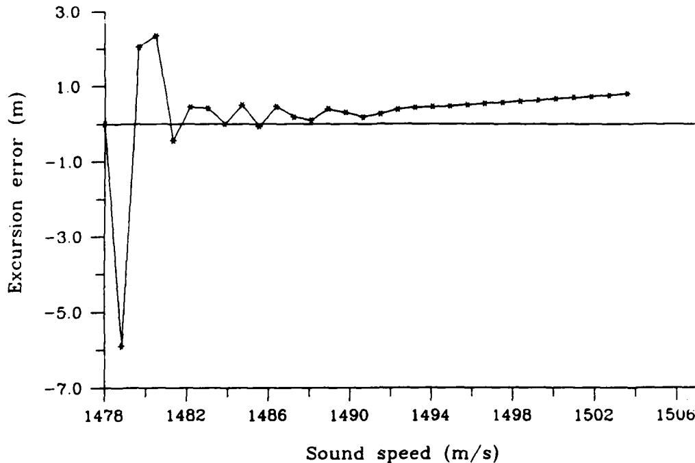
Figure 3-14: Excursion error for the bilinear profile in the region with two turning points.
