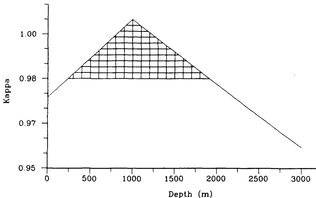
Figure 3-1: The integration over \xi' is carried out over the cross-hatched region extending from \xi to the curve \kappa(z) .
