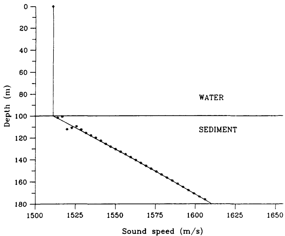
Figure 4-3: Inversion results for waveguide model 1 using inversion method 1. The background curve is the actual sound speed profile in the waveguide.
