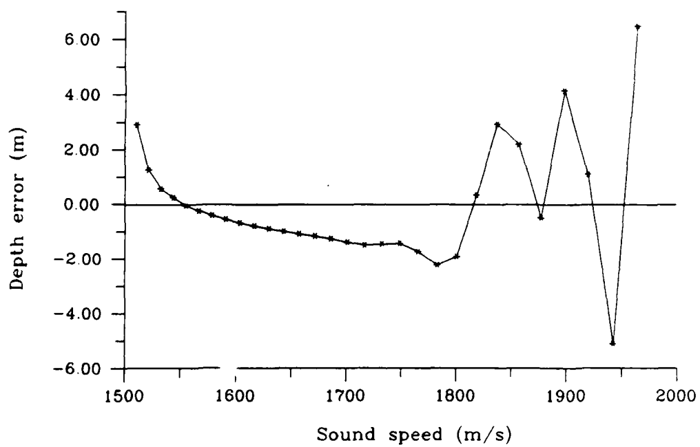
Figure 4-15: Depth error for inversion method 2 (least squares splines) applied to waveguide model 2.
