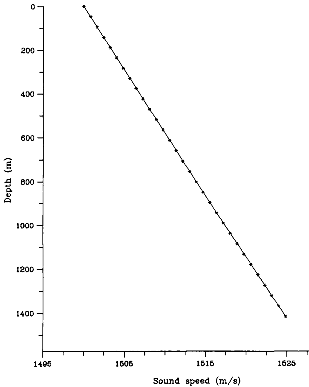
Figure 3-6: Excursion (depth) versus sound speed for the n^2(z) linear profile calculated using inversion method 2.
