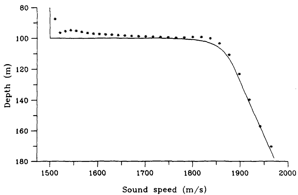
Figure 4-12: Inversion results for waveguide model 2 using inversion method 1 (smoothing splines).
