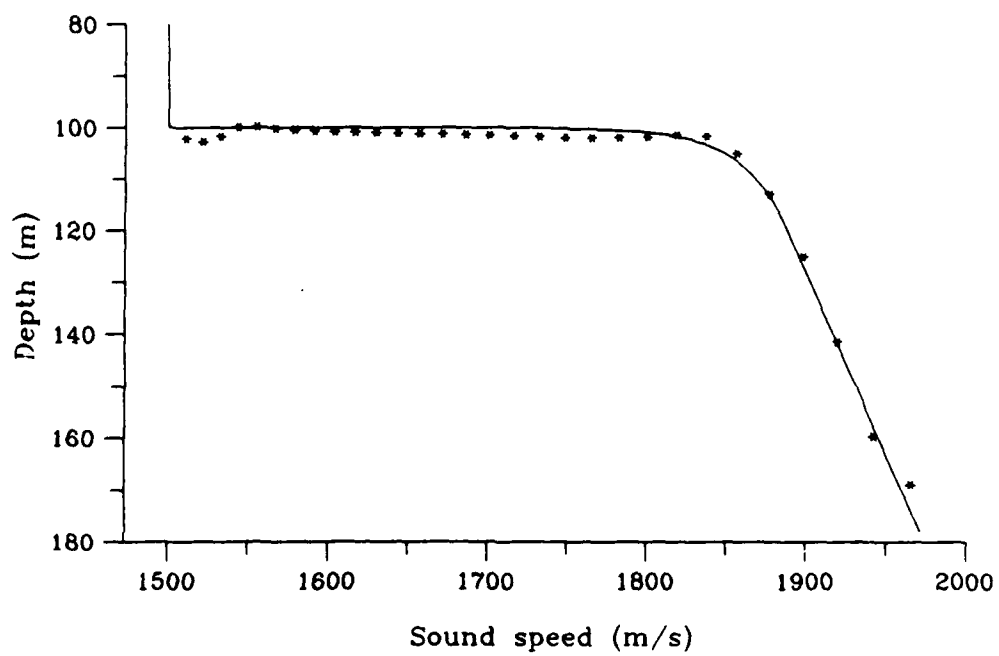
Figure 4-16: Inversion results for waveguide model 2 using inversion method 2 (smoothing splines).
