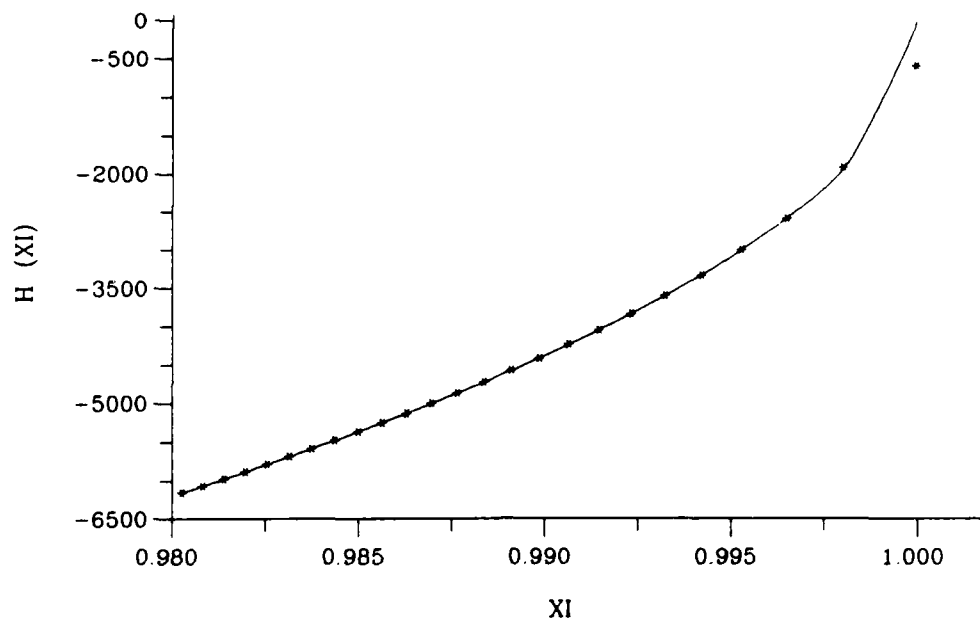
Figure 3-3: H(\xi) for the n^2(z) linear profile. The discrete points are the values of H(\xi) computed by the inversion program. The curve is the function calculated using the analytic expression.
