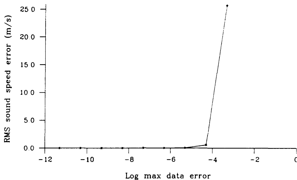
Figure 3-19: RMS error for inversion method 1 using least squares basis splines with noisy data.
