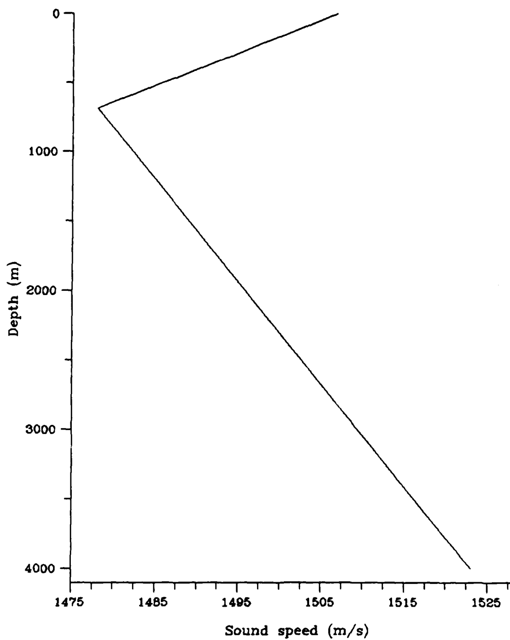
Figure 3-12: The bilinear sound speed profile model.
