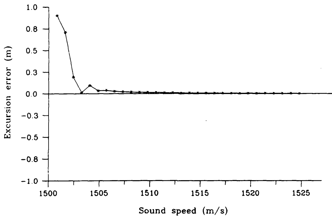
Figure 3-9: Excursion error as a function of sound speed for inversion method 1 applied to the parabolic profile. Excursion error is twice the depth error.
