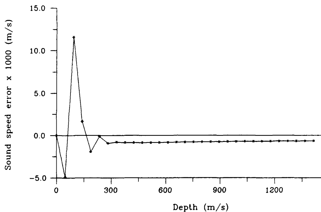
Figure 3-5: Sound speed error as a function of depth for the recovery of the n^2(z) linear profile using inversion method 1.
