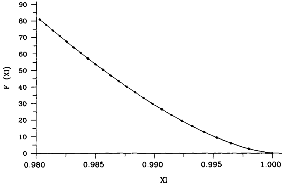
Figure 3-2: F(\xi) for the n^2(z) linear profile. The discrete points are the input data to the inversion program generated from the horizontal wavenumbers and the associated values of the WKB phase integral. The curve is F(\xi) computed using the analytic expression.
