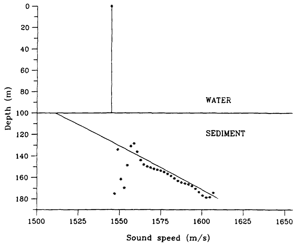
Figure 4-7: Inversion results for a terrigenous waveguide with a low velocity zone at the water/sediment interface. The eigenvalue of the lowest mode was discarded since it produced a value of \xi > 1 .
