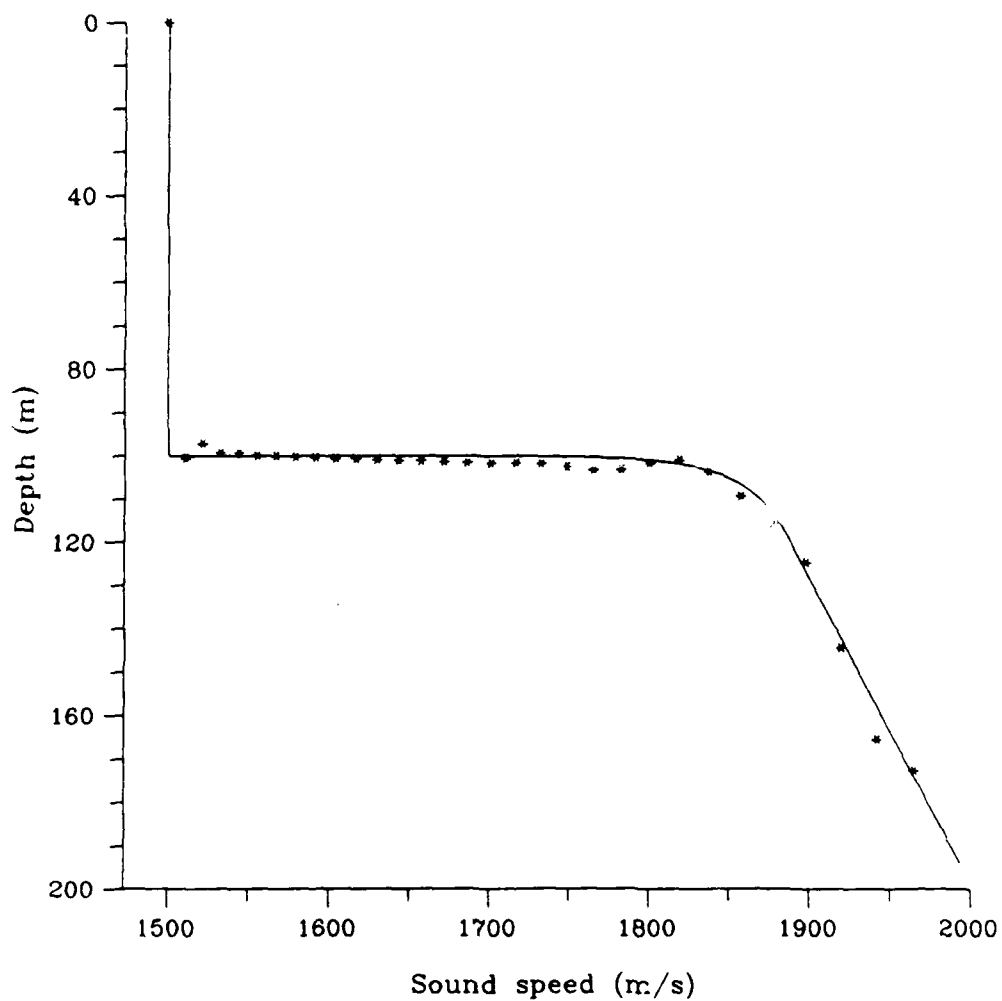
Figure 4-10: Inversion results for waveguide model 2 using inversion method 1 (least squares splines).
