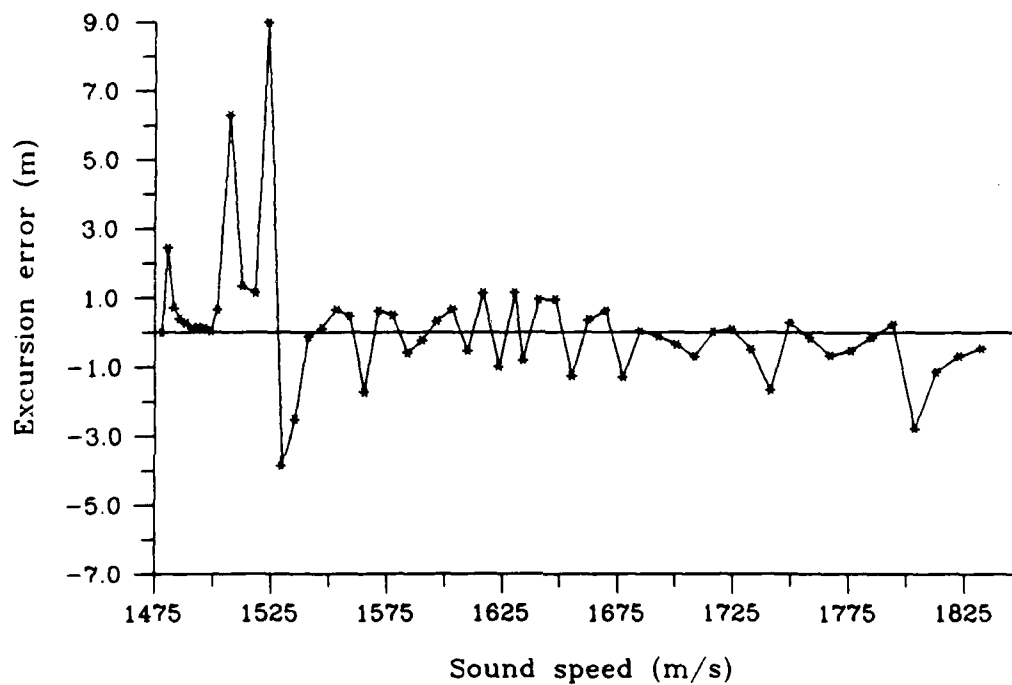
Figure 3-17: Excursion error as a function of sound speed for the bilinear profile. For sound speeds greater than 1507 m/s this is depth error.
