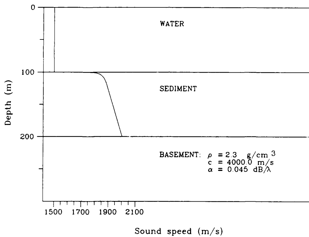
Figure 4-9: The shallow water waveguide model with a fine sand bottom.
