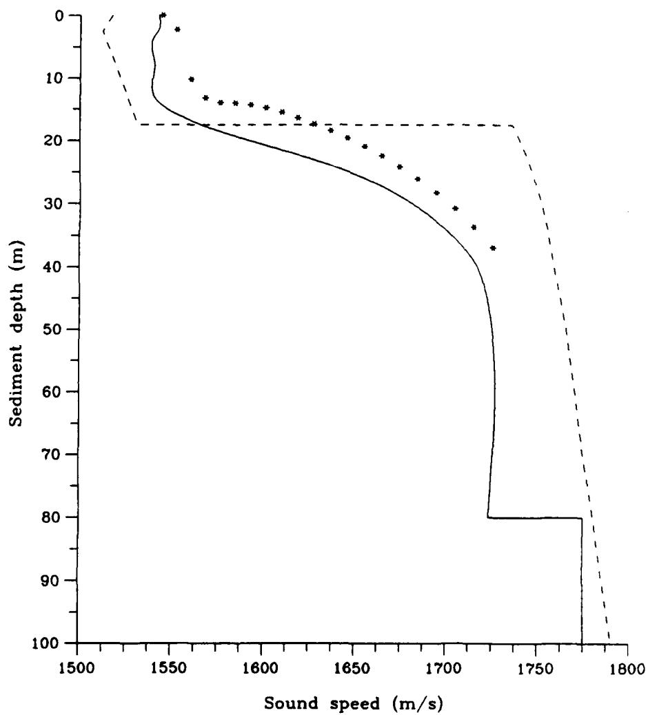
Figure 4-22: Corpus Christi sediment sound speed profile obtained with inversion method 1 after removing the second 50 Hz eigenvalue, the profile obtained perturbatively by Rajan (solid curve), and predicted profile (dotted curve).
