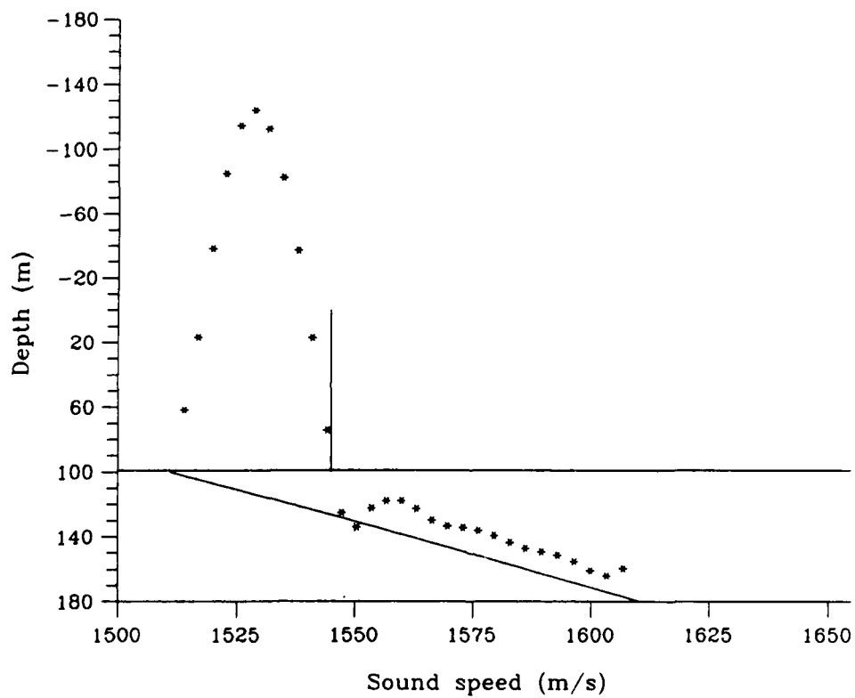
Figure 4-8: Inversion results for a terrigenous waveguide with a low velocity zone at the water/sediment interface obtained using the correct reference sound speed of 1511 meters per second.
