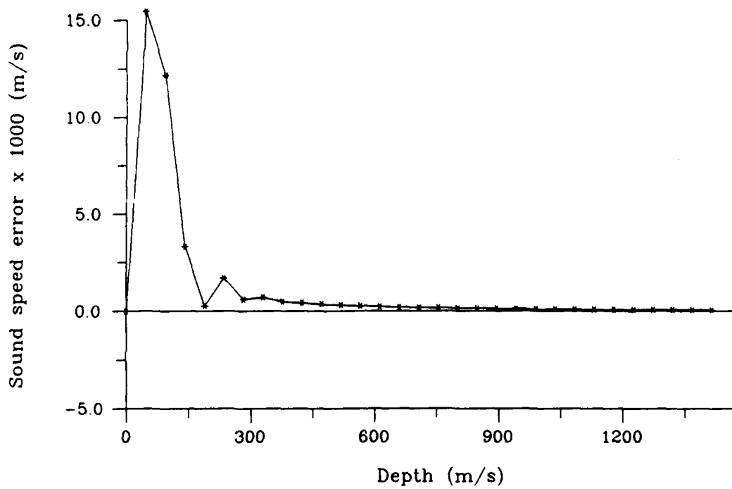
Figure 3-7: Sound speed error versus depth for inversion method 2 applied to the n^2(z) linear profile.
