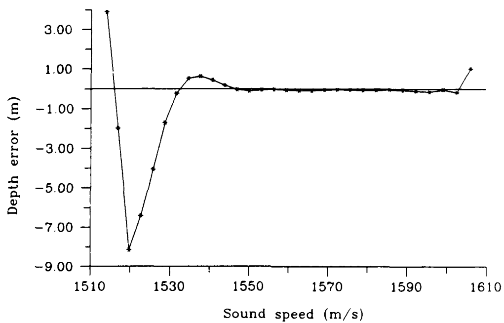
Figure 4-6: Depth error for inversion method 2 applied to waveguide model 1.
