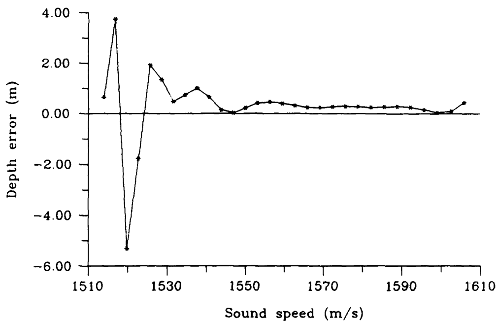
Figure 4-4: Depth error for inversion method 1 applied to waveguide model 1.
