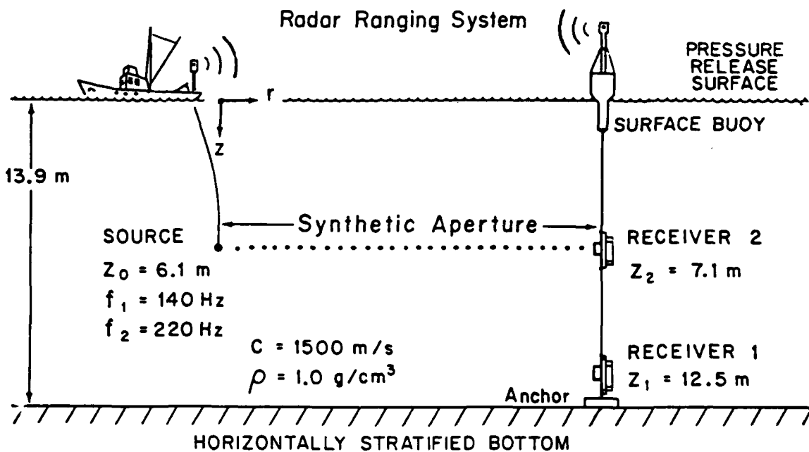
Figure 4-1: Experimental configuration for measuring the eigenvalues in a shallow water waveguide. The parameters shown are for an experiment in Nantucket Sound, Massachusetts [21]
