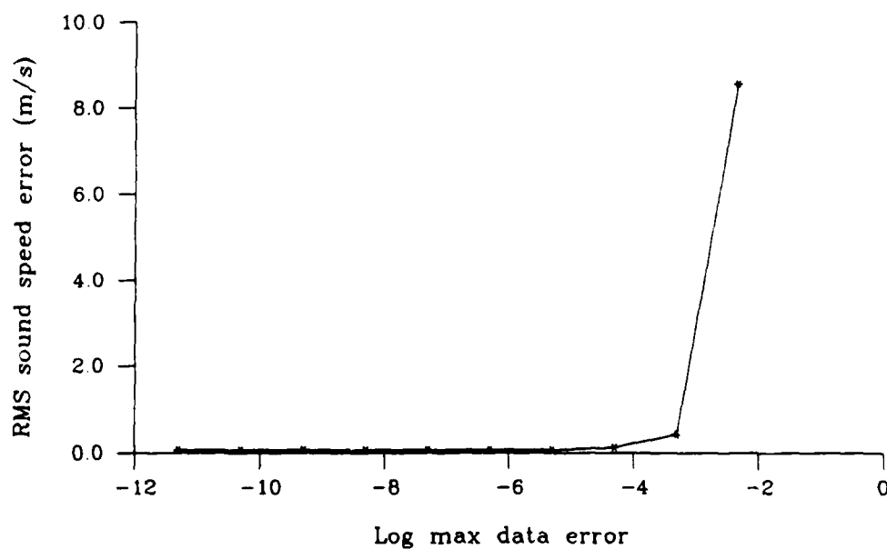
Figure 3-25: RMS error for inversion method 2 using smoothing splines with noisy data.
