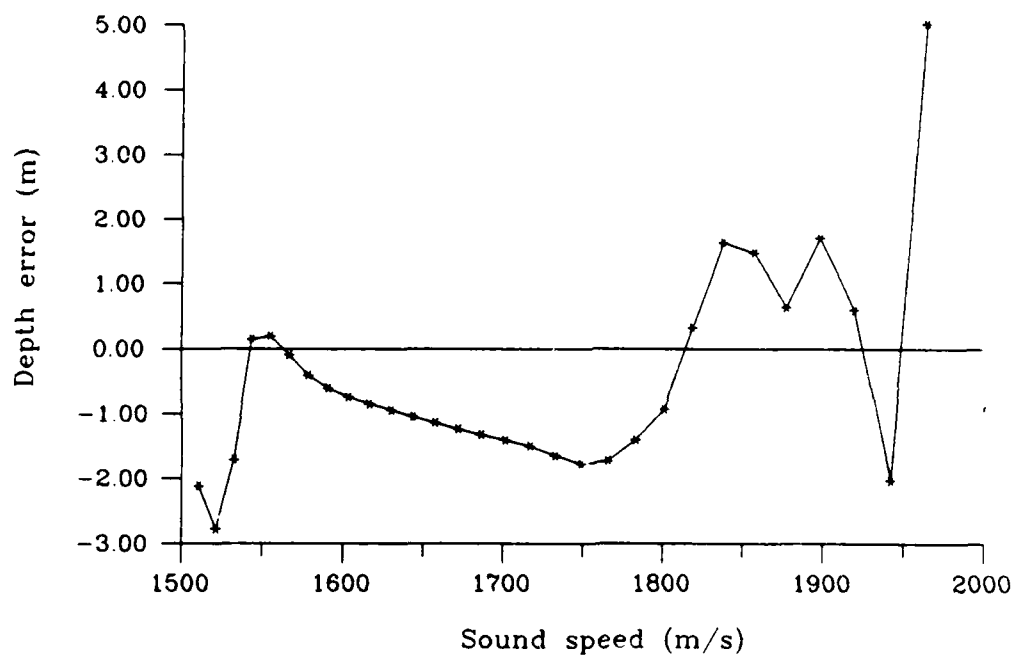
Figure 4-17: Depth error for inversion method 2 (smoothing splines) applied to waveguide model 2.
