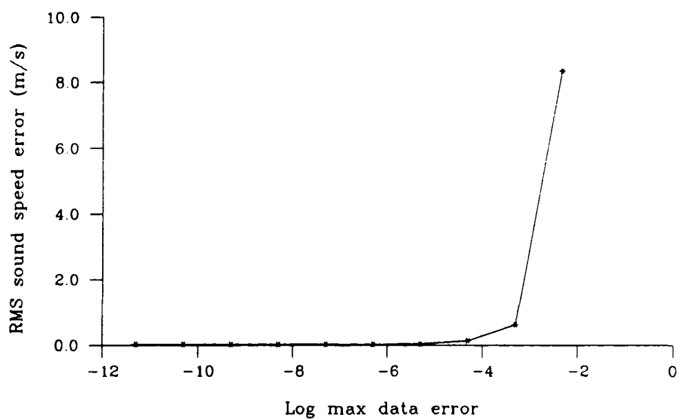
Figure 3-23: RMS error for inversion method 1 using smoothing splines with noisy data.
