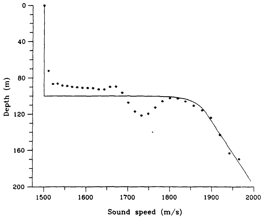
Figure 4-18: Inversion results for waveguide model 2 using inversion method 1 (least squares splines) treating the low order modes as reflecting from a half-space with a 1727 meter per second sound speed.
