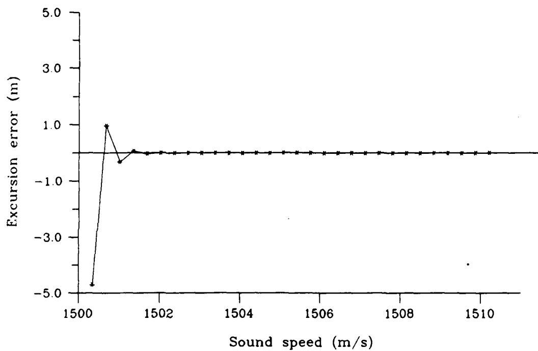
Figure 3-11: Excursion error versus sound speed for inversion method 2 applied to the parabolic profile.
