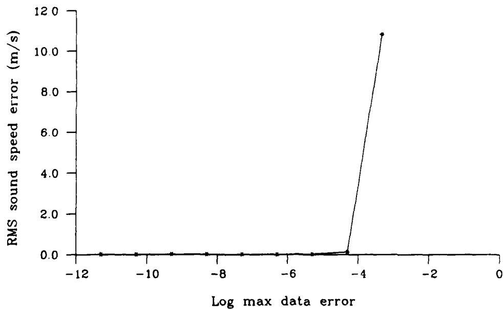
Figure 3-21: RMS error for inversion method 2 using least squares basis splines with noisy data.
