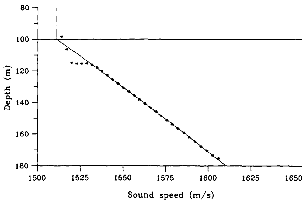
Figure 4-5: Inversion results for waveguide model 1 using inversion method 2. The background curve is the actual sound speed profile in the waveguide.
