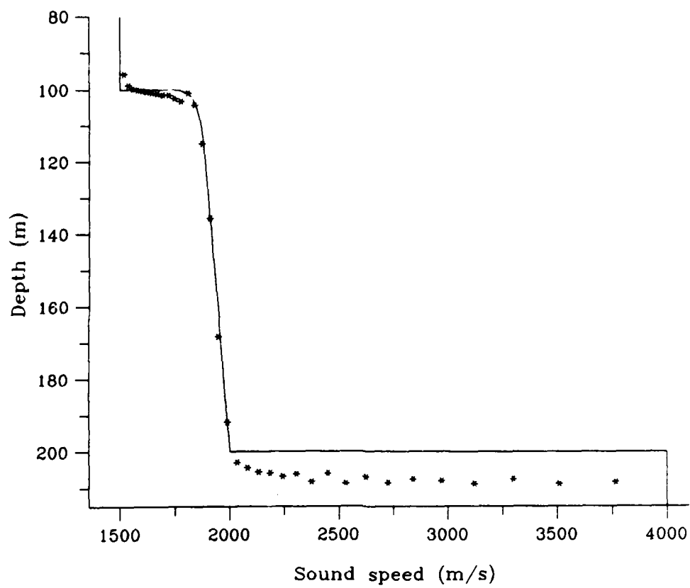
Figure 4-19: Inversion results for waveguide model 2 using inversion method 1 (least squares splines) using the eigenvalues of all propagating modes.
