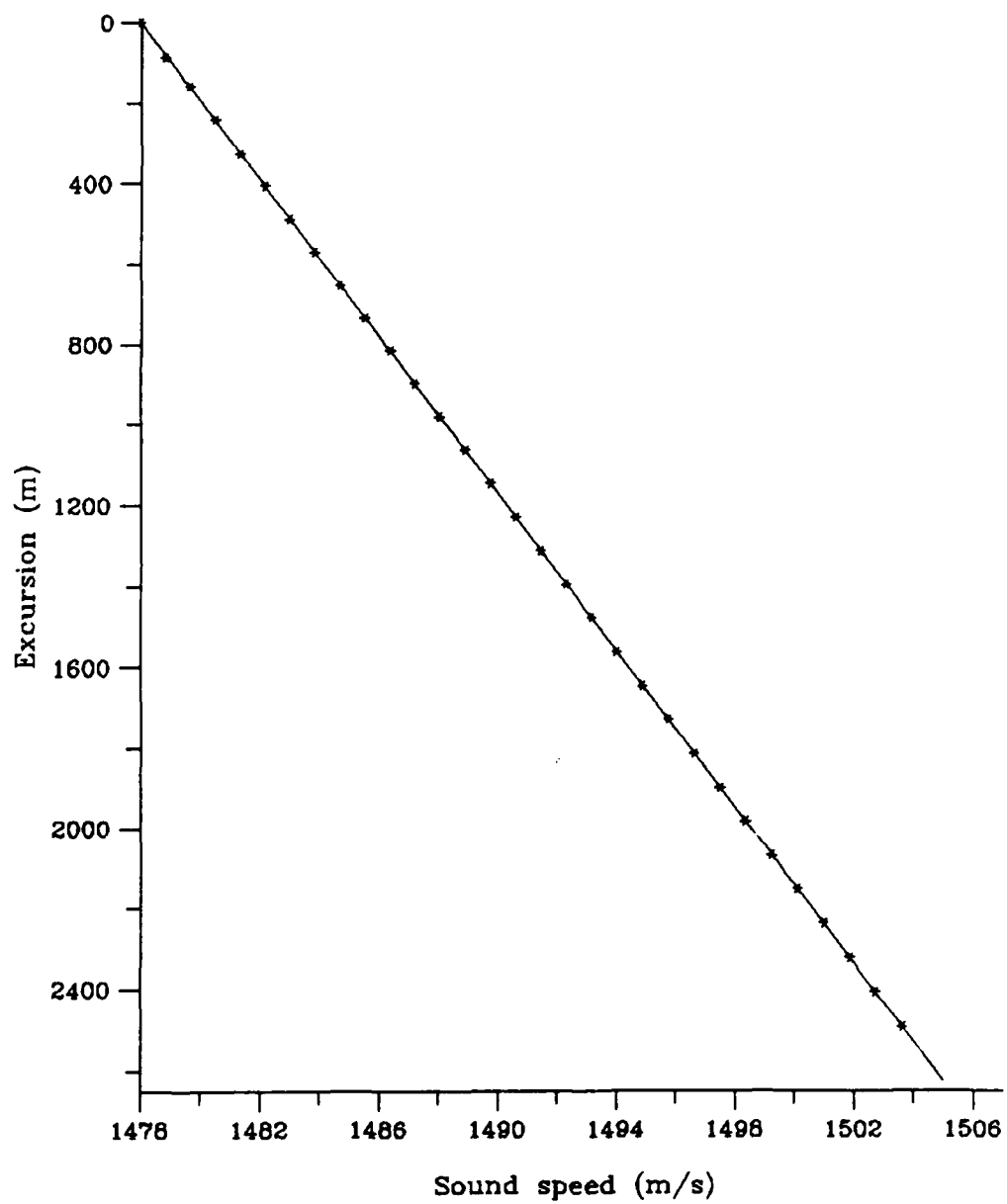
Figure 3-13: The excursion for the bilinear profile using eigenvalues for modes with an upper turning point deeper than 100 meters.
