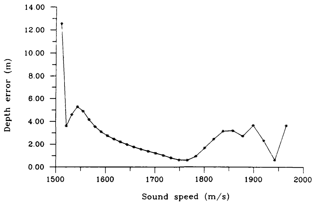
Figure 4-13: Depth error for inversion method 1 (smoothing splines) applied to waveguide model 2.
