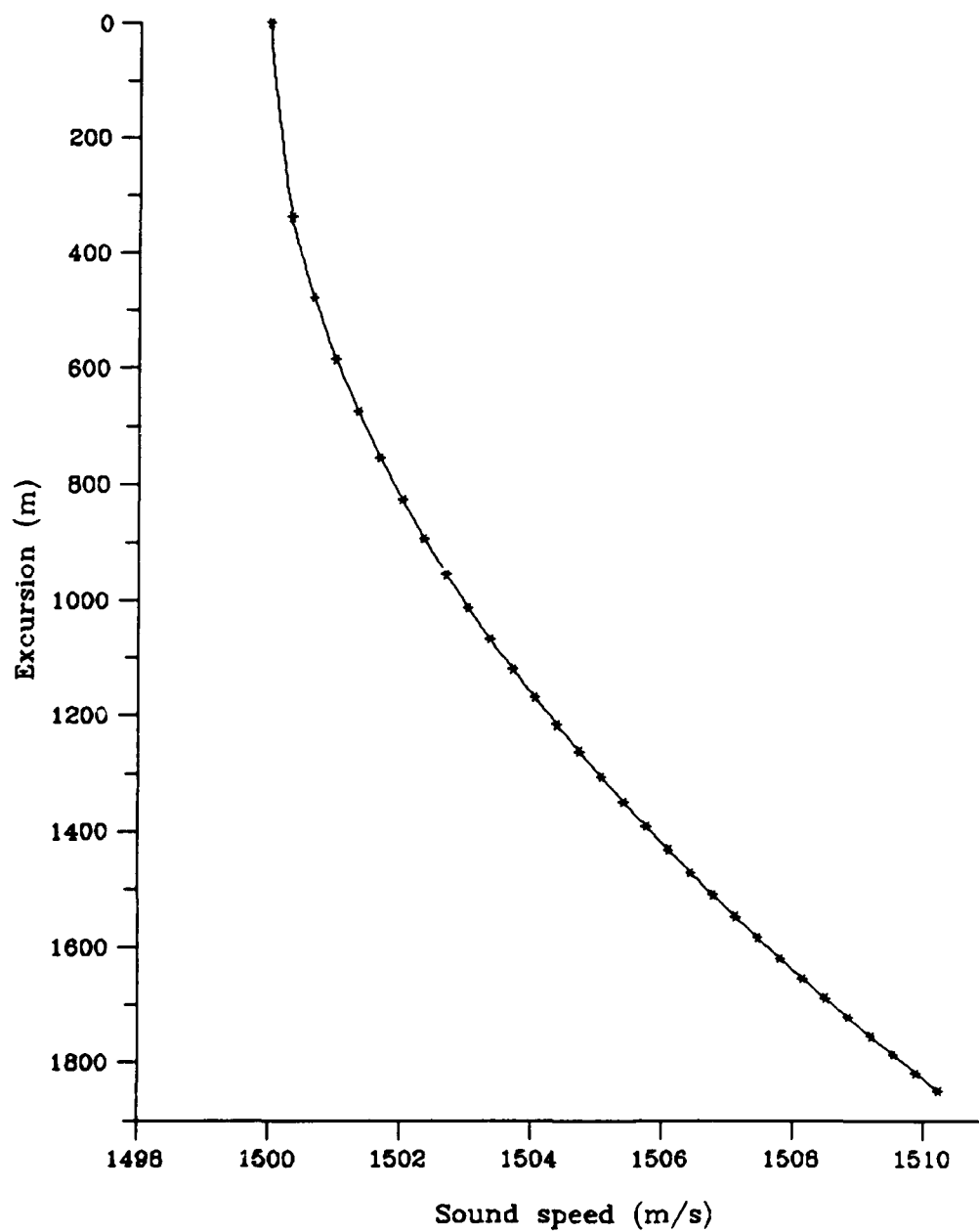
Figure 3-10: The excursion for the parabolic profile computed using inversion method 2. The excursion is the distance between points of equal sound speed on the two branches of the sound speed profile.
