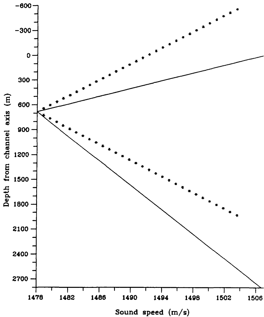
Figure 3-18: Sound speed versus depth for the symmetric profile equivalent to the bilinear profile.
