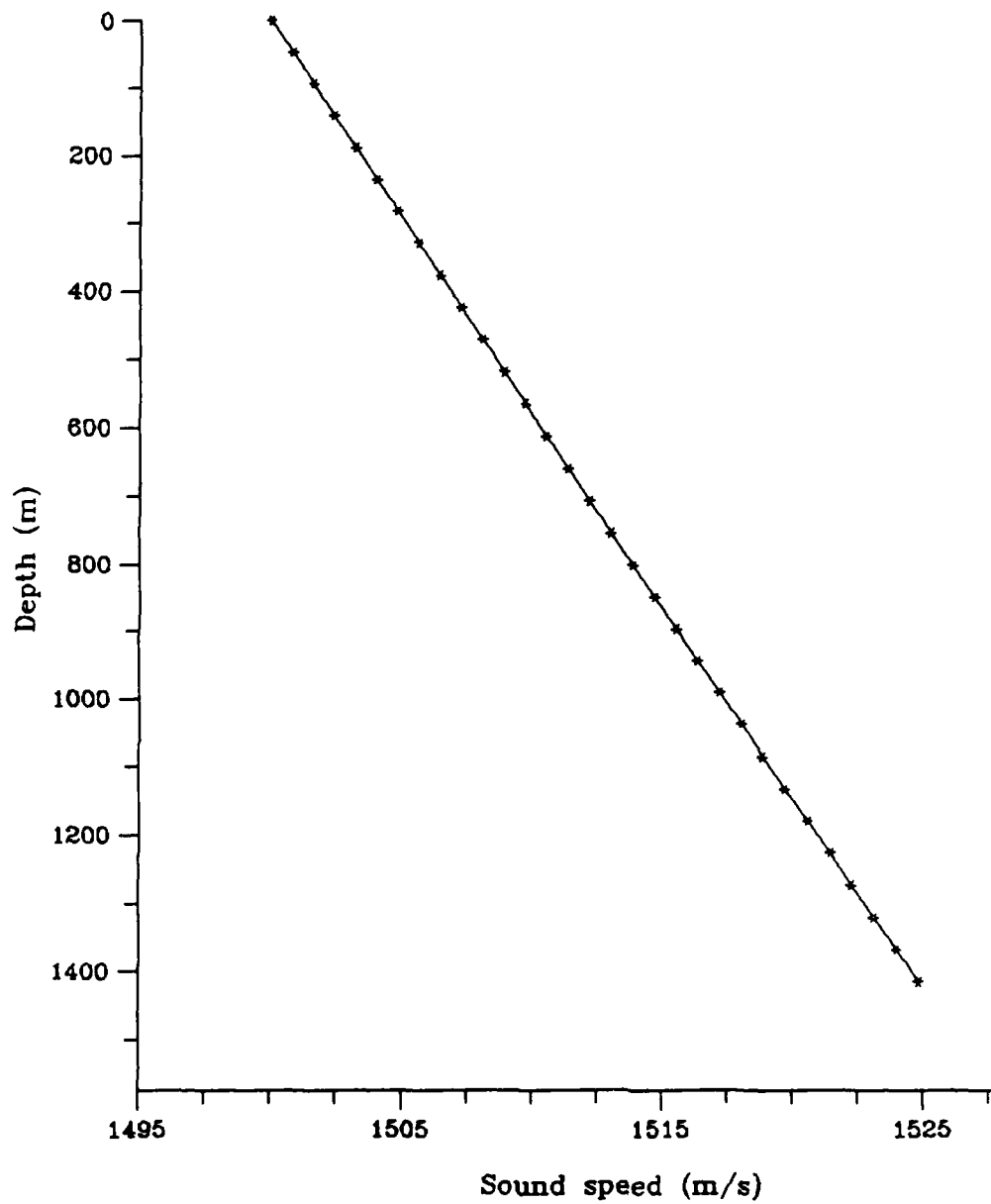
Figure 3-4: The sound speed profile for the n^2(z) profile recovered using inversion method 1. The discrete points are the output values from the inversion.
