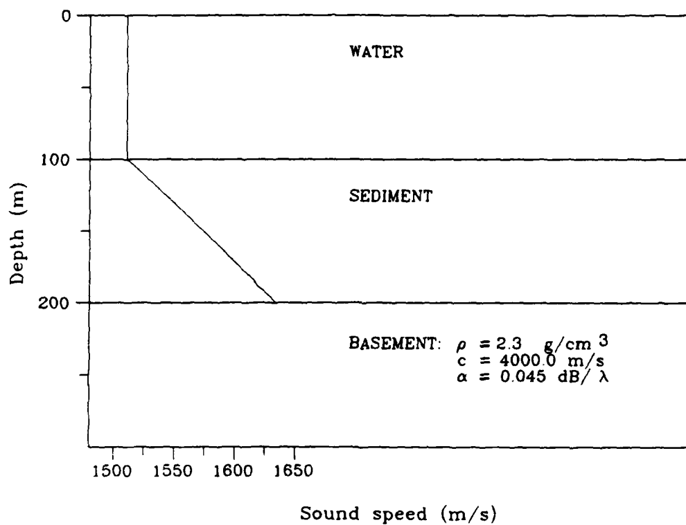
Figure 4-2: The shallow water waveguide model with a terrigenous sediment bottom.
