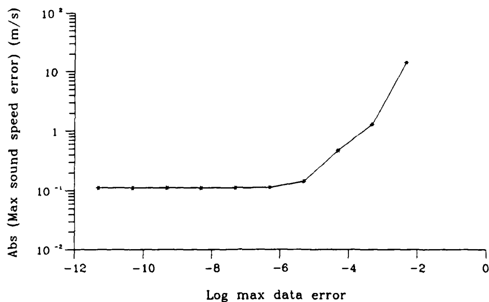
Figure 3-24: Absolute value of the maximum error for inversion method 1 using smoothing splines with noisy data.
