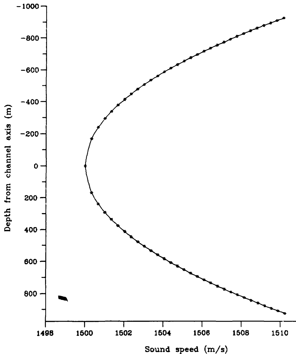
Figure 3-8: Depth versus sound speed for the parabolic profile recovered using inversion method 1. The points below the channel axis are the actual inversion results, and the profile symmetry was used to generate the profile above the axis.
