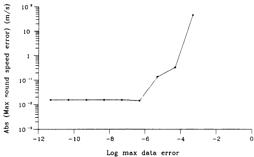
Figure 3-22: Absolute value of the maximum error for inversion method 2 using least squares basis splines with noisy data.
