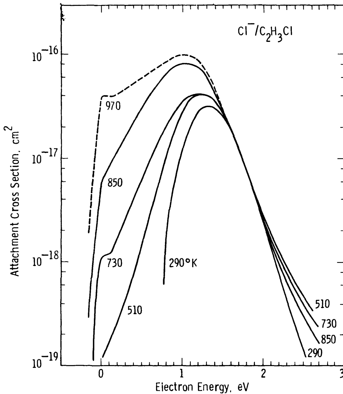
Figure 9 — The cross section for \text{Cl}^- production from \text{C}_2\text{H}_3\text{Cl} measured at the temperature indicated, using the "High-Temperature Collision Chamber." The highest temperature curve (970°K) is uncertain due to thermal dissociation effects.
