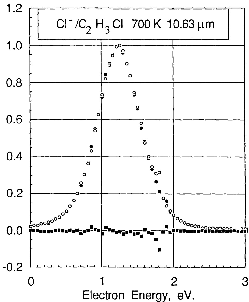
Figure 4.8 — Cl - production from C 2 H 3 Cl measured with (•) and without (o) the laser beam (10.63 μm) at 700 K. The difference signal is shown by the filled squares.
