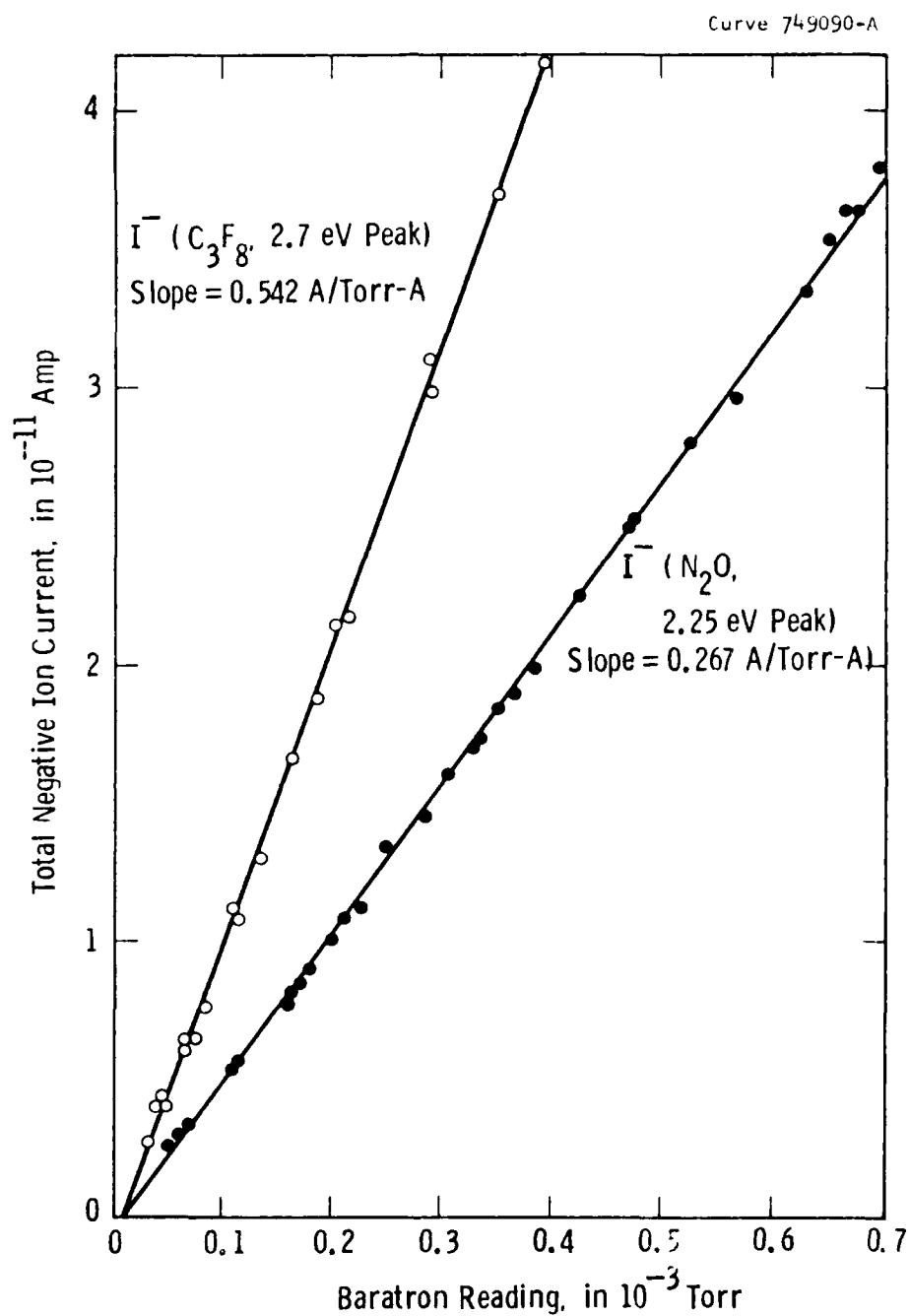
Figure 2 — An example of the total negative ion currents measured as a function of the collision chamber pressure in N_2O and C_3F_8 . In each case the electron beam energy is adjusted to the peak in the cross section. The ratio of the slopes gives the ratio of the peak cross sections.
