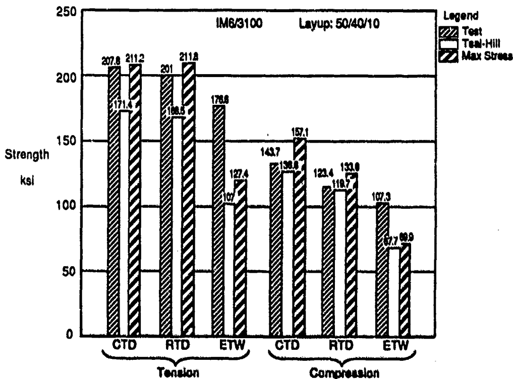
Figure 87. Prediction of IM6/3100 50/40/10 Laminate Strengths
