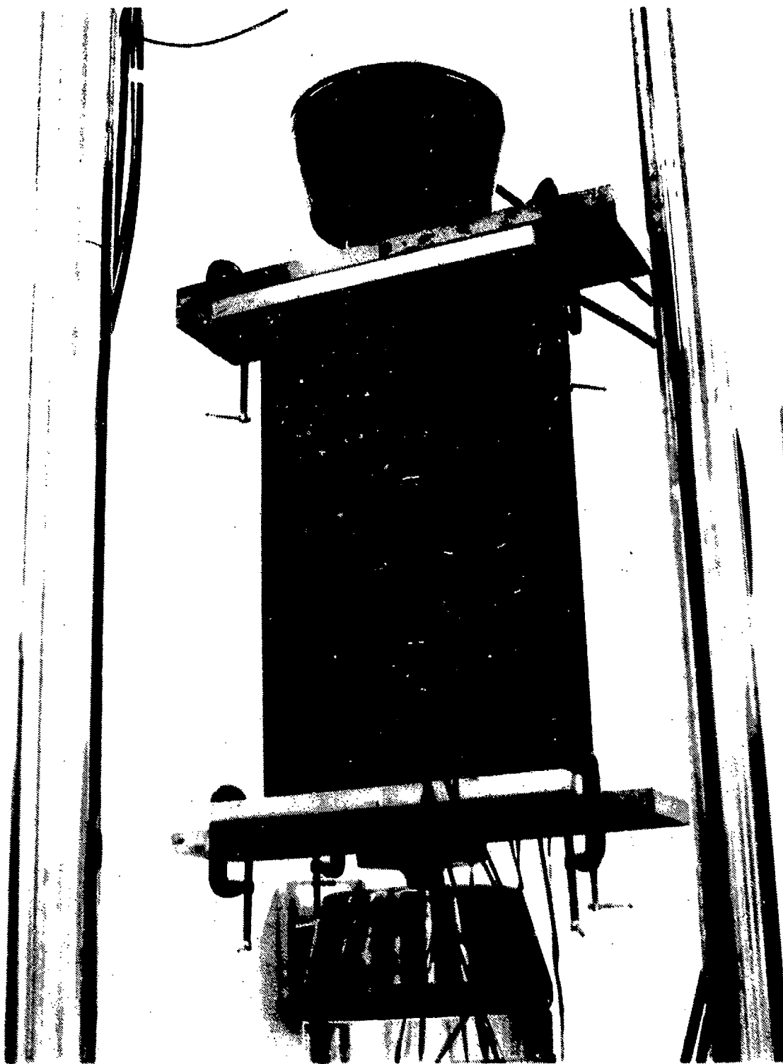
Figure 143. Panel Test Setup
