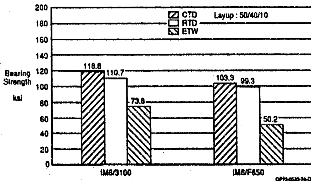
Figure 116. Loaded Hole (Bearing) Strength Test Results
