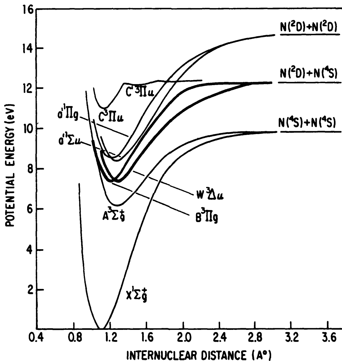
Figure 1. Potential energy curves of selected states of N_2 .
