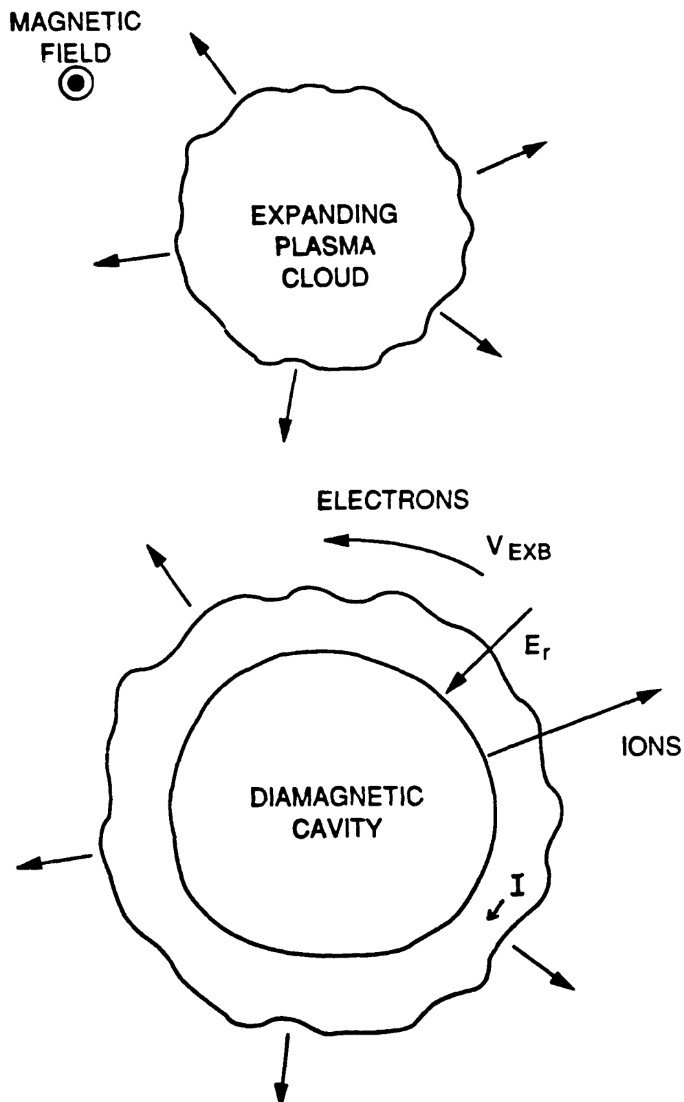
Figure 1. Schematic of the structuring mechanism showing the outward motion of the ions, the radial electric field, the electron \vec{E} \times \vec{B} drift, the resulting current (I), and the diamagnetic cavity.
