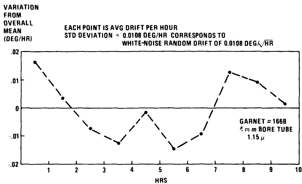
Figure 3-8. One-Hour Drift Analysis of Figure 3-7 Data
