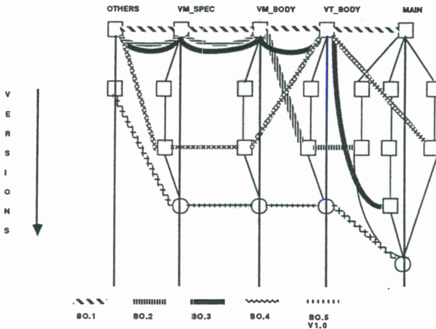
Figure A-2: Configuration Model Resulting from Performing Steps in Experiment #1
