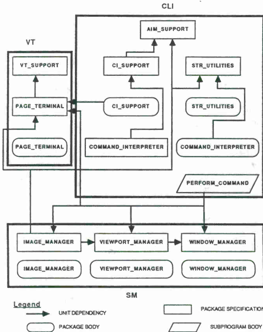
Figure A-1: Evaluation System Model
