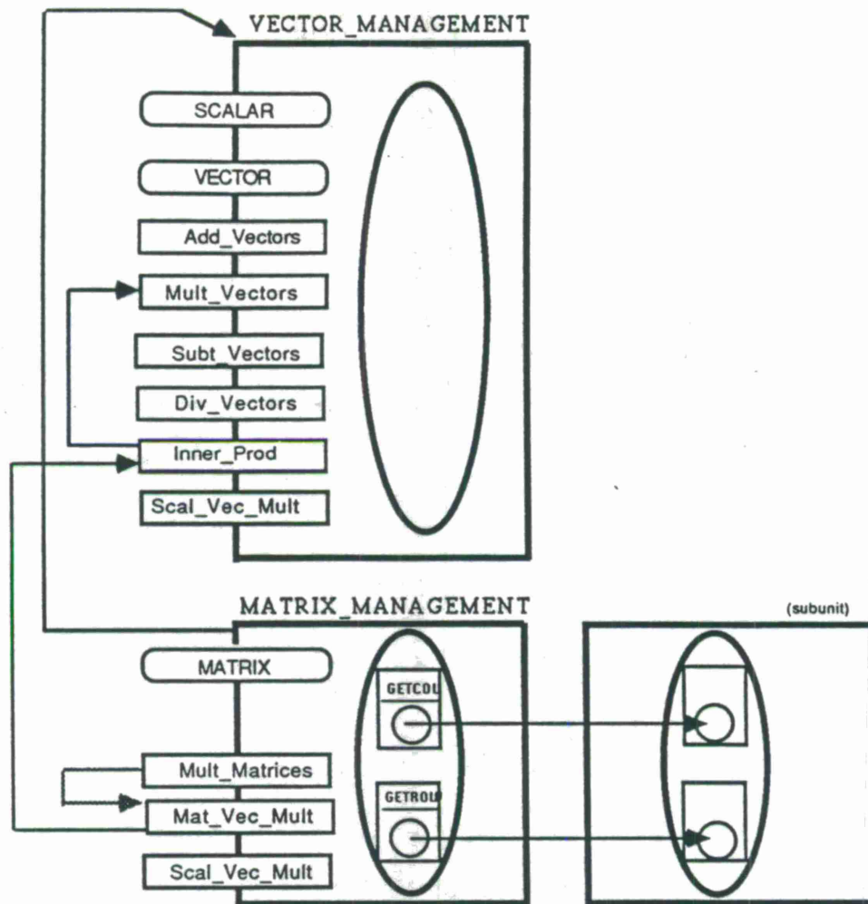
Figure A-12: Subprogram Interdependencies
