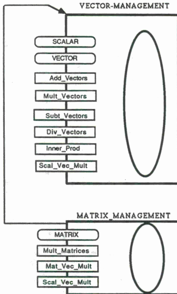
Figure A-9: Preliminary Package Design
