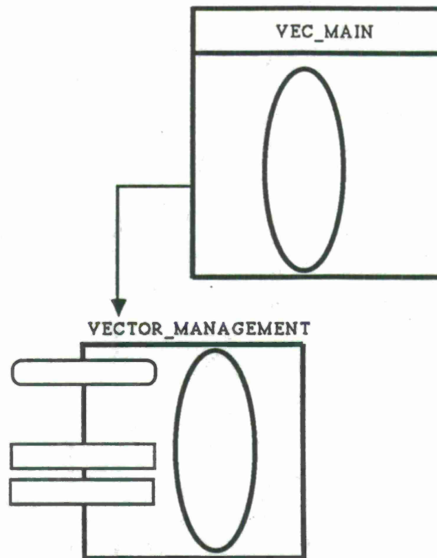
Figure A-13: Vector Multiplication Test Harness
