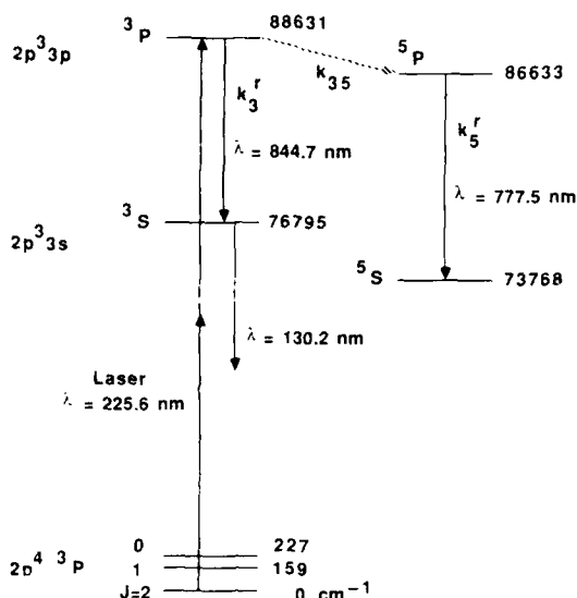
Fig. 1. Relevant energy levels for two-photon excitation of oxygen atoms and excited-state collisional energy transfer. The electronic energies, taken from ref. [16], are given in \text{cm}^{-1} , and allowed radiative transitions are denoted, with wavelengths given in nm. The denoted radiative and collisional rate constants are defined in section 3.2.
