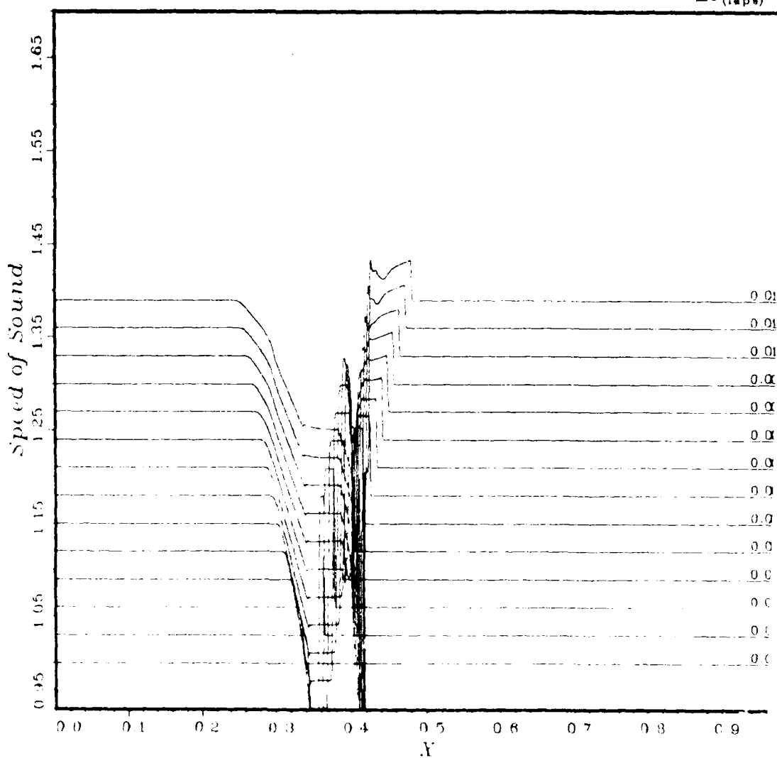
Figure 61. Detail study, magnified sound speed versus distance, part 1
