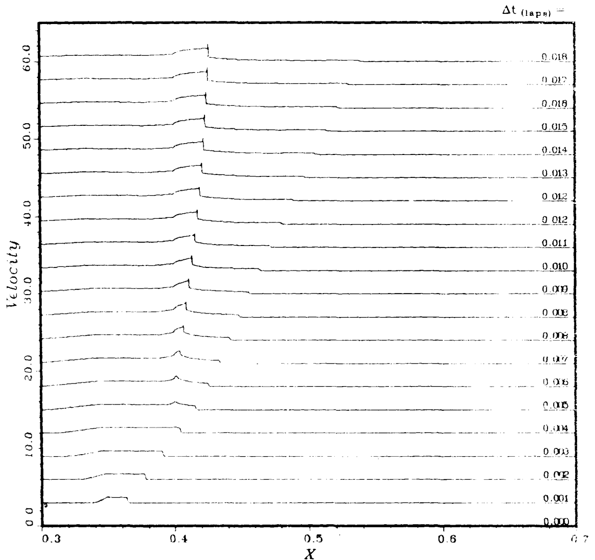
Figure 72. Detail study, velocity versus distance 0.3 to 0.7, part 1
