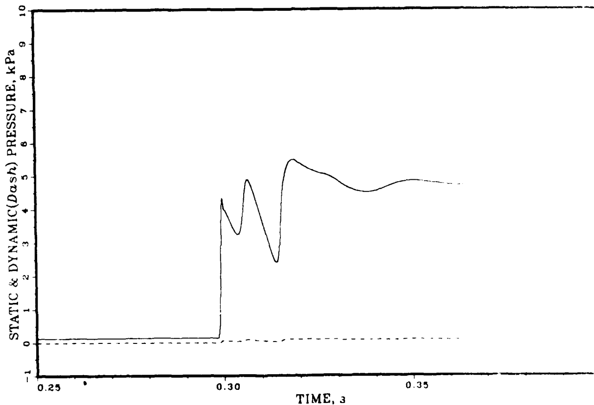
Figure 99. Pressure versus time, case 9, 20ms opening time
