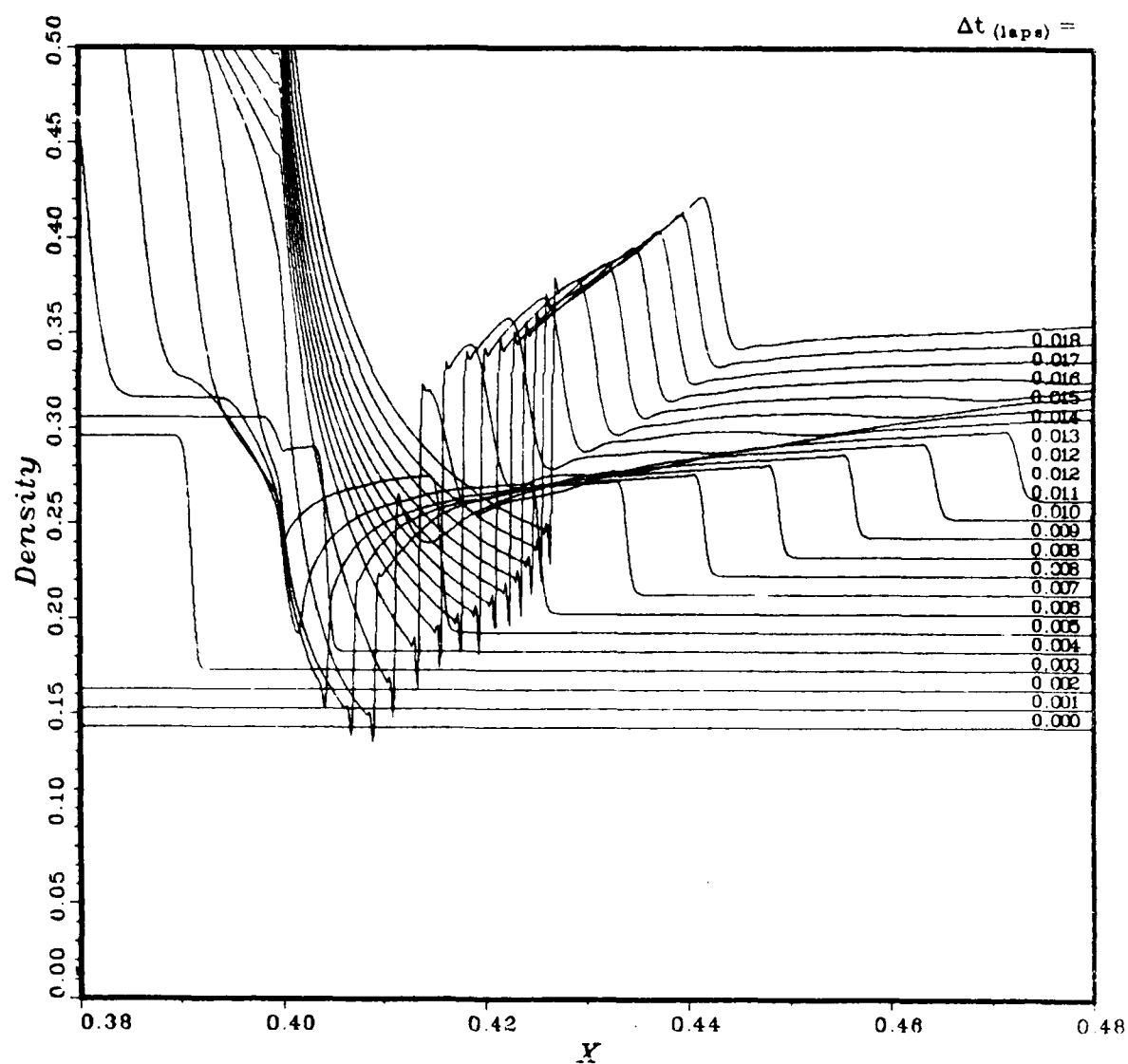
Figure 81. Detail study, density versus distance 0.38 to 0.48
