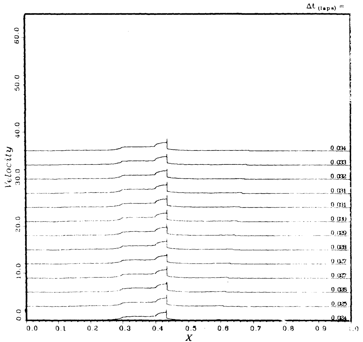
Figure 54. Detail study, velocity versus distance, part 3
