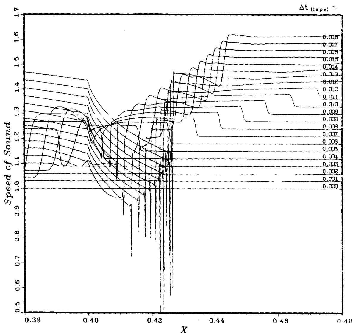
Figure 83. Detail study, sound speed versus distance 0.38 to 0.48
