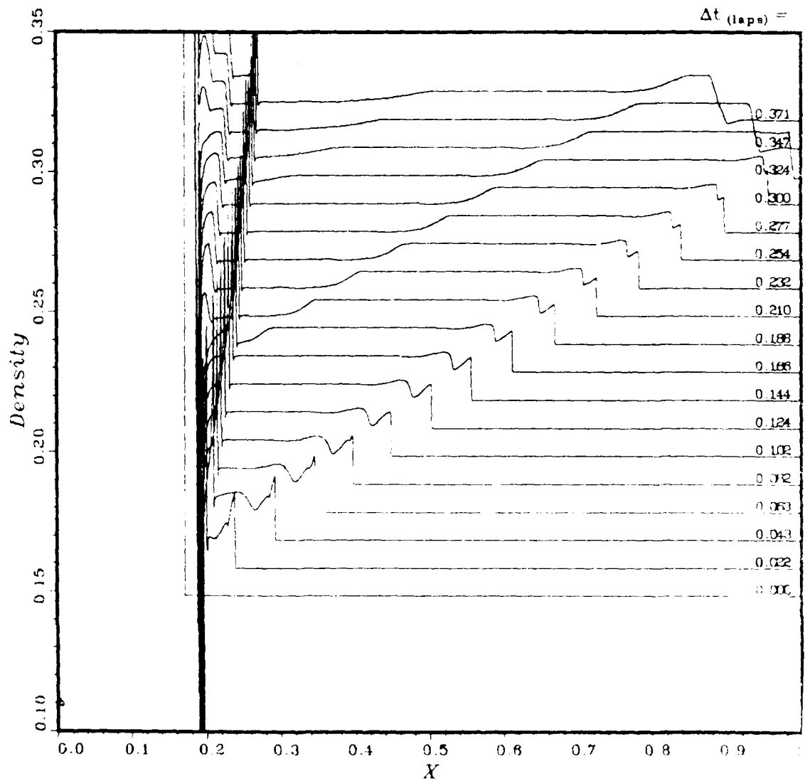
Figure 33. Magnified density versus distance, case 8, zero opening time
