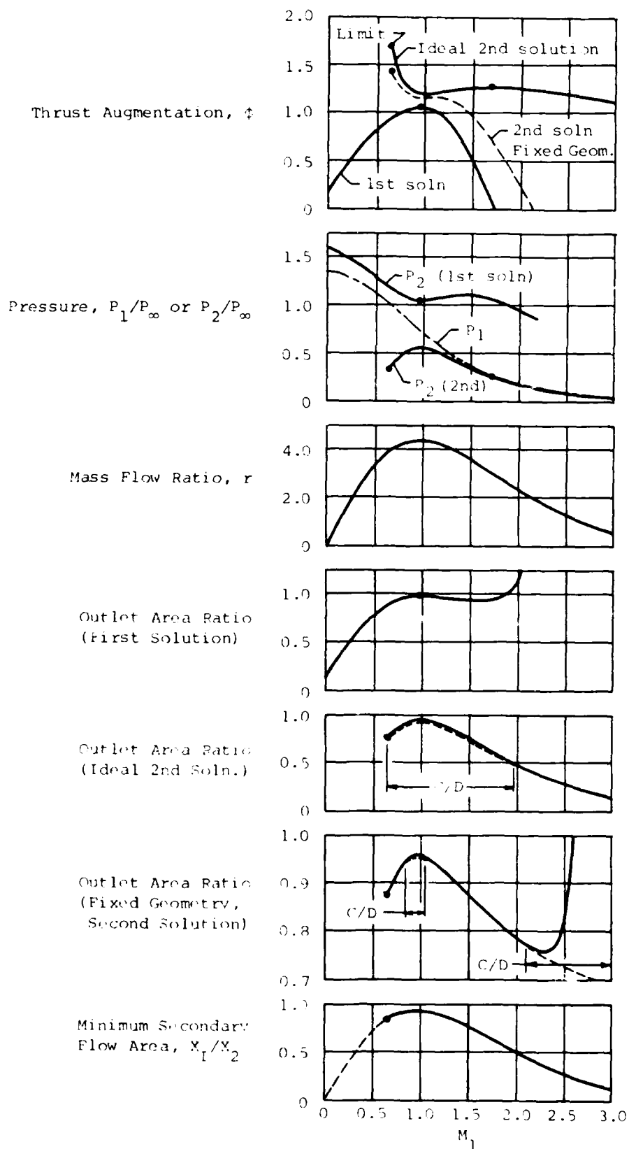
Figure 2. Elector characteristics with cold primary flow, M_\infty = 0.65 , \alpha_\star = 22.65 , T_{op}/T_\infty = 1 , P_{op}/P_\infty = 6.1
