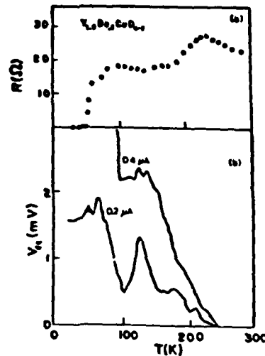
FIG. 1 (a) The resistance vs temperature of the Y-Ba-Cu-O sample used in the reverse ac Josephson experiment. (b) The dc voltages induced by rf currents of two different amplitudes. f = 5 MHz.
