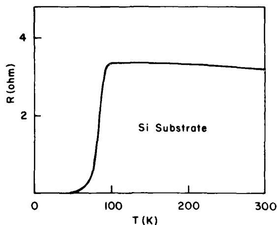
FIG. 1. Temperature dependence of the resistance of a 2-μm-thick YBaCuO film deposited on a (100)Si wafer after rapid thermal annealing in oxygen at 920 °C for 8 s; T_c(0) = 46 K.
