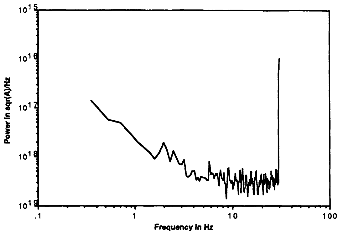
Figure 4.12 Instrumentation noise of potentiostat with OP-27 operational amplifiers. Noise power has been measured with a 466Ω load. The large spike at 30 Hz is due to aliasing of 60 Hz power-line pickup.
