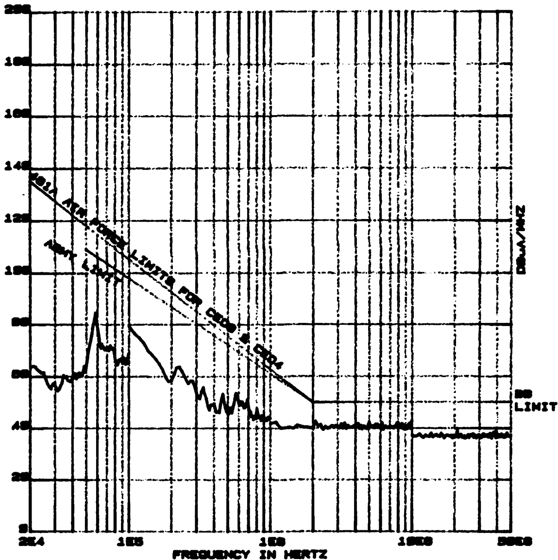
Figure 38. CE03 measured emissions - line #5 28 volt return - BB active.
