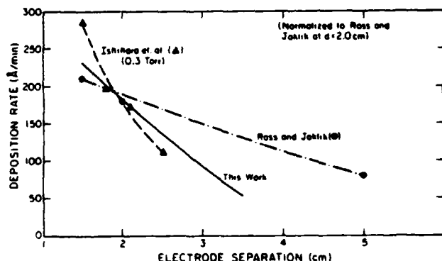
FIG. 12. Computed deposition rate of a\text{-Si:H} as a function of electrode separation compared to the results of Ross and Jaklik (Ref. 3) and Ishihara et al. (Ref. 6) for similar conditions. The results have been normalized to Ross and Jaklik at d = 2 \text{ cm} .
