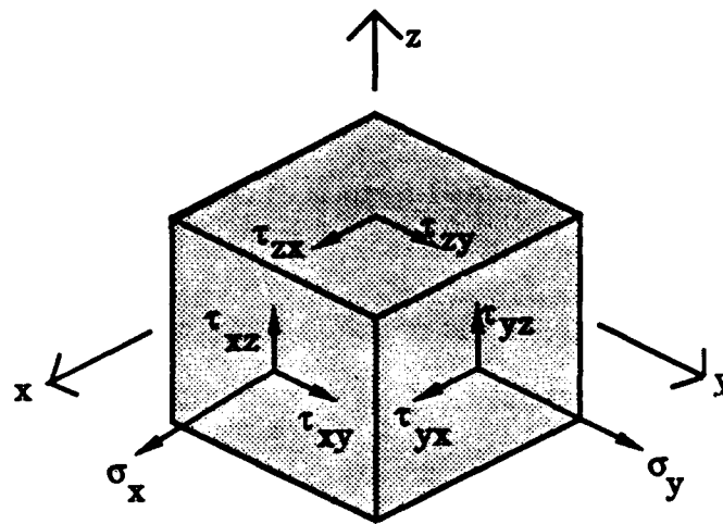
Figure 5. Stresses in a Cube of Material.
