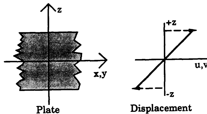
Figure 8. Variations in x and y displacements as a function of z for the Mindlin Plate Theory.
