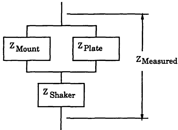
Figure 35. Impedance Measurement Model.
