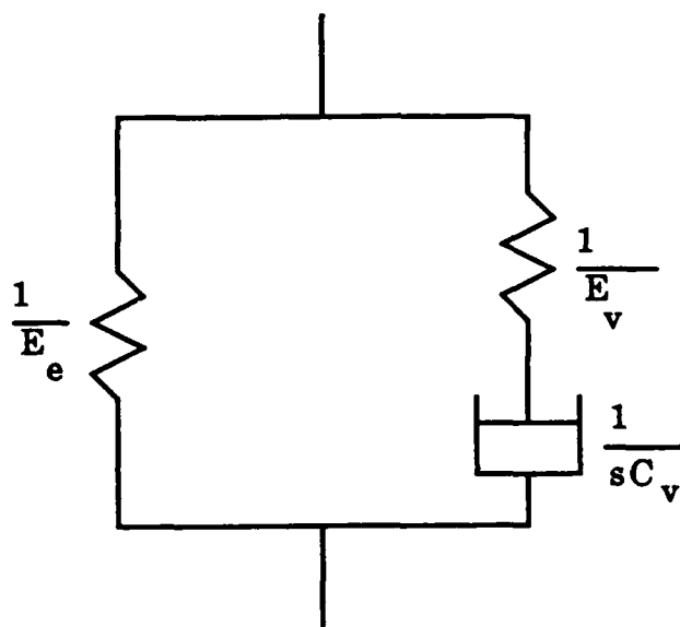
Figure 6. Laplace Transform of Viscoelastic Material Model
