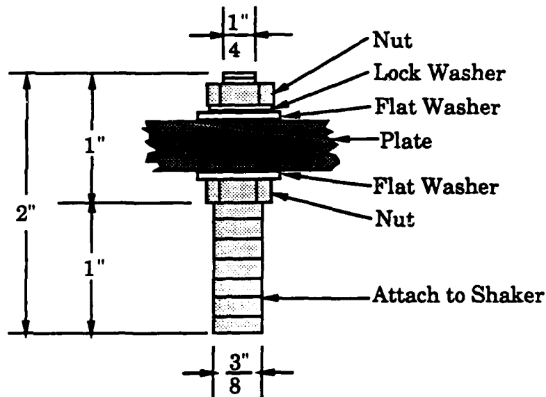
Figure 32. Steel Plate to Shaker Mount.
