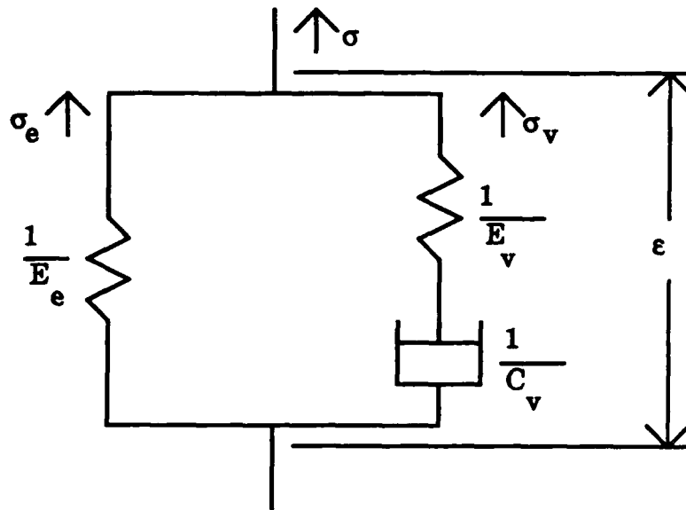
Figure 3. Viscoelastic Material Model.
