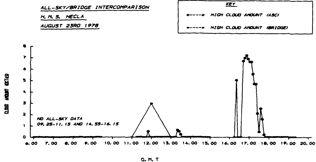
Figure 40 All-sky/bridge high cloud intercomparison for August 23rd 1978
