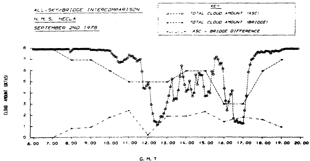
Figure 36 All-sky/bridge total cloud intercomparison for September 2nd 1978
