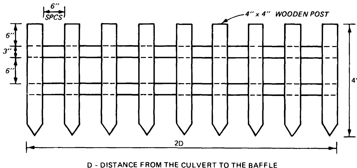
Figure 18. Slotted baffles
