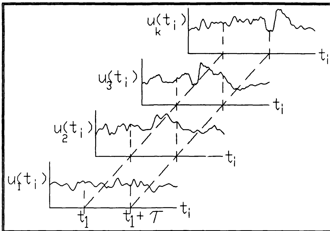
Figure III-1. AN ENSEMBLE OF TIME HISTORY RECORDS [BENDAT AND PERSOL, REF. 6].
