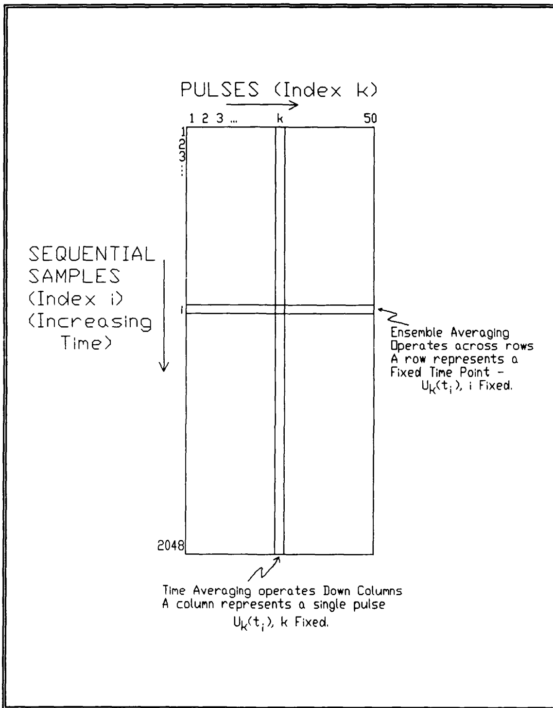
Figure IV-4. FORMAT OF ARRAY ENSEMBLE.
