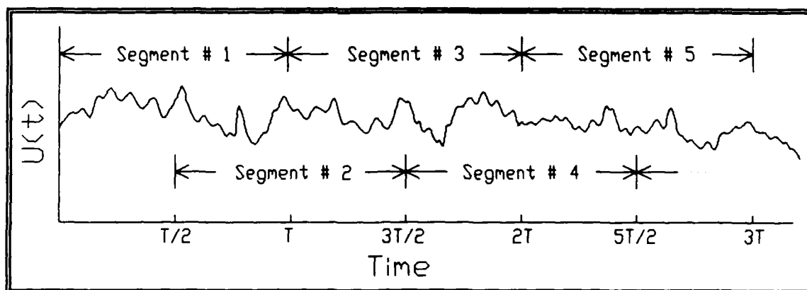
Figure IV-21. SEQUENCE OF OVERLAPPED SEGMENTS OF LENGTH WITH 50% OVERLAPPING.
