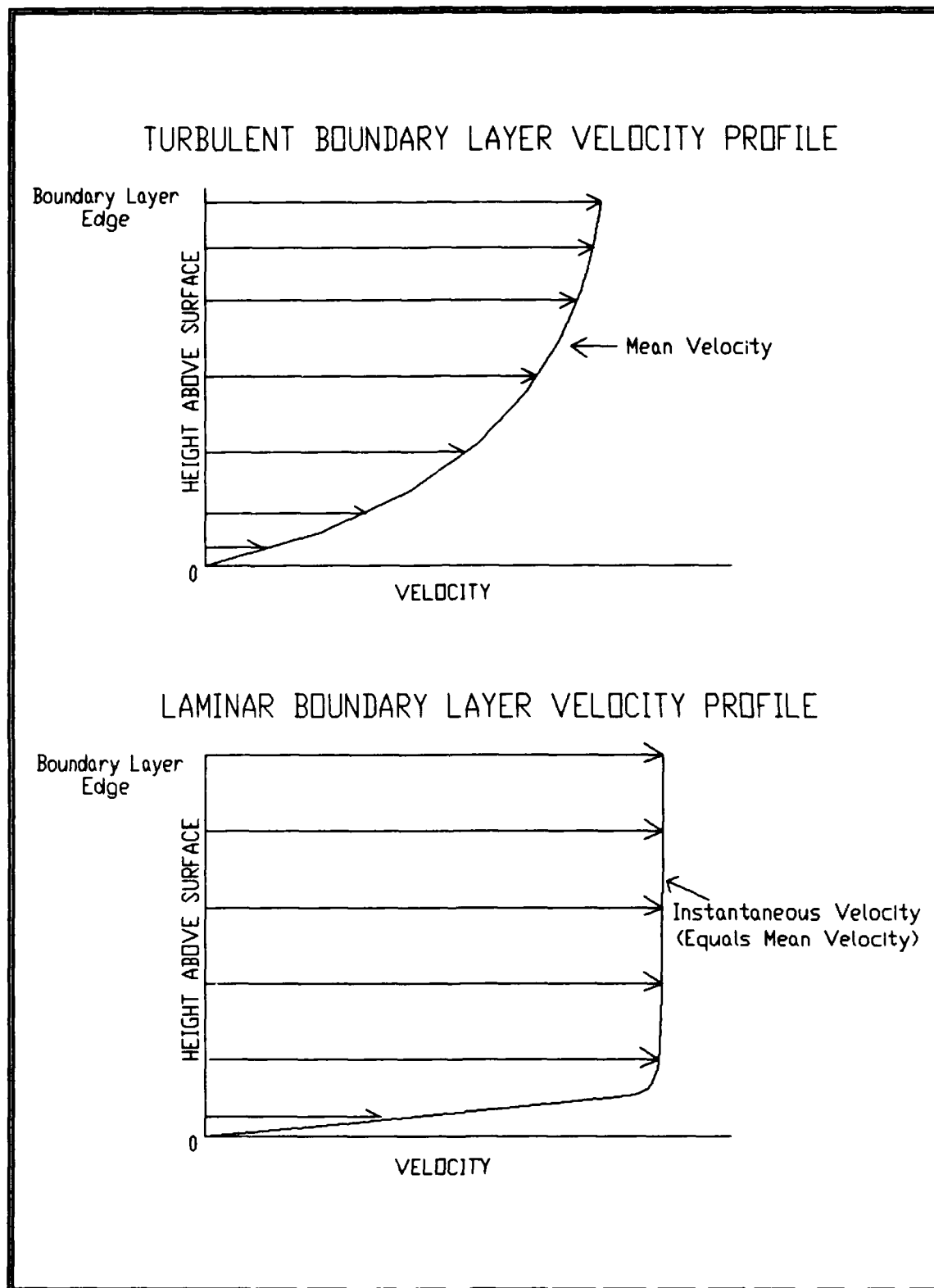
Figure II-3. LAMINAR VERSUS TURBULENT BOUNDARY LAYER PROFILE.
