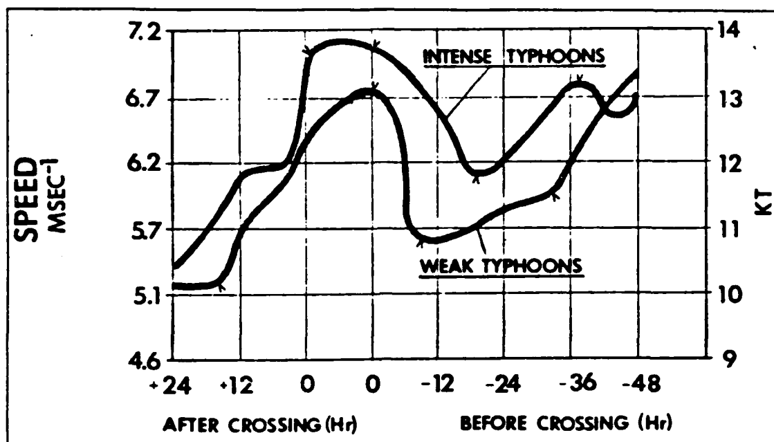
Fig. 5. Average translation speed profiles: Average translation speed profiles for storms crossings the Philippines north of 14.5°N. Land is between the 0 times. Marked points indicate the endpoints of straight line approximations used in the algorithm. (After Sikora, 1976)
