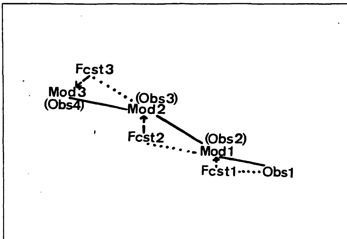
Fig. 13. Illustration of the Option 2/Option 5 procedure: Schematic of the relationship between the input forecasts and the terrain-modified forecasts in program Options 2 and 5. Segments between Obs "N" and Mod "N" is copied from Mod "N" to Fcst "N+1". Terrain modifications are indicated by dashed arrows. Forecast track segments are along dotted lines. Final track including terrain modifications is along the solid lines. Intensity, translation speed and position modifications are allowed to accumulate. This is the procedure used for testing position modifications (see Chapter 5).
