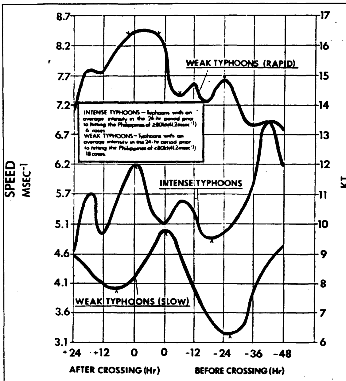
Fig. 6. Average translation speed profiles: As in Fig. 5, except storms crossing the Philippines south of 14.5°N. (After Sikora, 1976)
