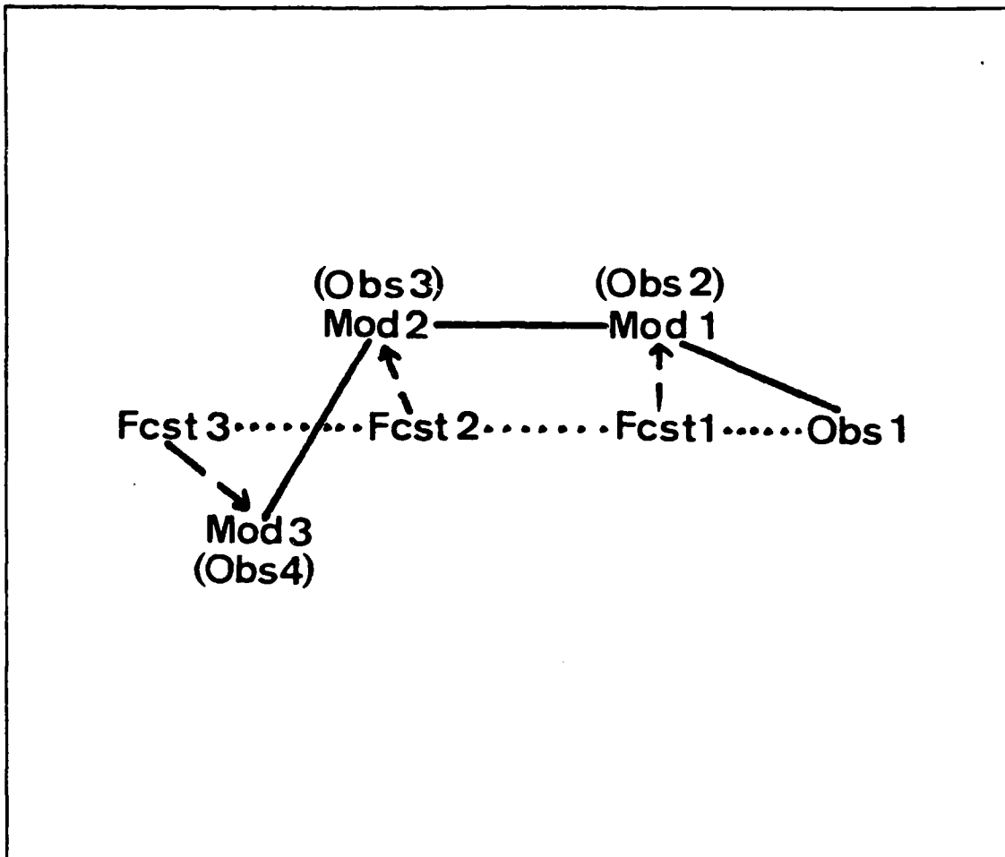
Fig. 12. Illustration of the Option 2/Option 4 procedure: Schematic showing the relationship of the original forecasts and terrain-modified forecasts in Options 2 and 4. Storm track before terrain influences are introduced is from Obs "N" to Fcst "N". Forecast track is along dotted line. Modifications are indicated by dashed arrows. Track including modifications is along the solid line. Terrain modifications do not accumulate. This is the procedure used to test intensity and speed modifications (see Chapter 5).
