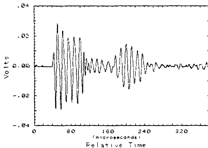
Figure 30. Brass Sphere Reflection, 82.7 kHz N=5
