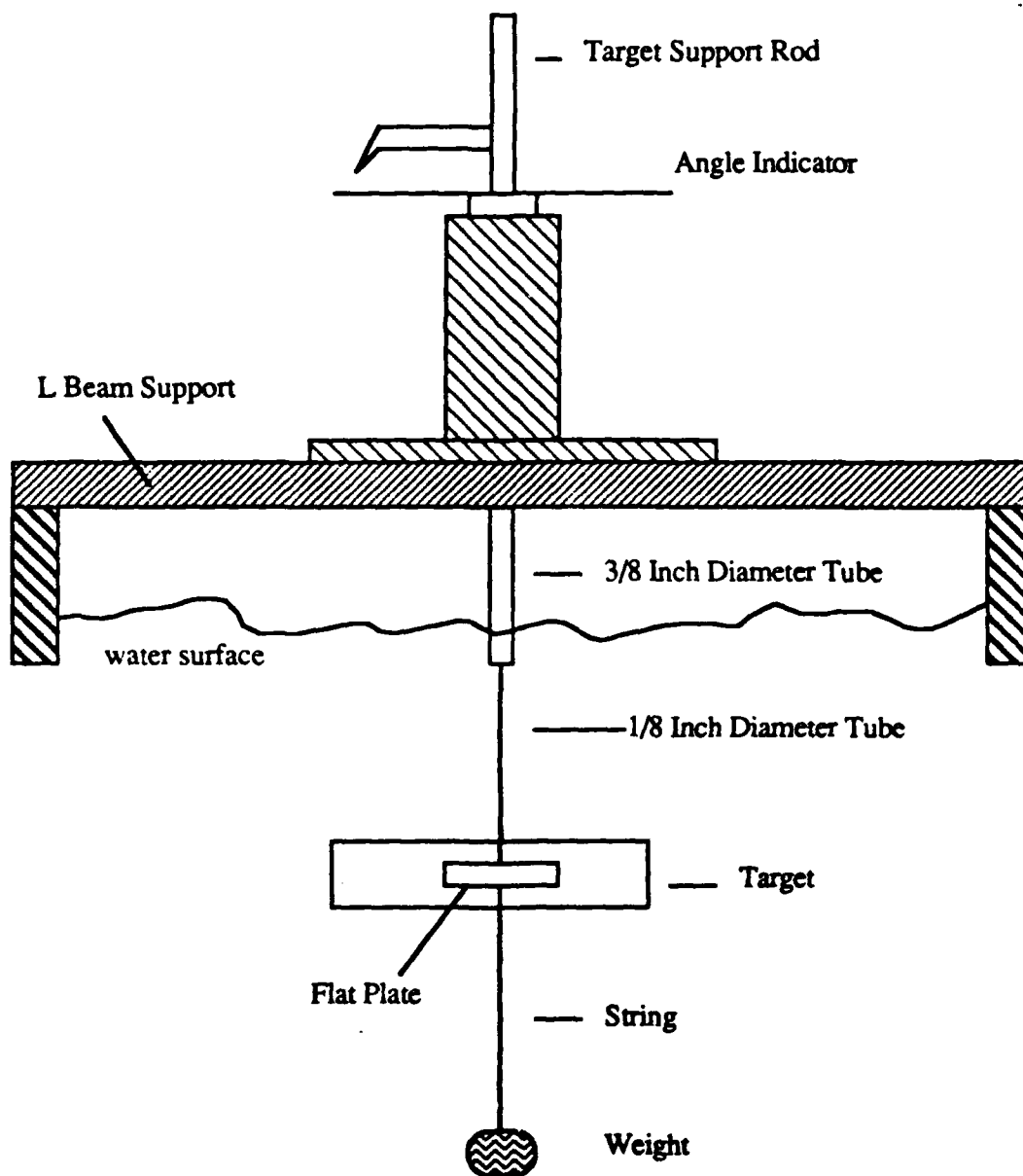
Figure 44. Support Platform Setup
