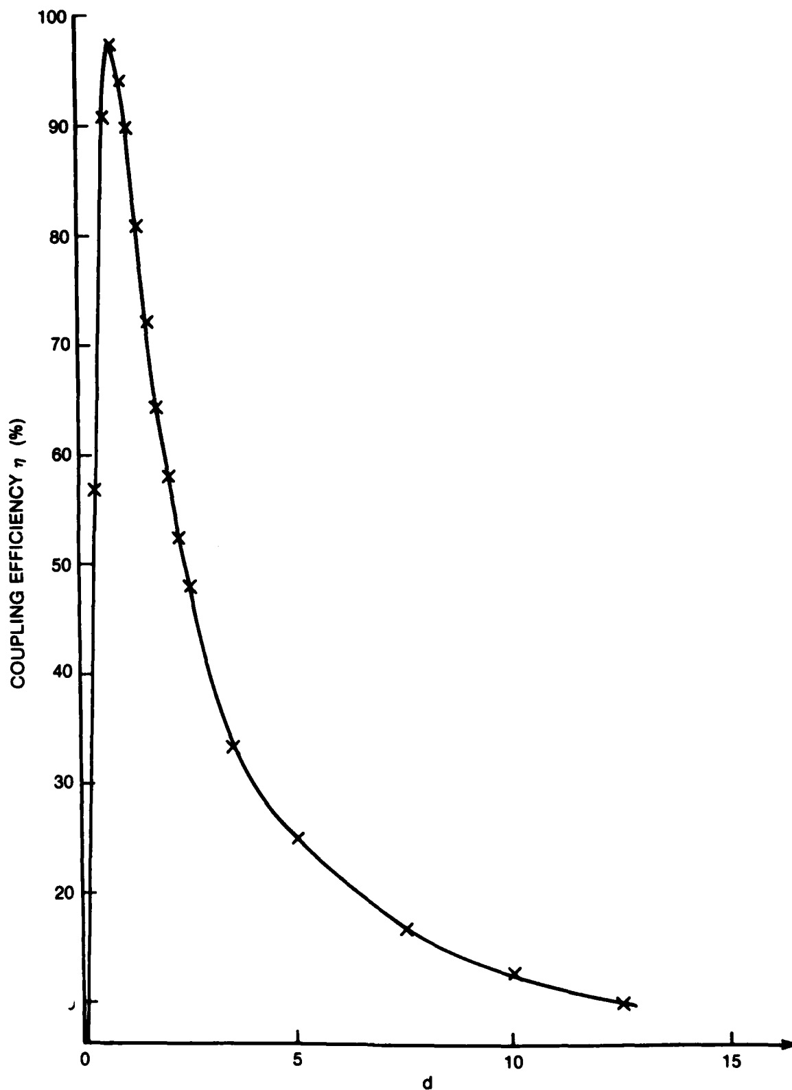
FIGURE 9: COUPLING EFFICIENCY IN THE TE 0 MODE AS A FUNCTION OF THE WIDTH BETWEEN THE FIRST NULLS OF THE ILLUMINATION FOR ILLUMINATION PATTERNS POSITIONED OPTIMALLY
