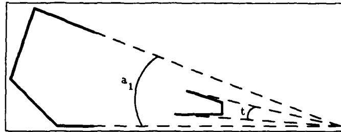
Figure 5.6: The group on the left has a finite projection. After rotating the other group to fall in this projection, "t" represents the aspect the second group presents, and " a_1 " is the angle of projection of the first group. The probability that the second group falls in the first's projection is again approximated by \frac{a_1 - t}{2\pi} .
