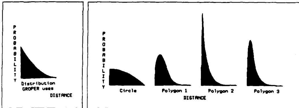
Figure 5.4: On the left, the probability distribution which GROPER uses for the expected distance between groups of edges from the same object. Then, the distribution we would expect from a library of just circles, or just one of the three random polygons shown in figure 3.7.
