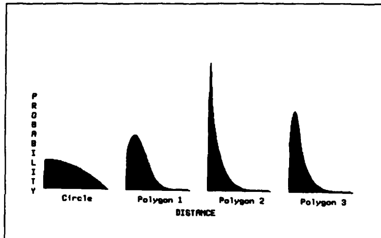
Figure 3.9: The square of the distribution obtained by taking a shape at a random scale, and measuring the distance between randomly chosen points. The distribution is calculated analytically, not experimentally.
