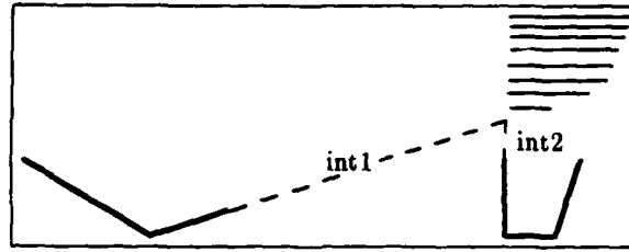
Figure 3.5: int_1 and int_2 , the distance to the intersection of the projections of two groups. The shaded area indicates where the projections intersect.
