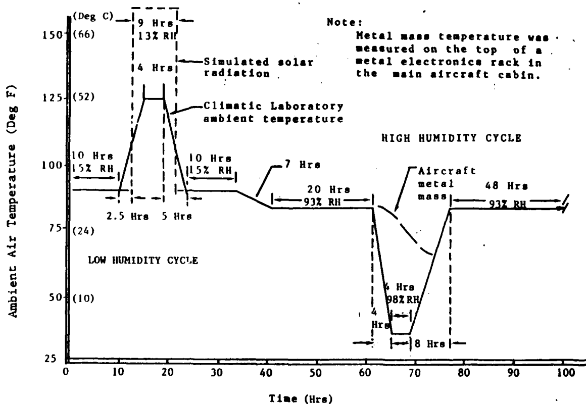
Figure 9. Typical Relative Humidity Cycle
