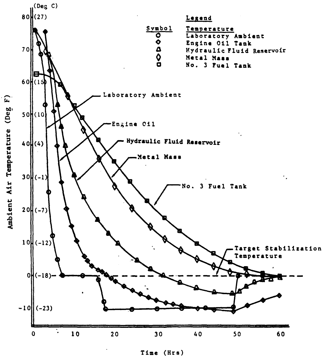
Figure 7. Mass Temperature Stabilization Time History
