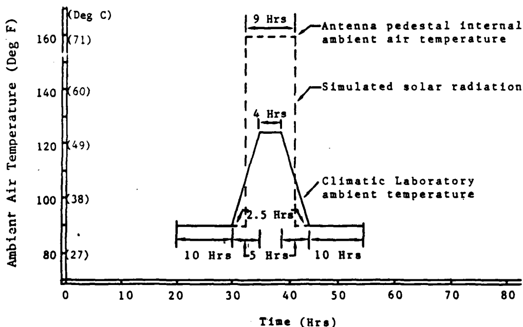
Figure 8. Typical Hot Temperature Diurnal Cycle
