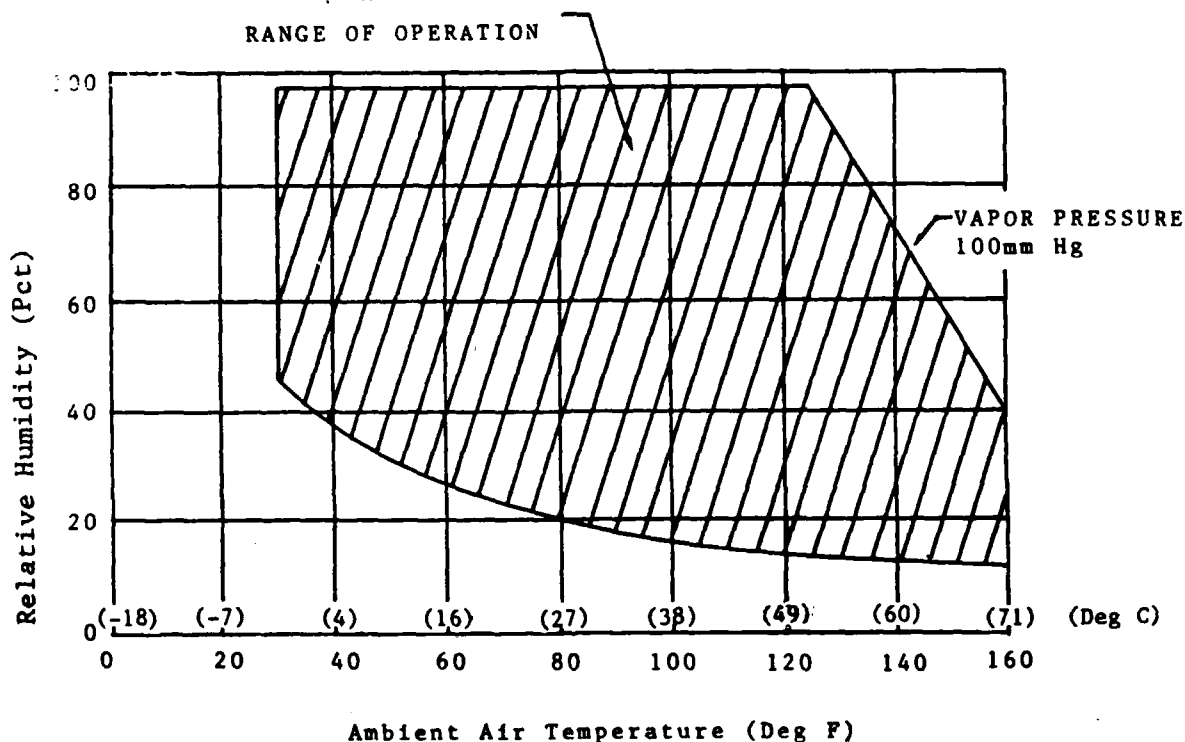
Figure 5. Relative Humidity vs Ambient Air Temperature for Climatic Laboratory Main Chamber
