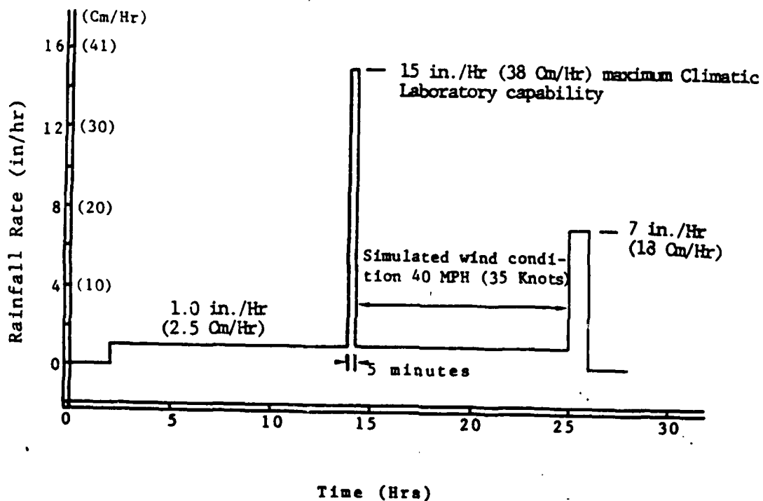
Figure 10. Rainfall Rate Used for Climatic Laboratory Tests
