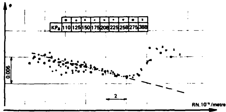
Fig. 12 - 5 metre wind tunnel calibration for August 1985.
