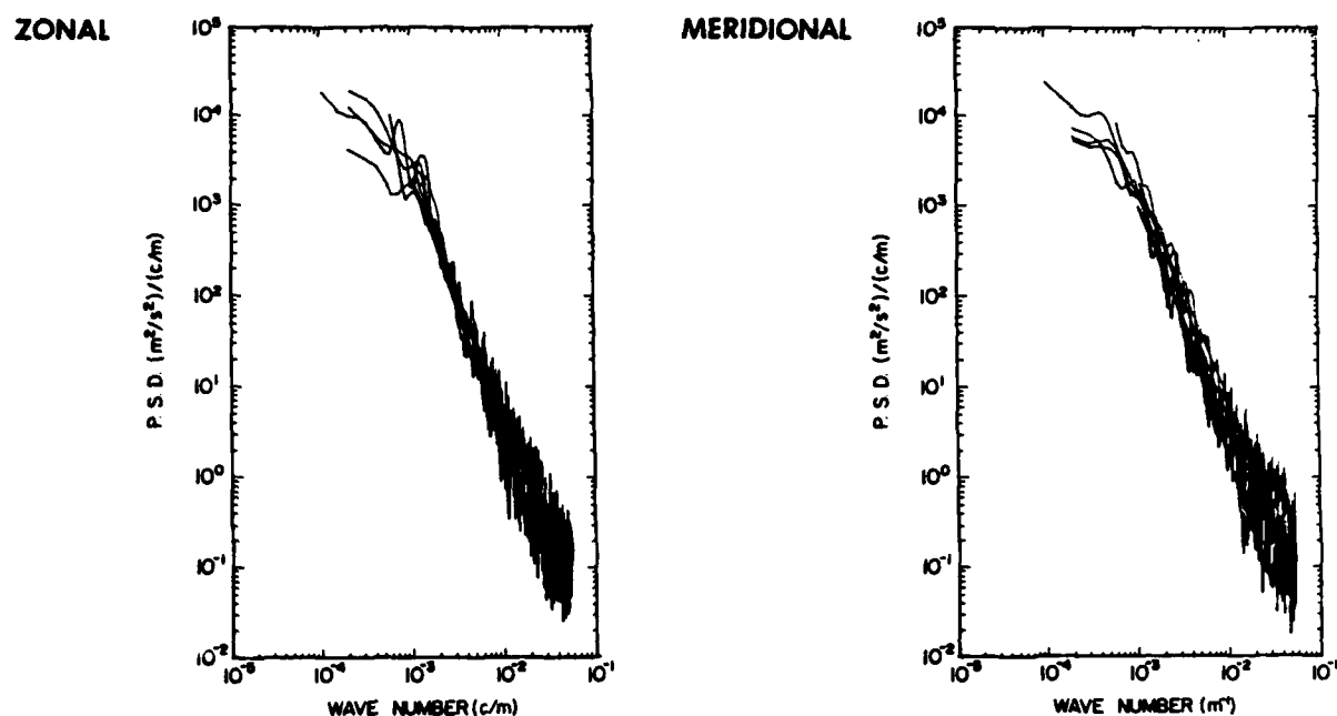
Fig. 3. Power spectral densities (PSD's) of Zonal (A), and meridional (B) velocity components. Table I shows labels, as in Fig. 1.
