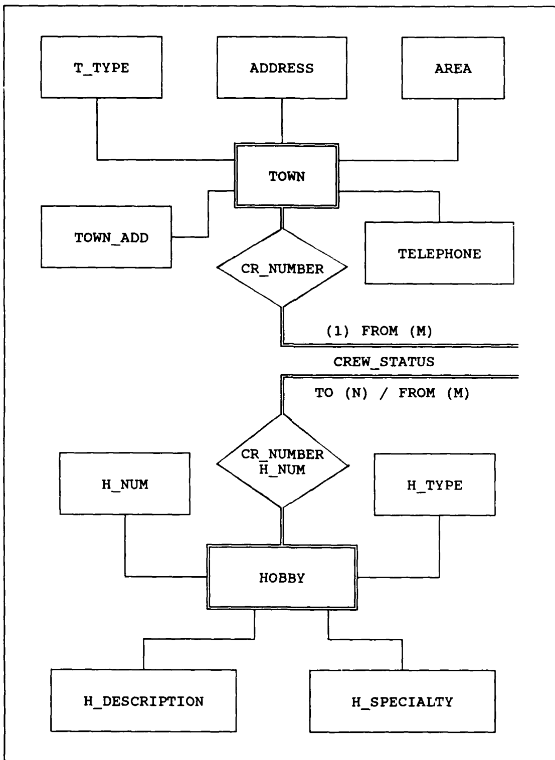
Figure A-3. E-R diagram.
