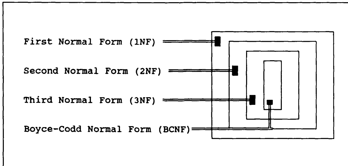
Figure 17. Relationship of normal forms.
