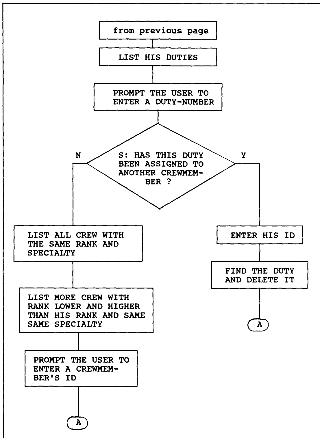
Figure 32. Flowchart of "change-duties" (cont 'd).
