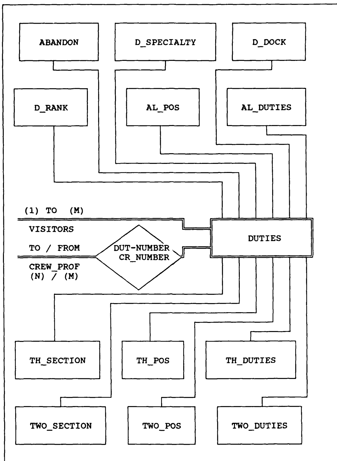
Figure 30. E-R design (cont 'd).
