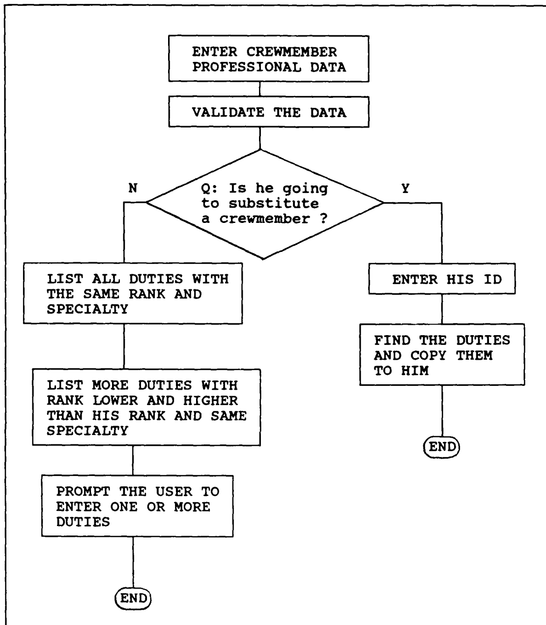
Figure 30. Flowchart of "insertion".
