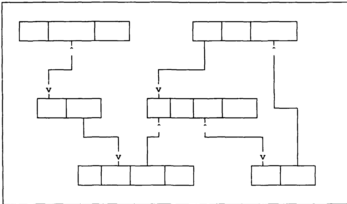
Figure 5. A Network data model.
