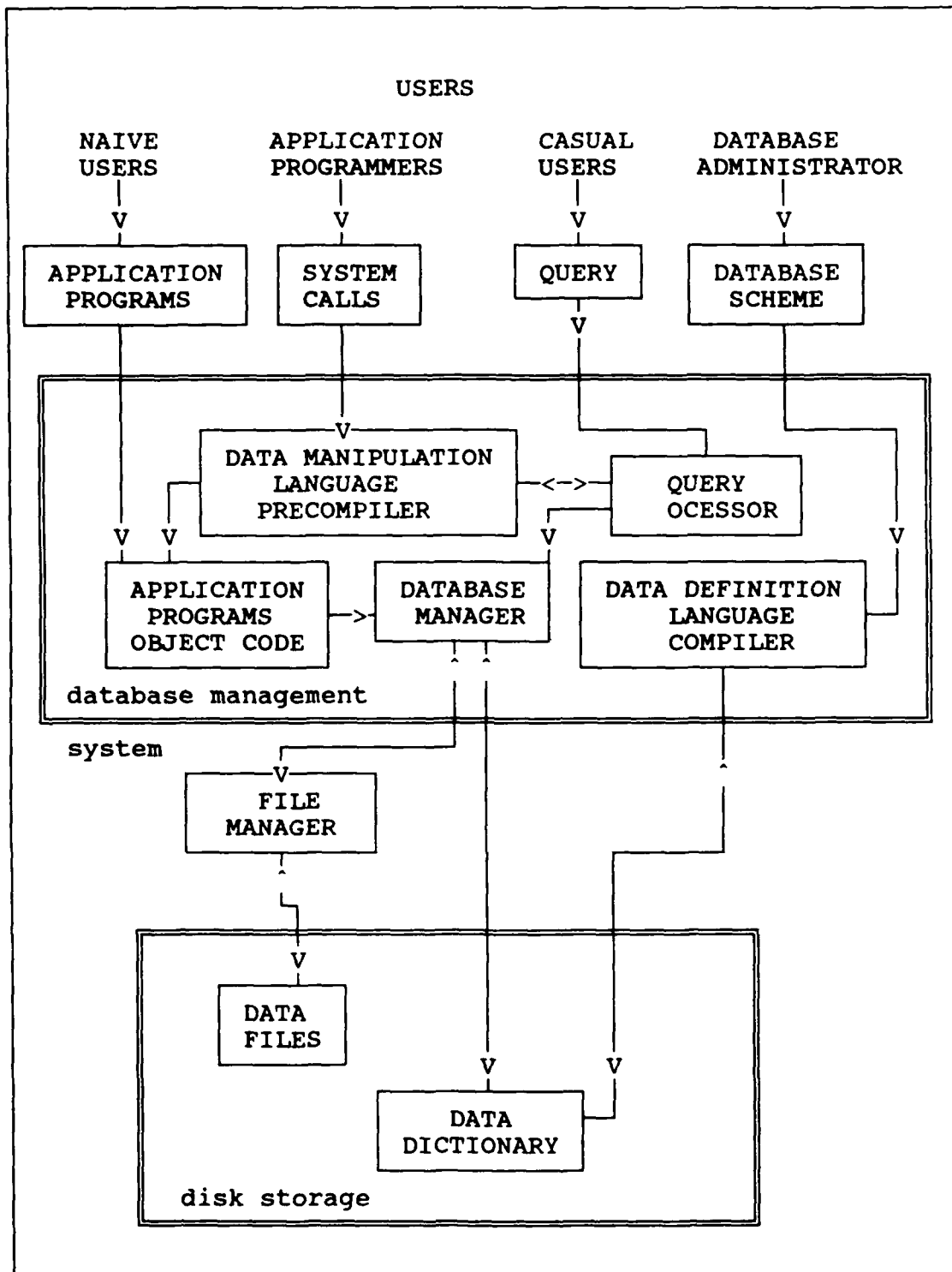
Figure 2. Database components.
