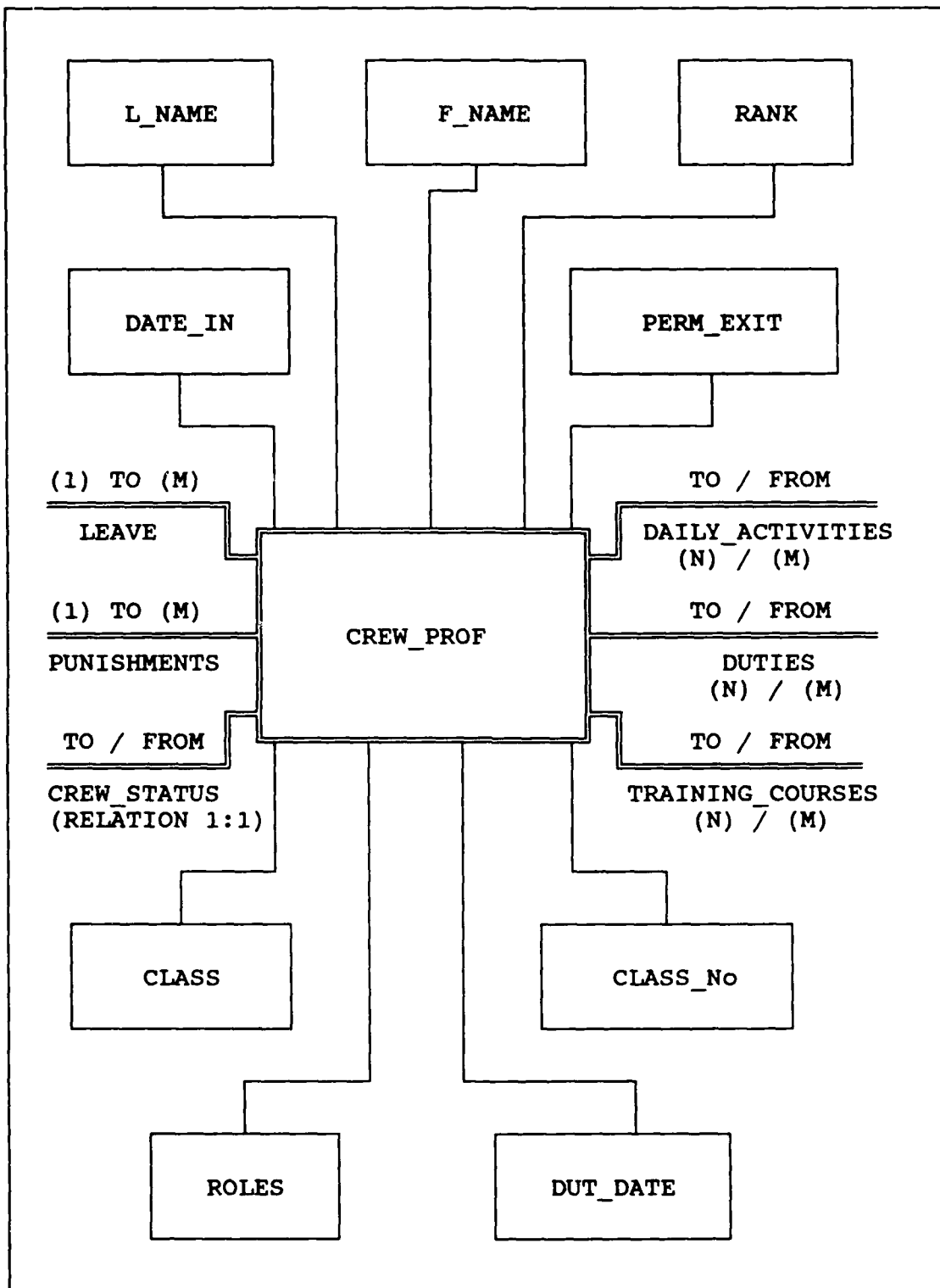
Figure A-3. E-R design (cont 'd).
