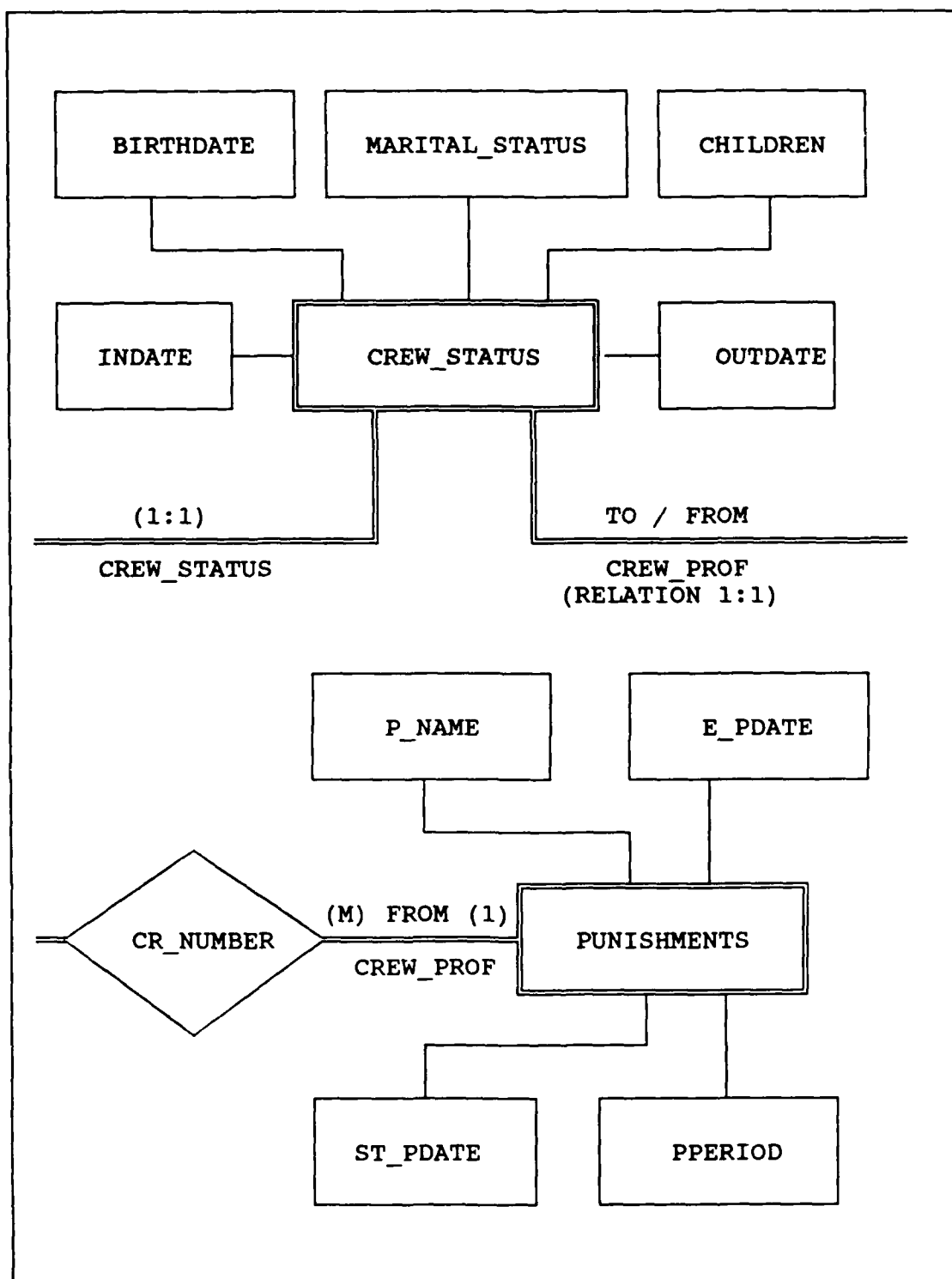
Figure A-3. E-R design (cont 'd).
