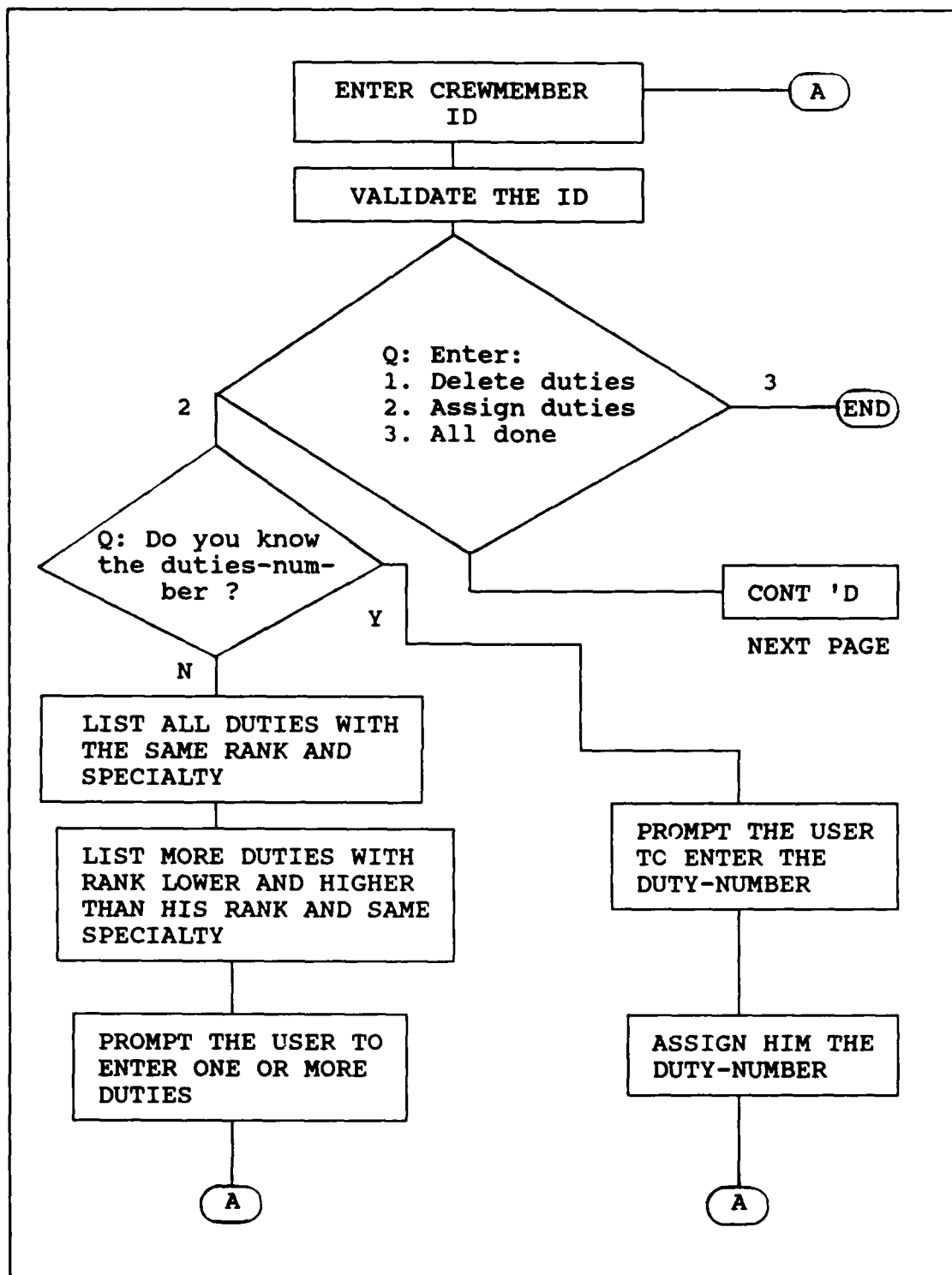
Figure 32. Flowchart of "change-duties".
