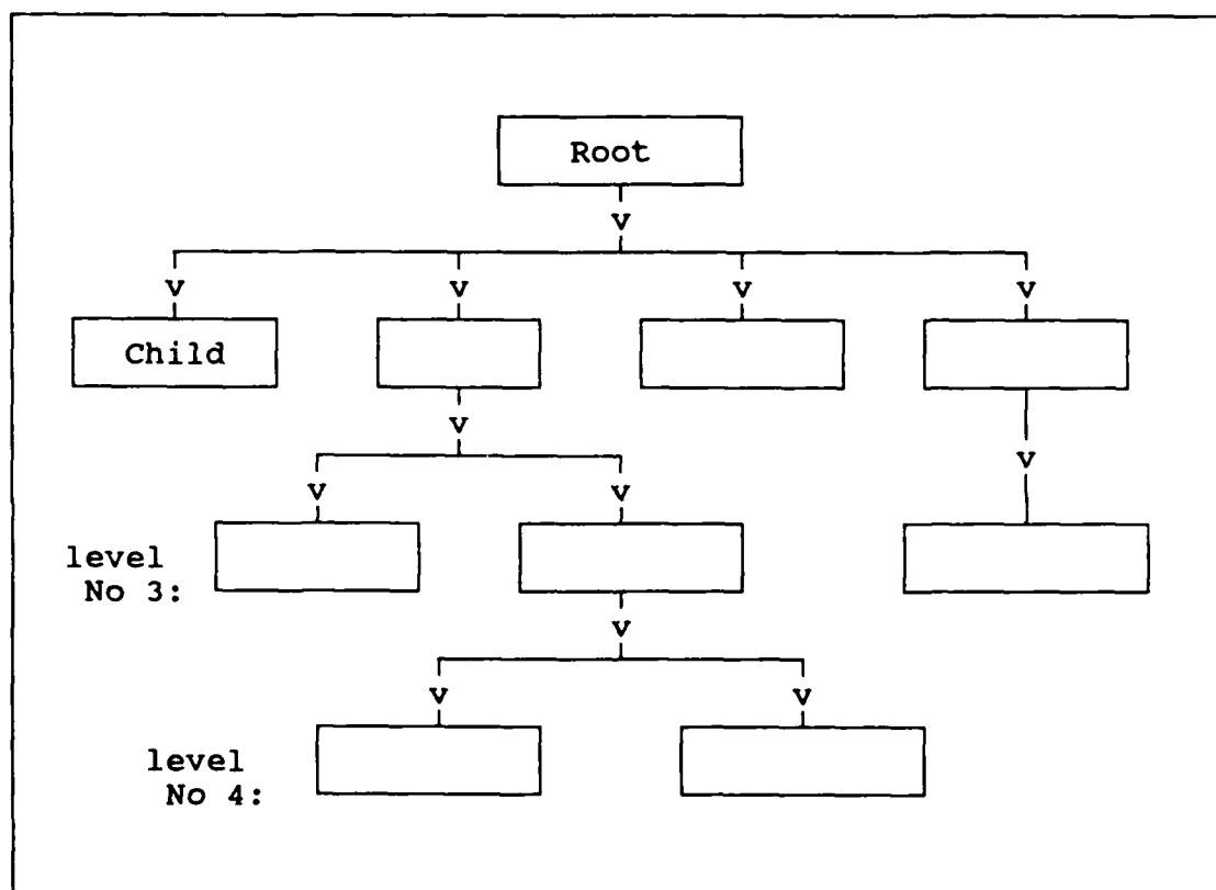
Figure 4. A Hierarchical data model.
