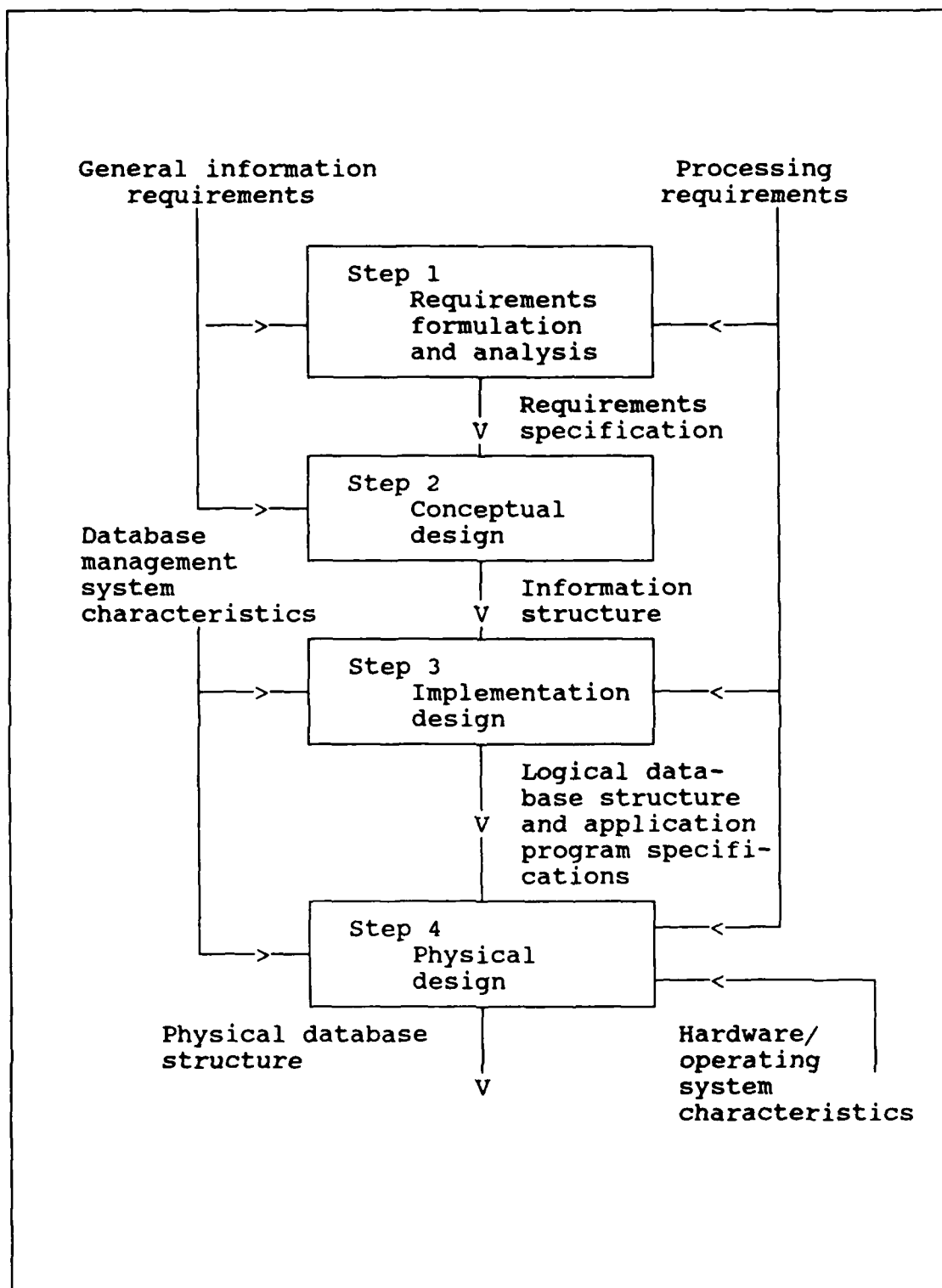
Figure 3. A general model for database design.
