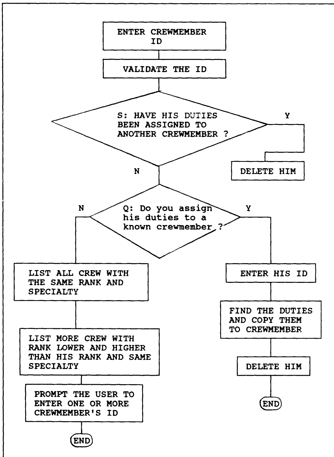
Figure 31. Flowchart of "deletion".
