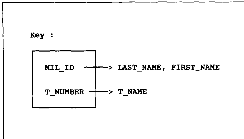
Figure 16. Functional Dependencies.
