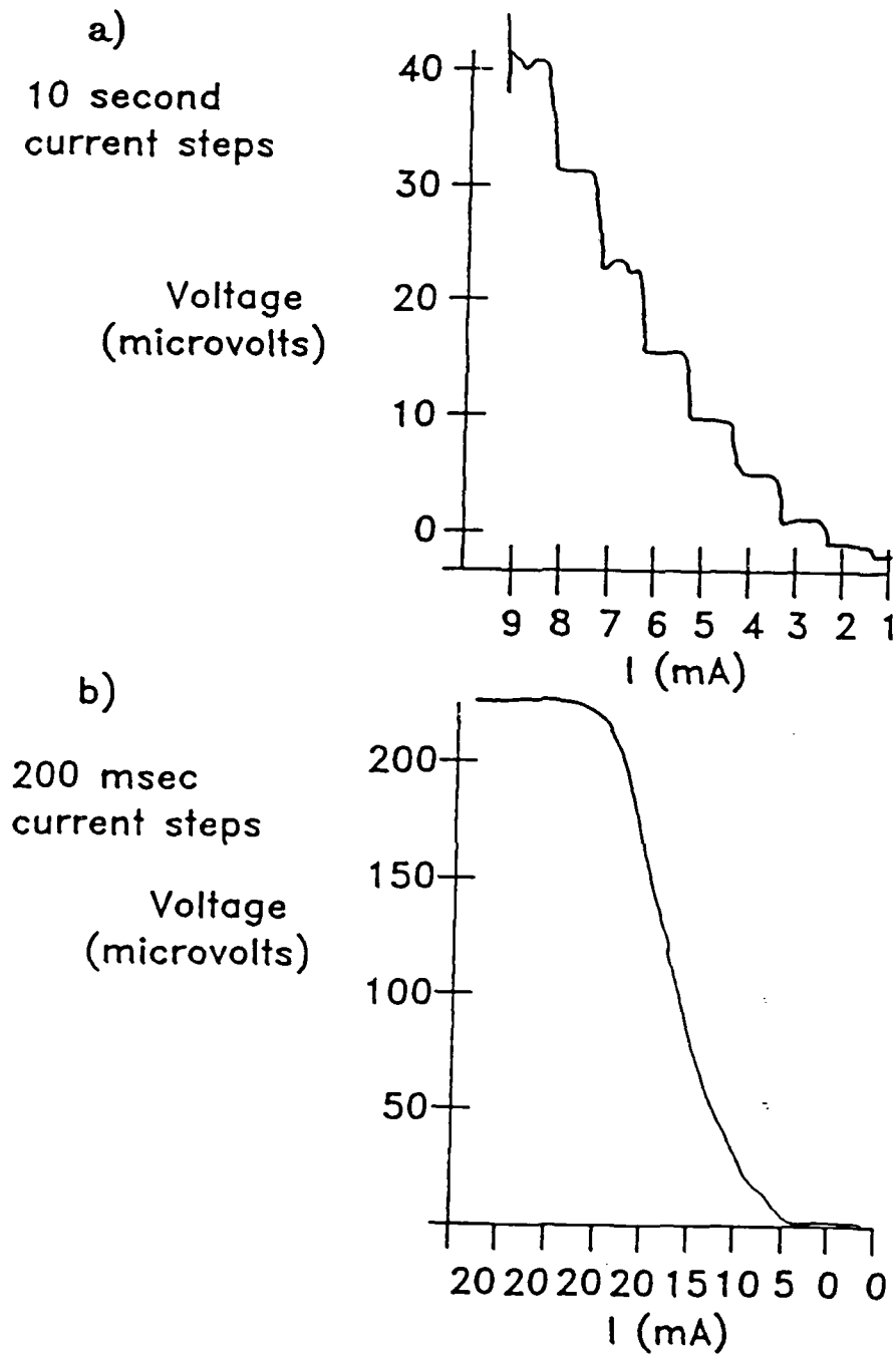
Figure 2.5.2 V-I Data from a Typical J_c Test.
