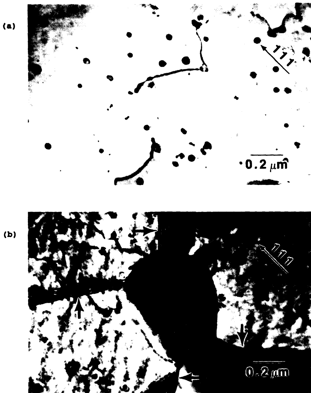
Figure 23. Bright field TEM micrographs of (a) ZrAl_3 particles precipitated coherently in the matrix, and (b) A T_2 precipitate residing on a boundary triple junction. Arrows indicate the boundaries adjacent to the precipitate.
