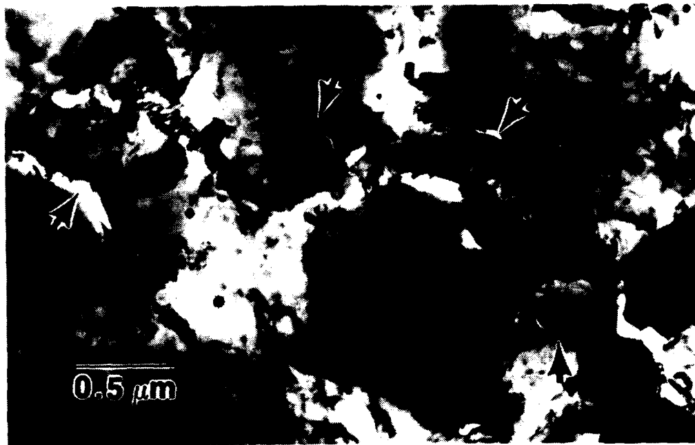
Figure 20. Areas of cracking found in alloy 2090 as forged, aged and rolled at 300°C with 30 min reheat intervals : (a) a fractured T_2 precipitate and (b) cracking associated with particle/matrix decohesion.
