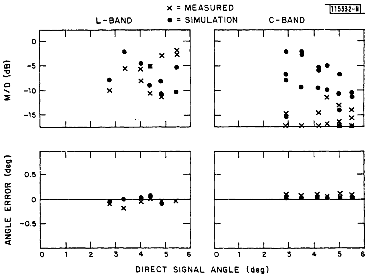
Fig. 5-39. Fort Devens measurement: radial line O-C, L-band and C-band elevation arrays, M/D ratios and angle errors.
