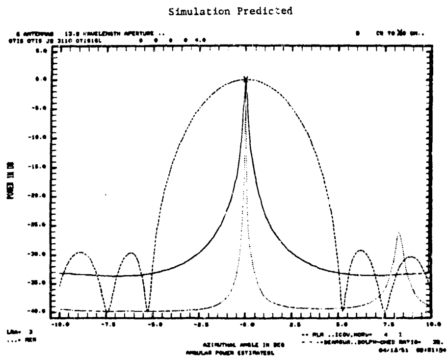
Fig. 5-57. Camp Edwards measurement: J2 range, L-band azimuth array, \theta_{EL} \approx 1.5^\circ .
