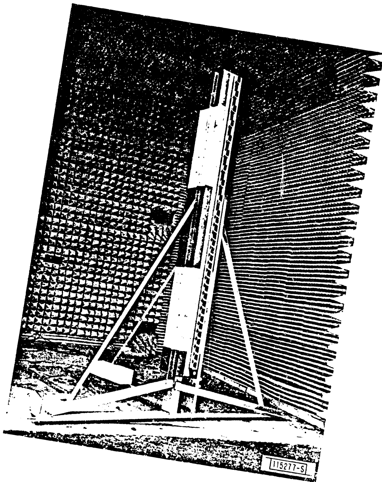
Fig. 2-5. The C-band elevation receiving array.
