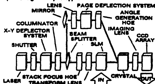
Fig. 1: Optical configuration
