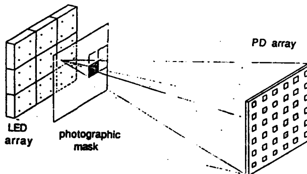
Fig.3 : shadow-casting architecture
