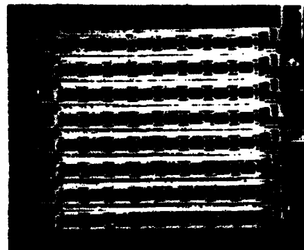
Fig.2 Photomicrograph of 1-D 8 VSTEP arrays. Each VSTEP has 8 windows for light absorption and emission
