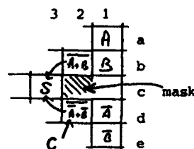
Fig 3-b : Logic implementation of a Half-adder using the interconnection net 3-a
