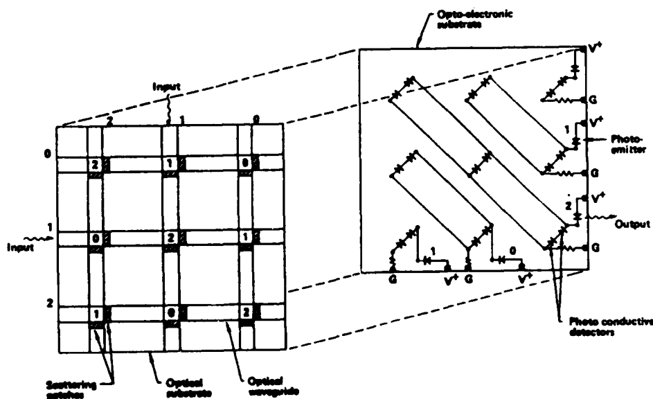
Figure 1 Modulo 3 addition table using dual substrate fabrication.
