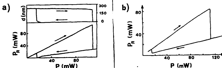
Fig. 3. a) Calculated reflected power P_R = [1-A(d)]P and gap width d and b) observed P_R versus input power P in configuration corresponding to Figs. 1a and 2a. \alpha=42.6^\circ , d=240 nm. Calculations with constant g_s/\lambda=13 nm/mW. \lambda=488 nm. Scan time T=200 s ( ). The prism was a high refractive index ( n_p=2.05 ) glass prism.
