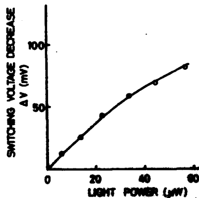
Fig.4 Switching voltage decrease with light incident on the VGS
