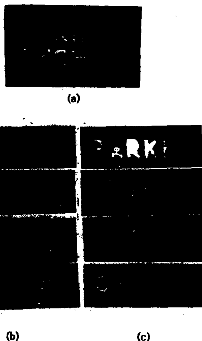
Fig.2 (a) Stored image in BaTiO 3 (b) Partial input image (c) Reconstructed image
