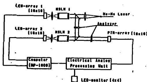
Fig. 1 Schematic diagram of experimental OPTICAL ASSOCIATRON
