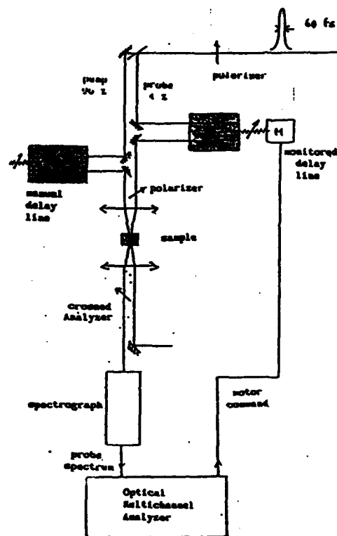
Fig. 1 : Principle of our Kerr effect experiments
