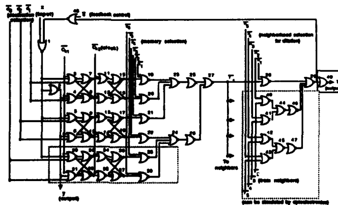
Figure 2. The circuit diagram of a 48-gate processing element of the DOCIP-array4.
