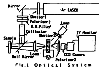
Fig.1 Optical System
