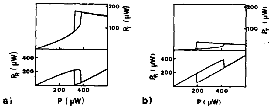
Fig.3. Reflected power P_R and transmitted power P_T versus input power P for FP described in Fig. 2, with a) 30 nm and b) 50 nm thick Au mirror coatings calculated with the constant S/\lambda=330 nm/mW, and g=0.5 . d_0=275 nm.
