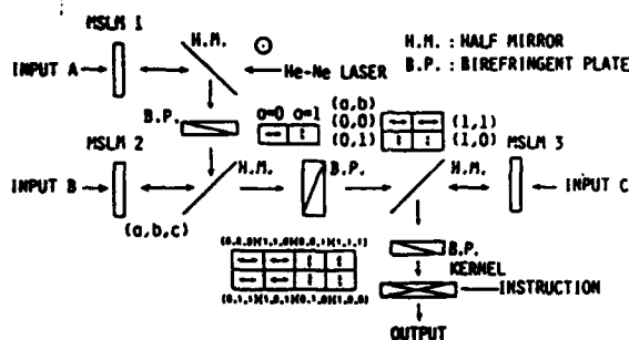
Fig. 1 Experimental setup of optical processor
