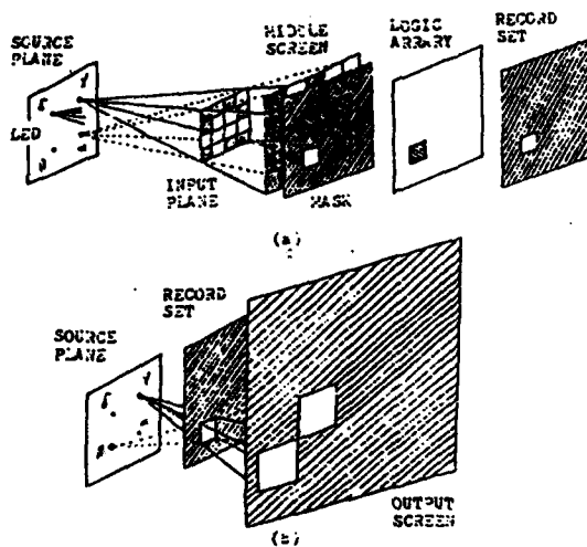
Fig. 2. Schematic diagrams of implementing symbolic substitution using shadow-casting; (a) recognition phase; (b) substitution phase.
