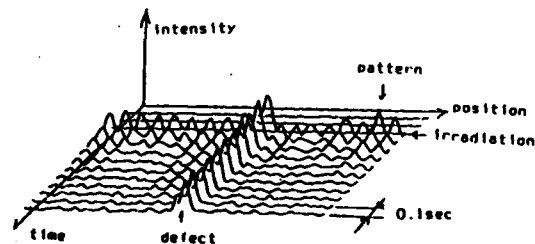
Fig.2 decrease in signals of the pattern and the defect with the time after the laser irradiation
