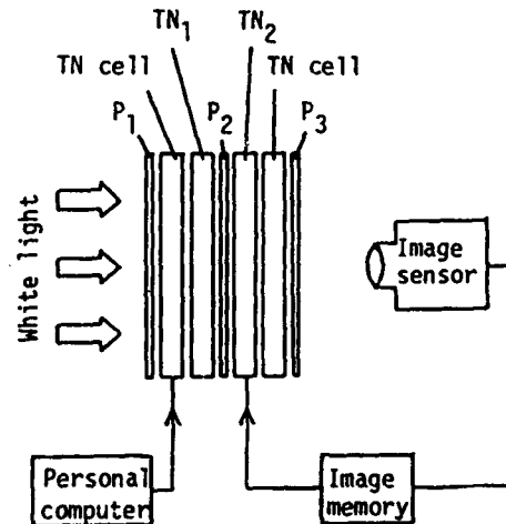
Fig.2 Configuration for iterative processing
