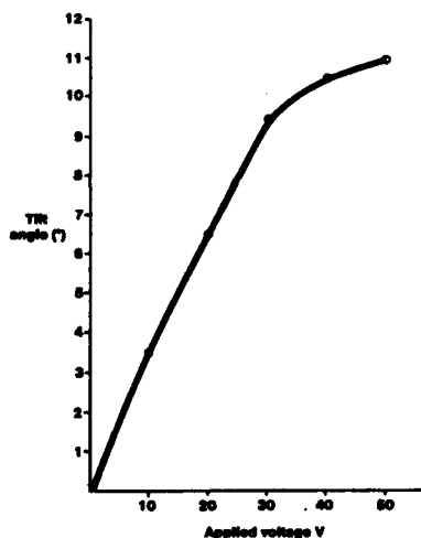
Fig.1 Tilt angle V applied voltage @ 60°C in 2 \mu m thick device
