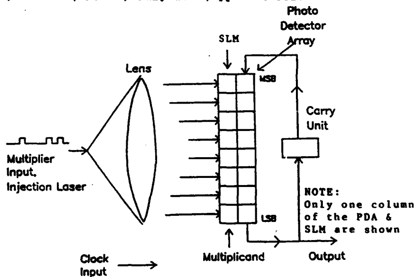
Fig. 1 Optical Distributed Arithmetic Unit
