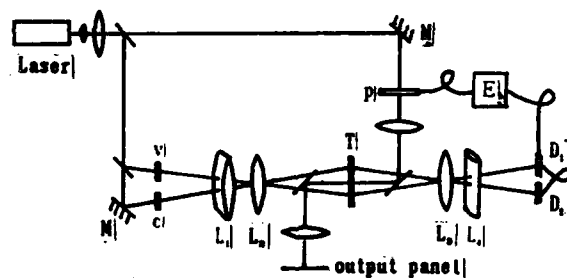
Fig. 2 Diagram of improved optical associative memory
