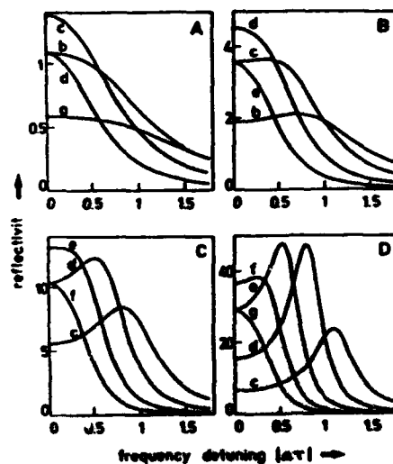
Fig. 3: Phase conjugate reflectivity R versus frequency detuning |Q\tau| . The parameters are coupling strength |\gamma_{01}| and the pump beam intensity ratio g . |\gamma_{01}| = 2 (A), 3 (B), 4 (C), 5 (D). g = 1 (a), 2.7 (b), 7.4 (c), 20 (d), 66 (e), 148 (f), 403 (g).
