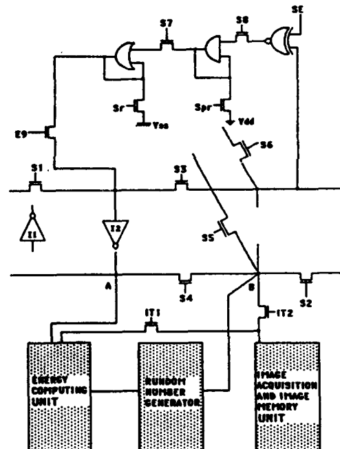
Figure 2 : Processing Element structure.
