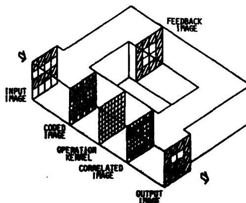
Fig.2 Schematic diagram of the OPALS
