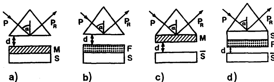
Fig. 1. Schematic of set-up for prism coupler excitation of a,c) surface plasmons, and b,d) guided modes in a planar waveguide. P , incident power; P_R , reflected power; \alpha , angle of incidence in glass prism; M , metal film (e.g., Au or Ag); F , waveguiding film; S , glass substrate (e.g. of refractive index n_s=1.5 ); \bar{S} , glass plate; d , width of air gap.
