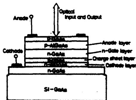
Fig.3 Cross sectional view of the VSTEP
