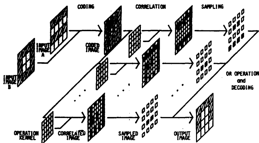
Fig.1 Processing procedures of optical array logic
