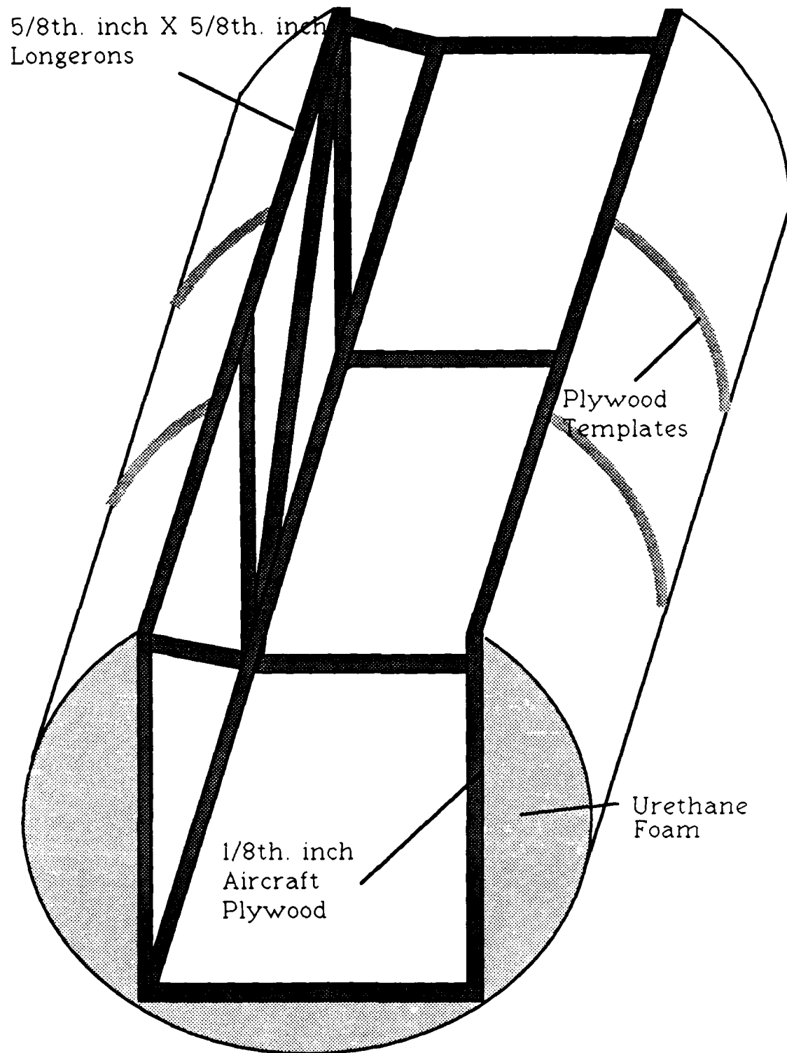
Figure 3. Typical Fuselage Cross Section
