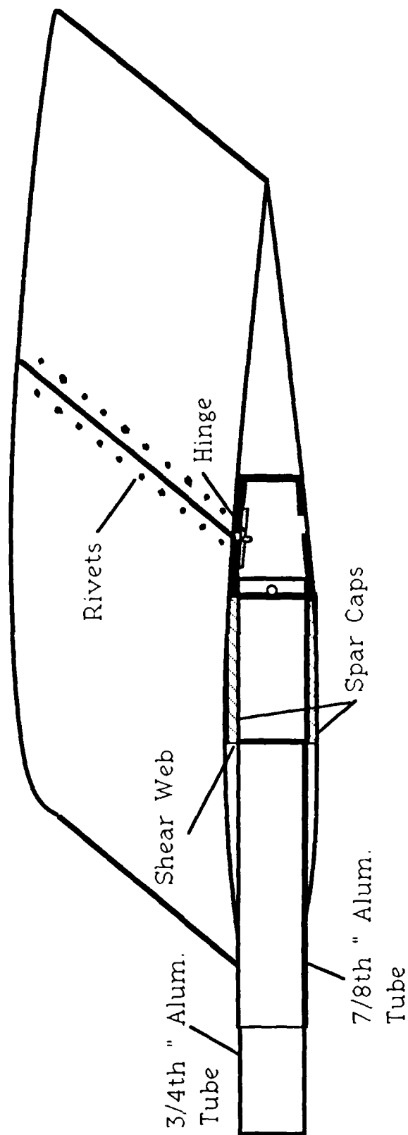
Figure 8. Horizontal Tail With Internal Housing Tube
