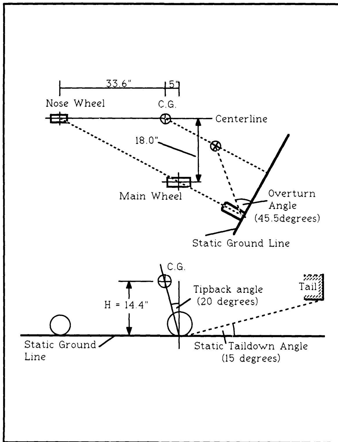
Figure 9. Landing Gear Geometry
