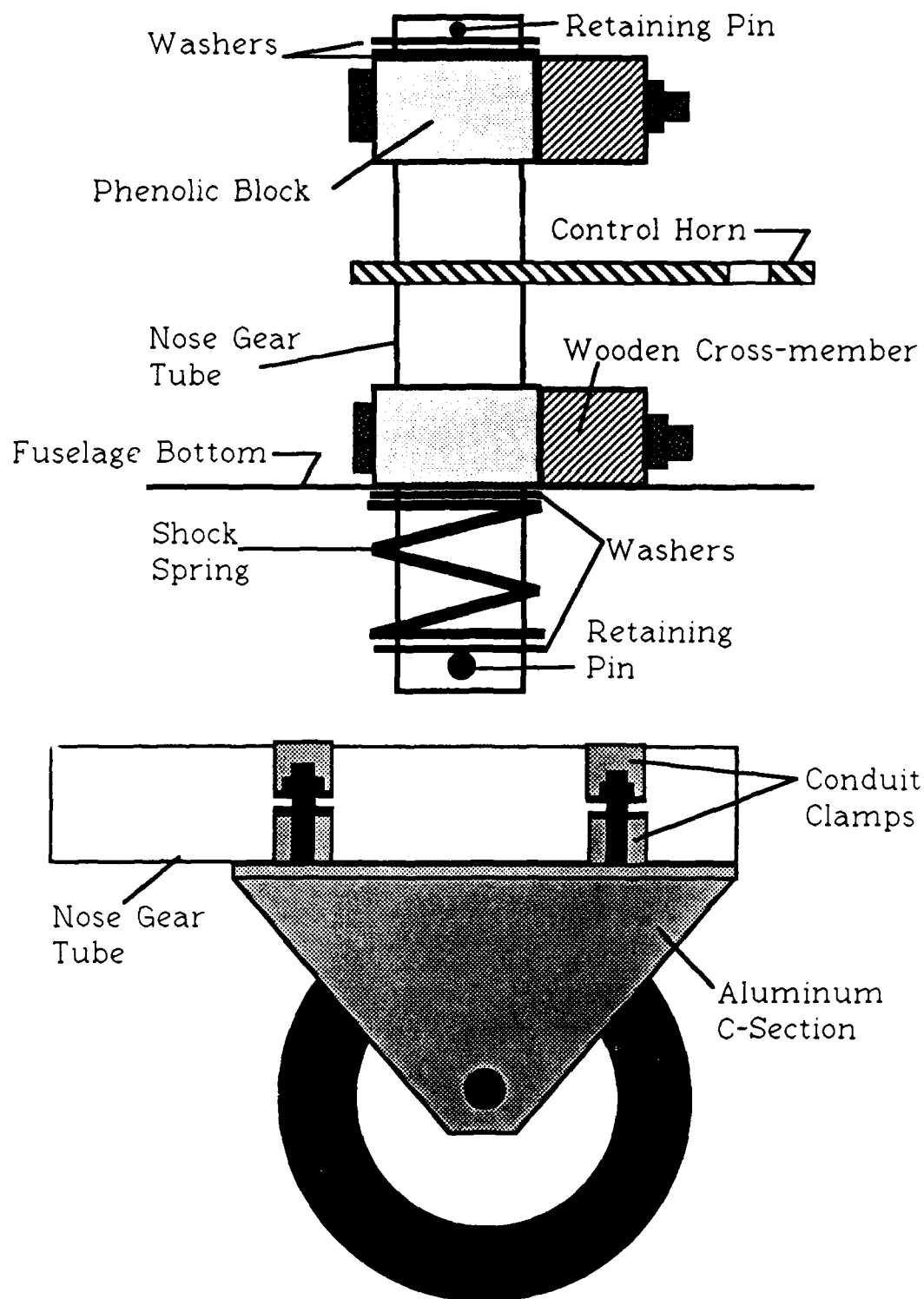
Figure 10. NoseGear Upper and Lower Attachment Detail
