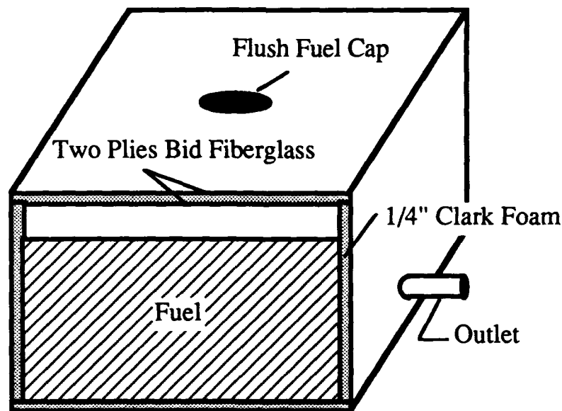
Figure 1. Fuel Tank Cross Section
