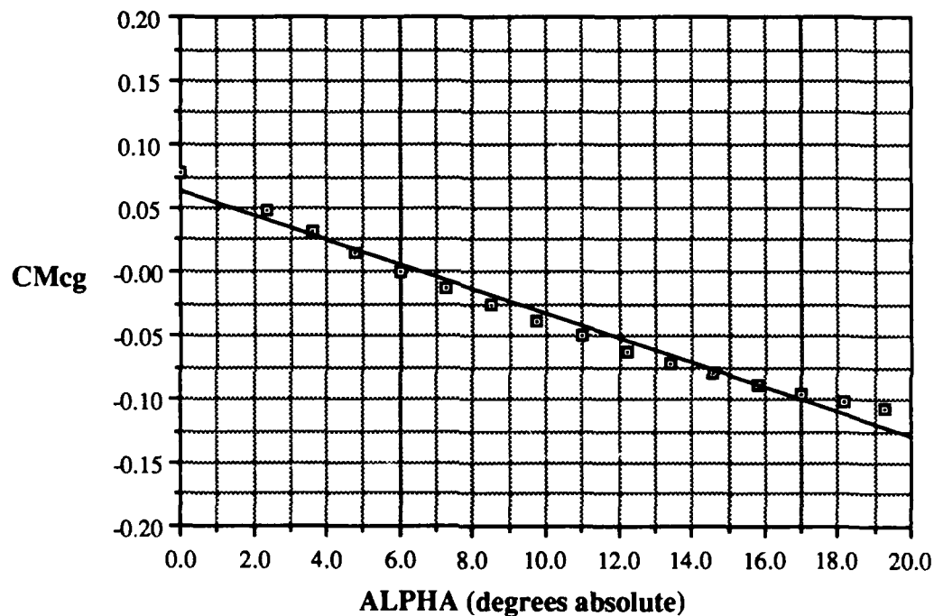
Figure 12. CM_{cg} versus \alpha with i_t + \epsilon_o = 6.1
