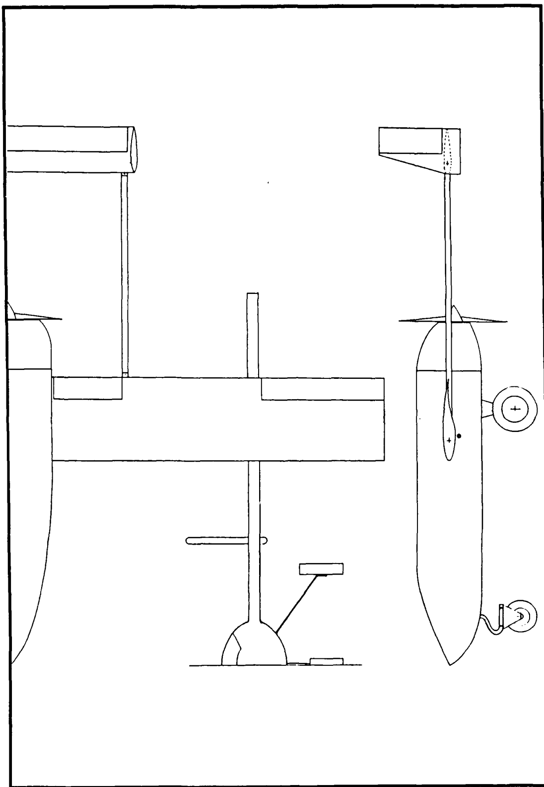
Figure 2. NPS RPV (3 View Drawing)
