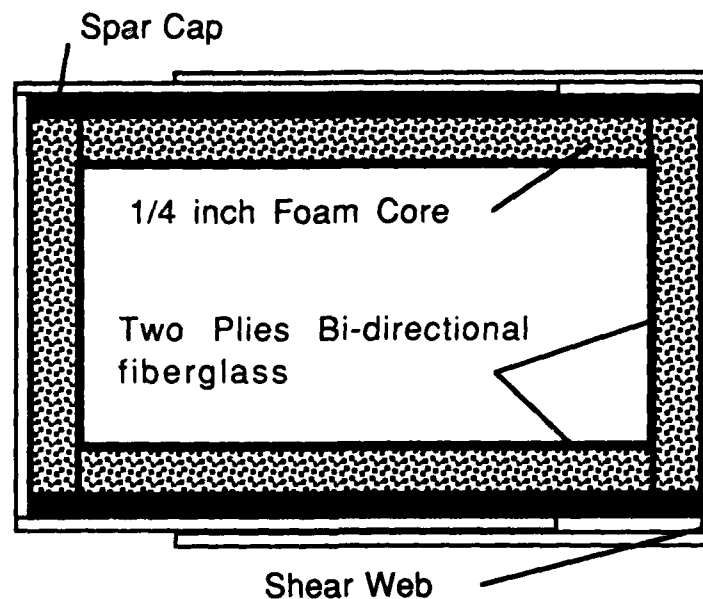
Figure 6. Spar Box Cross Section
