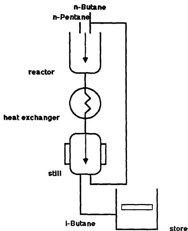
Figure 8: Butane isomerization
