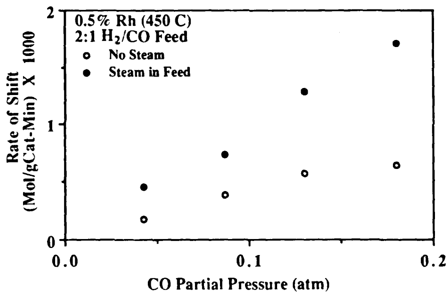
Figure 4.58 Comparison of Shift Rate versus CO Partial Pressure With and Without Steam 450°C
