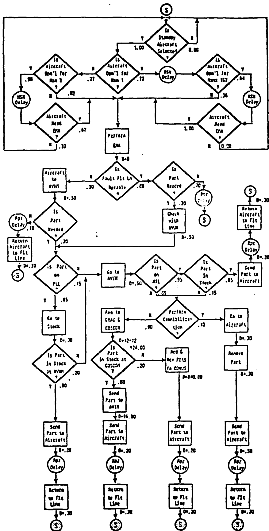
FIGURE 2. AHC AIRCRAFT AVAILABILITY MODEL
