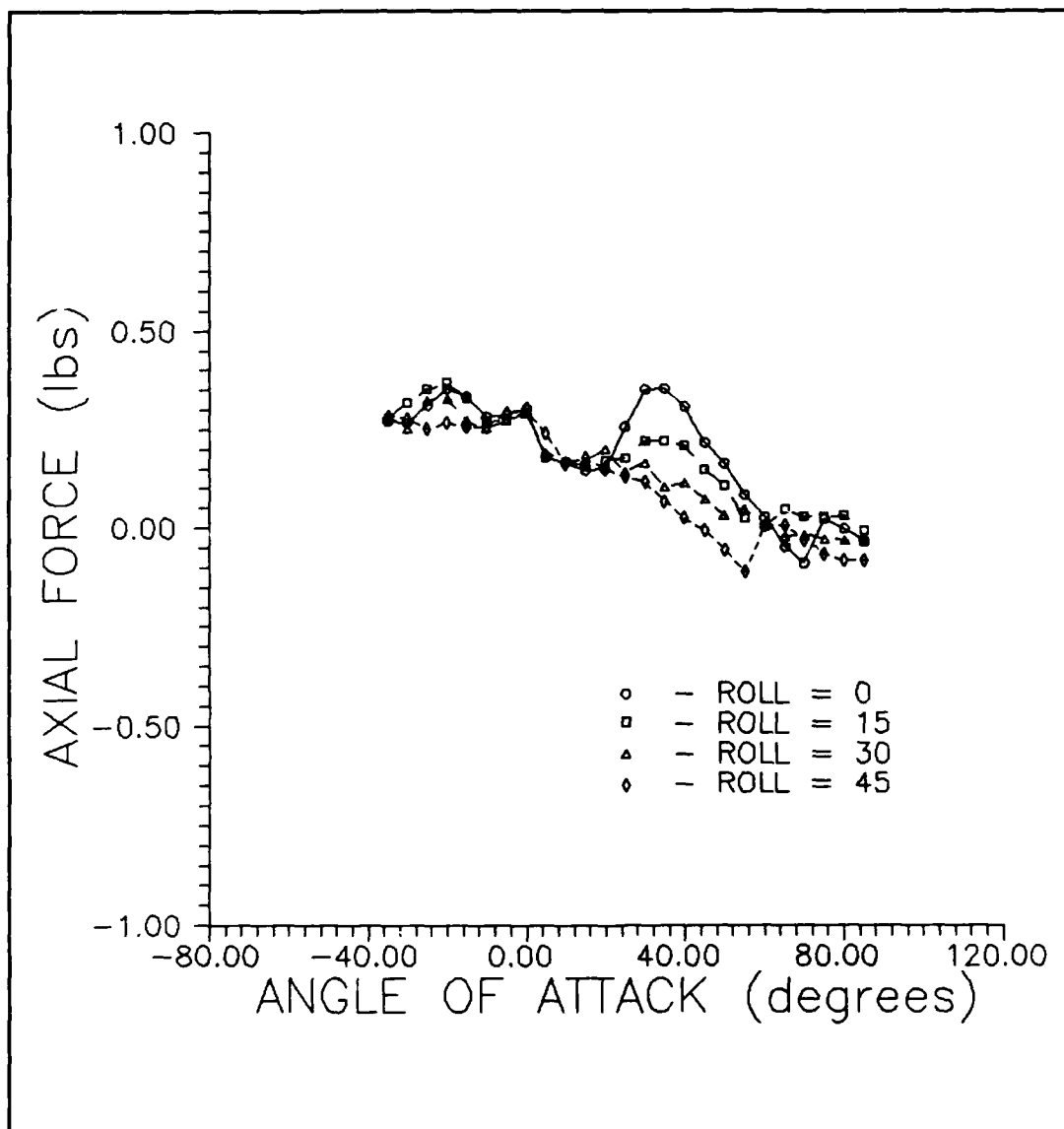
Figure 139. Axial Force (Roll)
