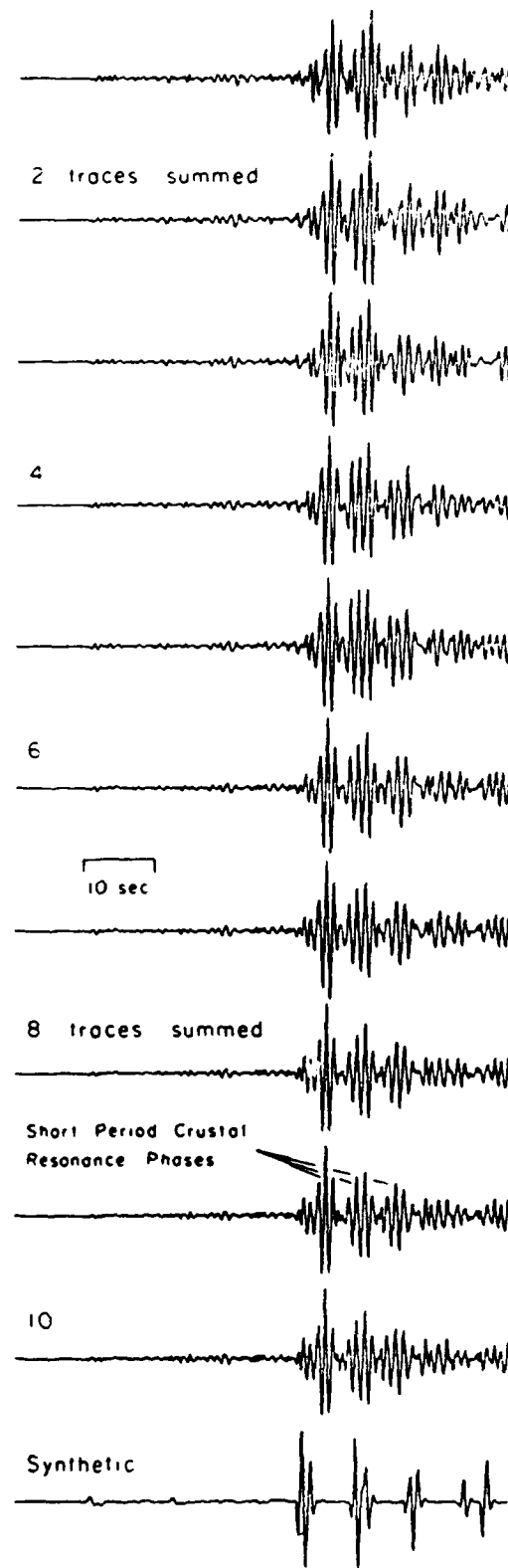
Figure 27. The crustal resonance phases for Yucca events are separated from the noise by stacking. The synthetic at the bottom merely indicates that the phases have approximately the right timing and amplitude.
