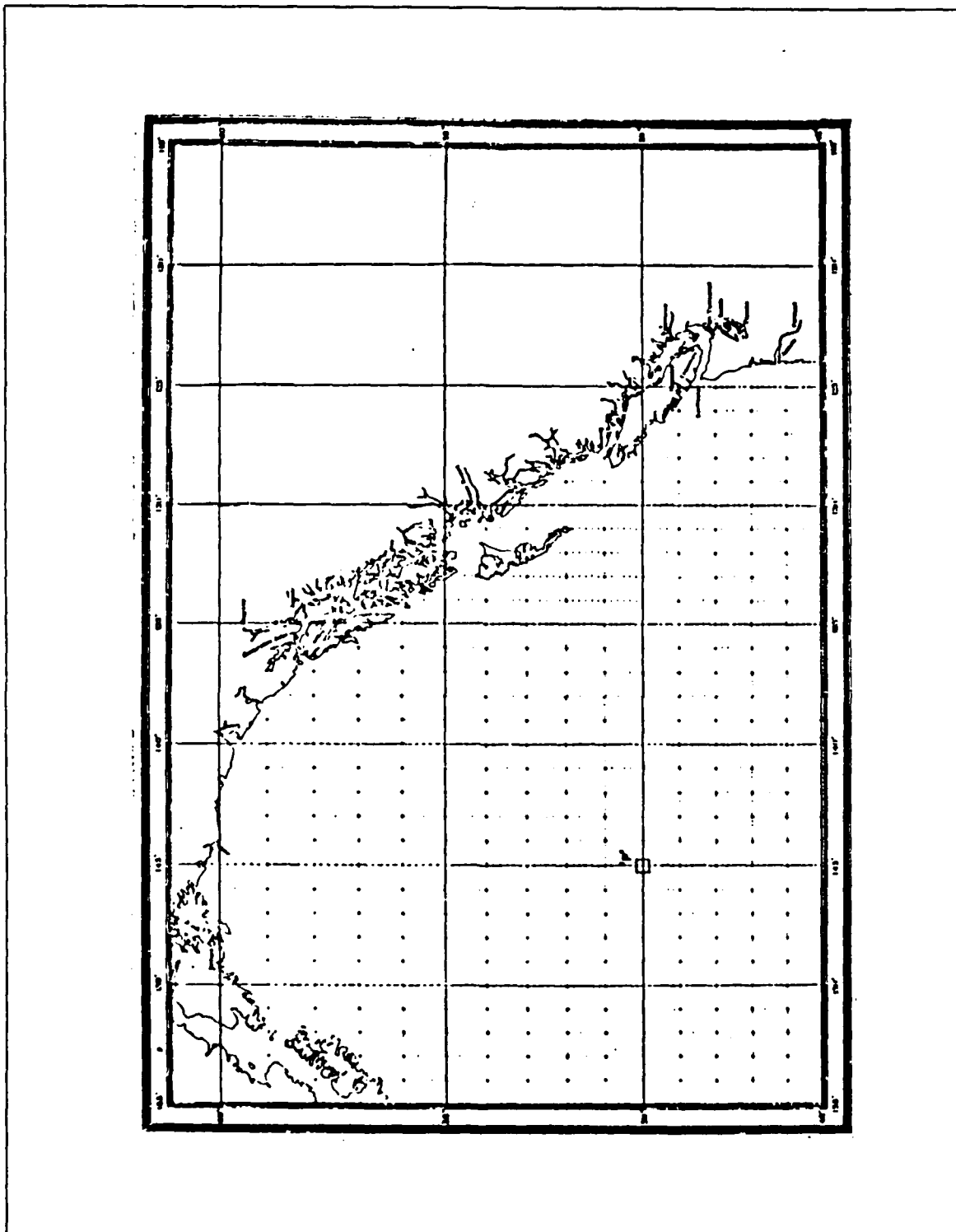
Fig. 1. Region Surrounding Ocean Station "P" (from Tabata, 1961)
