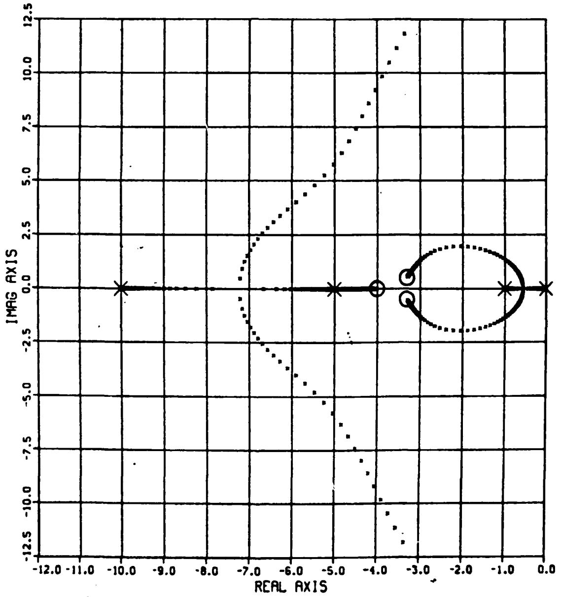
Figure 3.8.b Compensated System Root Loci with Zero Offsets
