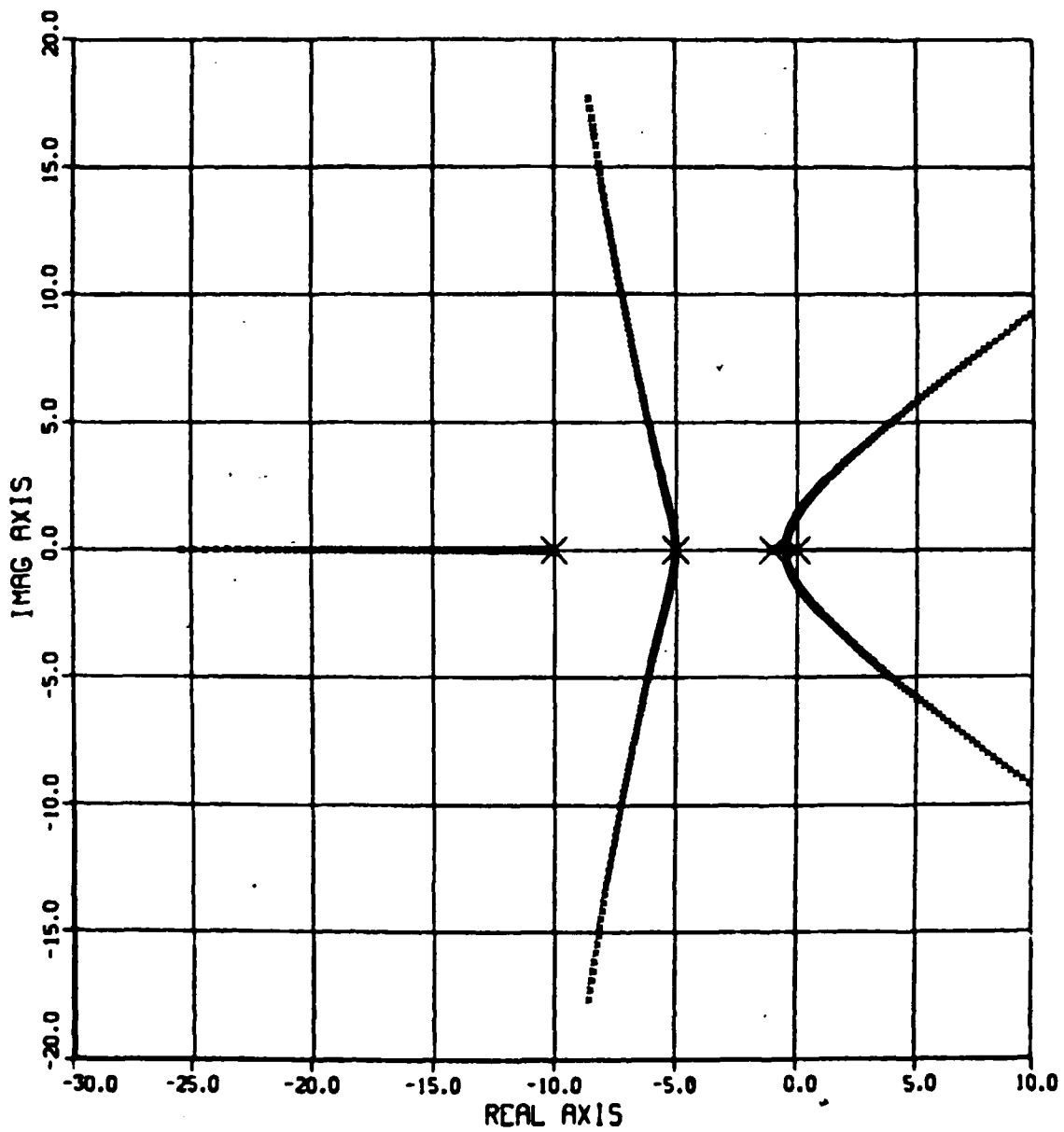
Figure 3.7.a Uncompensated System Root Locus Plot
