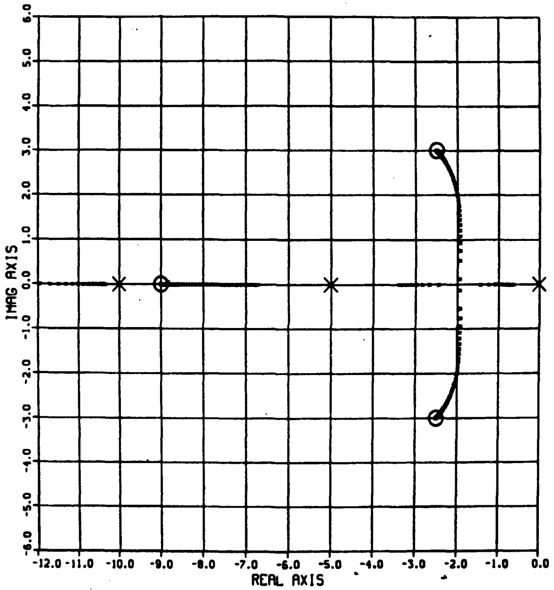
Figure 2.4.c Compensated System Root Loci with Zero Offsets
