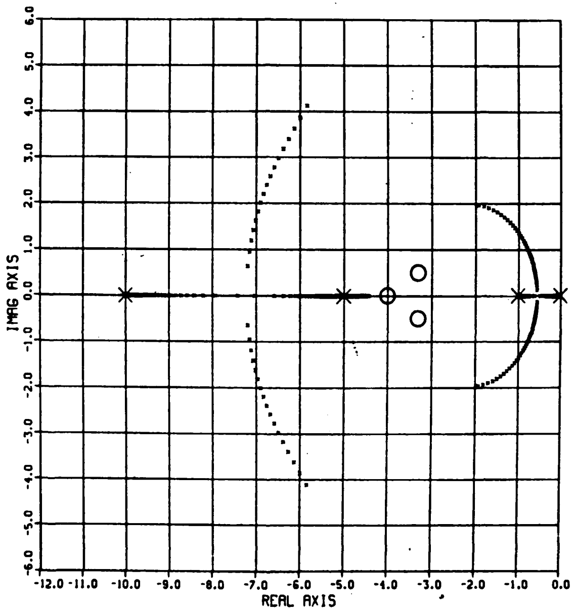
Figure 3.8.c Final Compensated System Root Locus Plot
