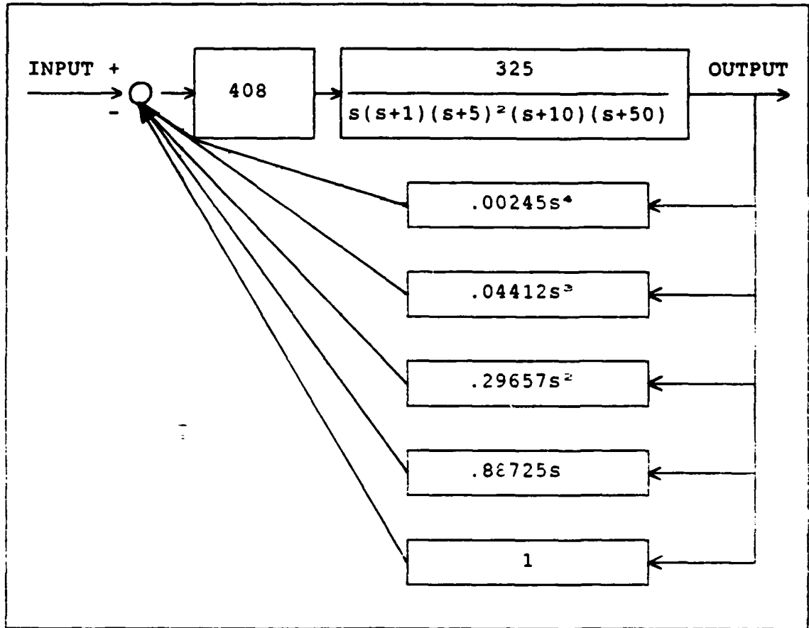
Figure 3.3.f Compensated System Block Diagram
