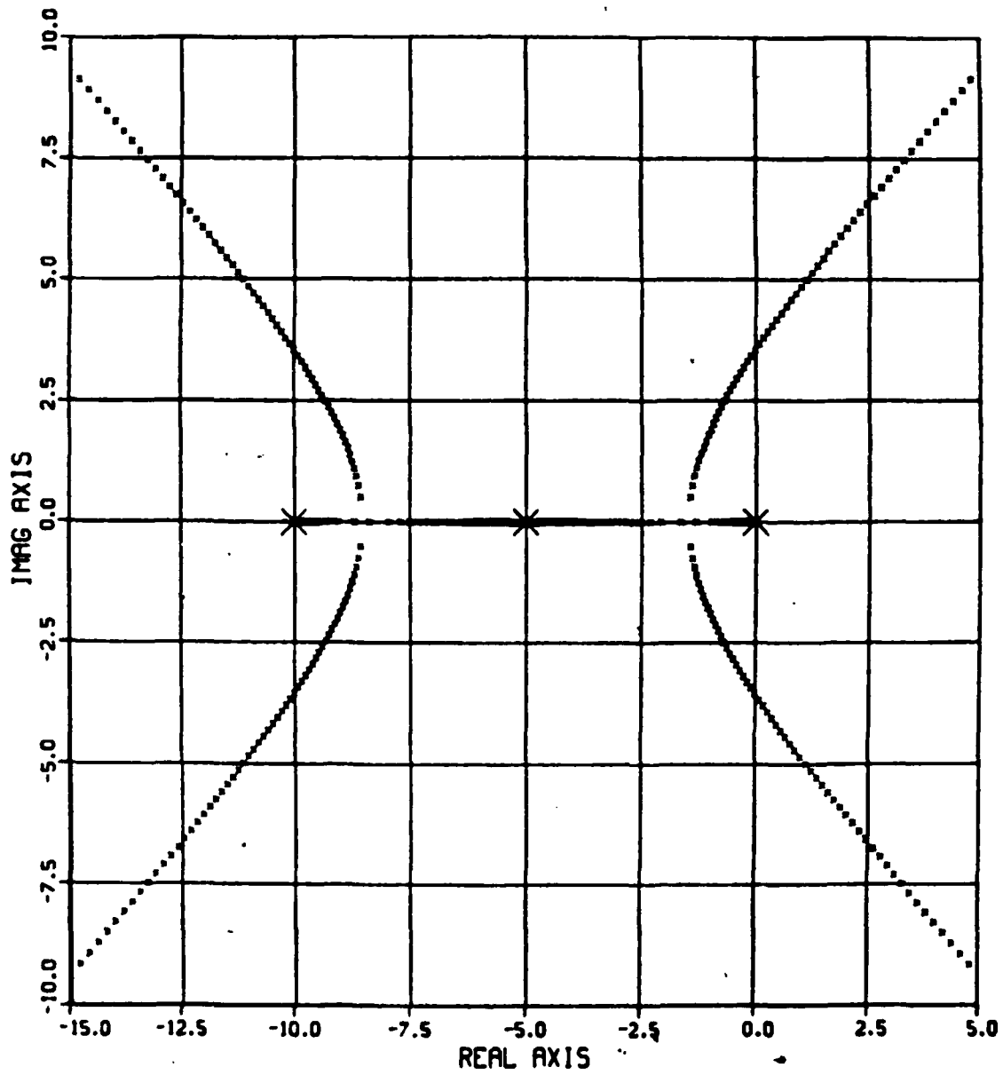
Figure 3.1.a Uncompensated System Root Locus Plot
