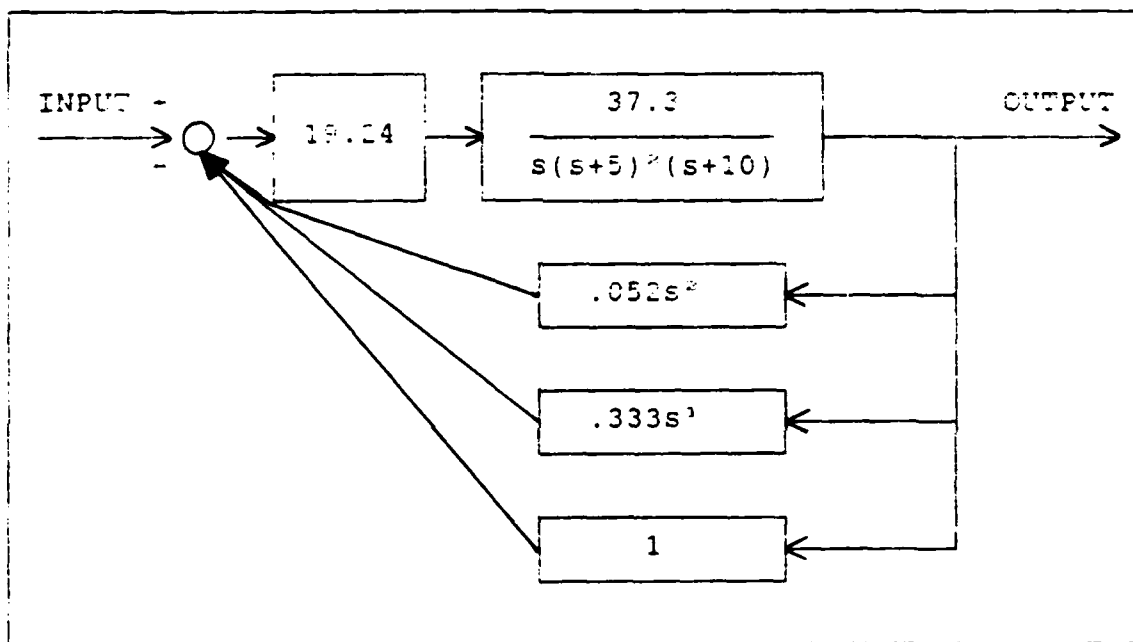
Figure 3.1.f Compensated System Block Diagram
