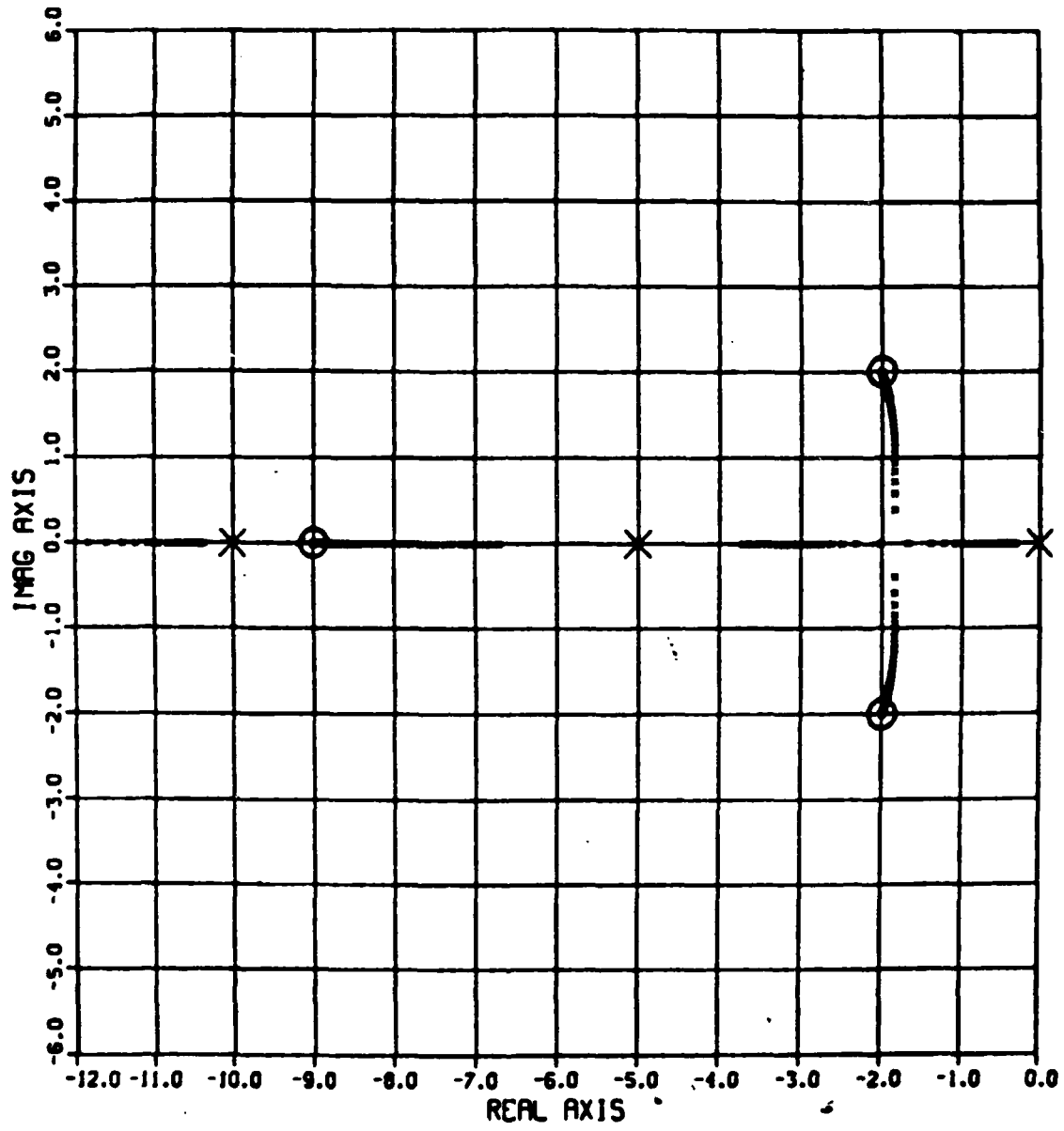
Figure 2.4.b Compensated System Root Loci without Zero Offsets
