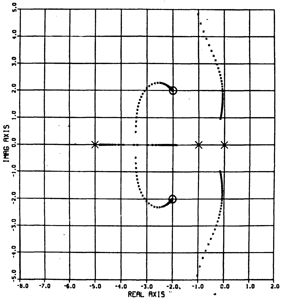
Figure 3.2.b Compensated System Root Locus Plot
