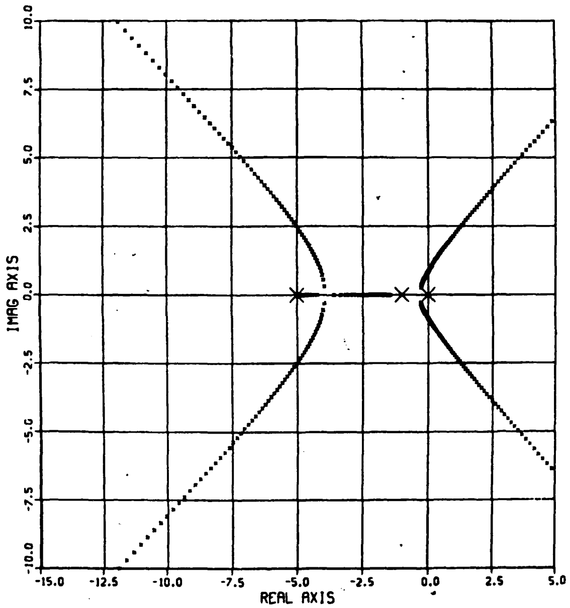
Figure 3.2.a Uncompensated System Root Locus Plot
