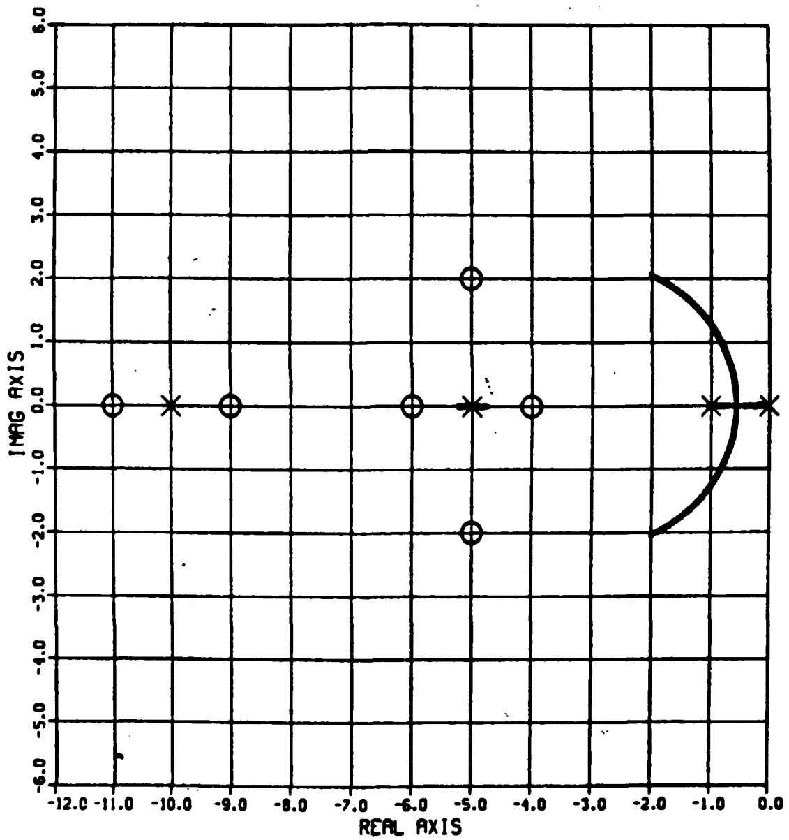
Figure 2.6.e Final Compensated System Root Locus Plot
