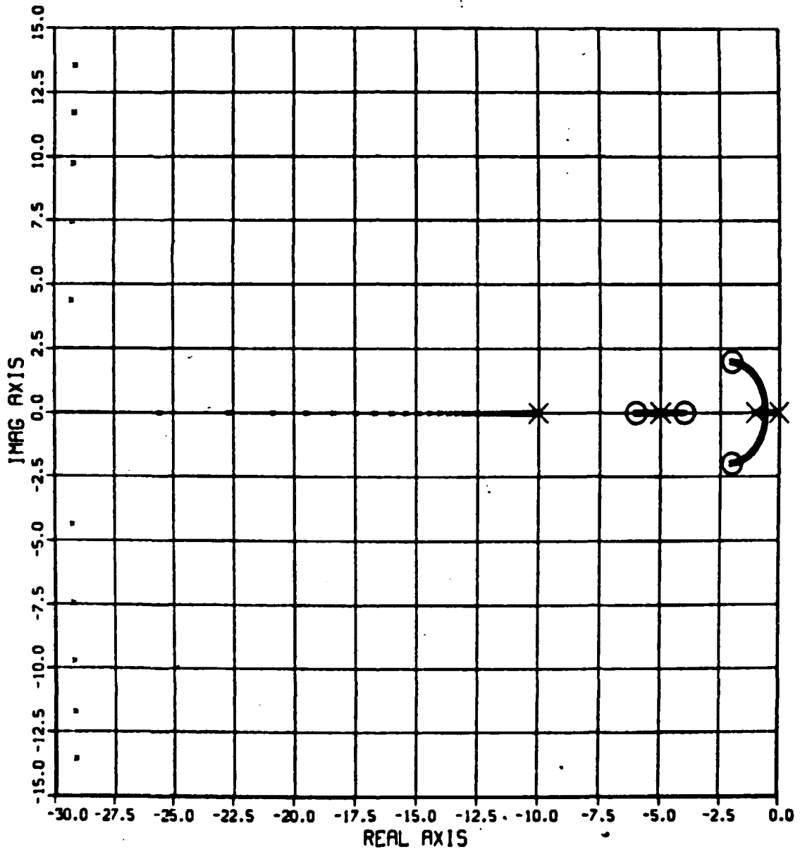
Figure 3.3.b Compensated System Root Loci without Zero Offsets
