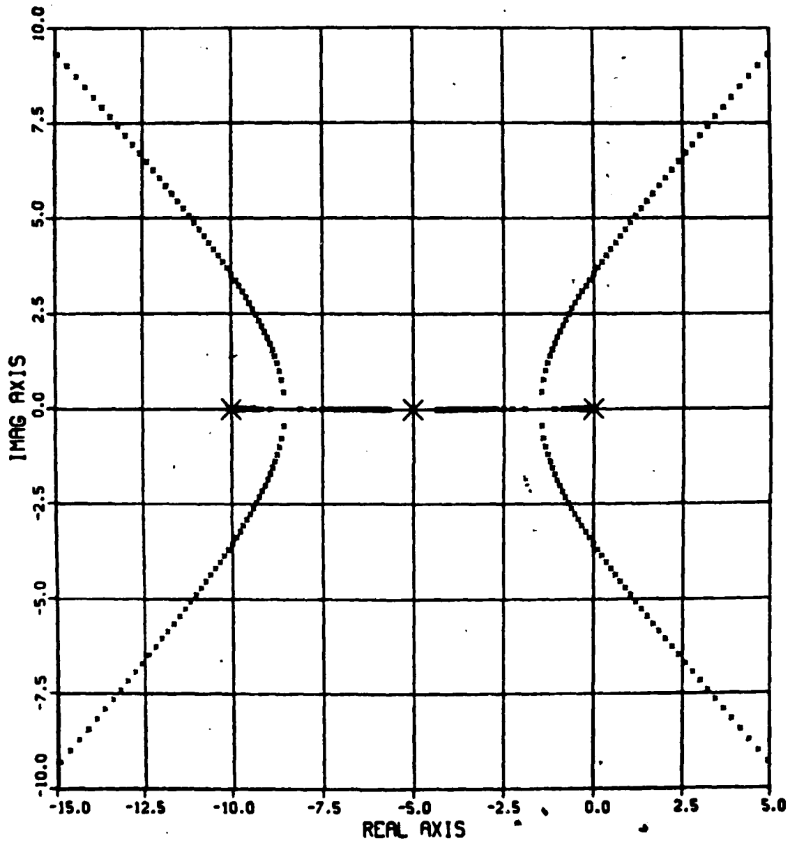
Figure 2.4.a Uncompensated System Root Locus Plot
