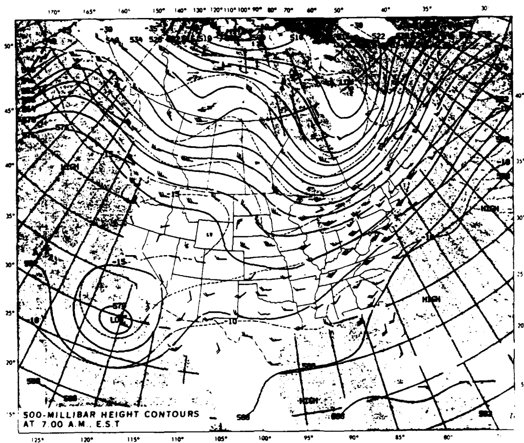
Figure 7. (b.) 500 mb Weather Map for 9 October 1986
