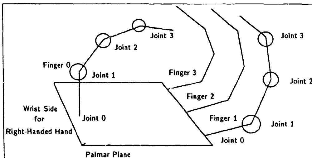
Figure A.1: Numbering of joints on the Utah-MIT hand
