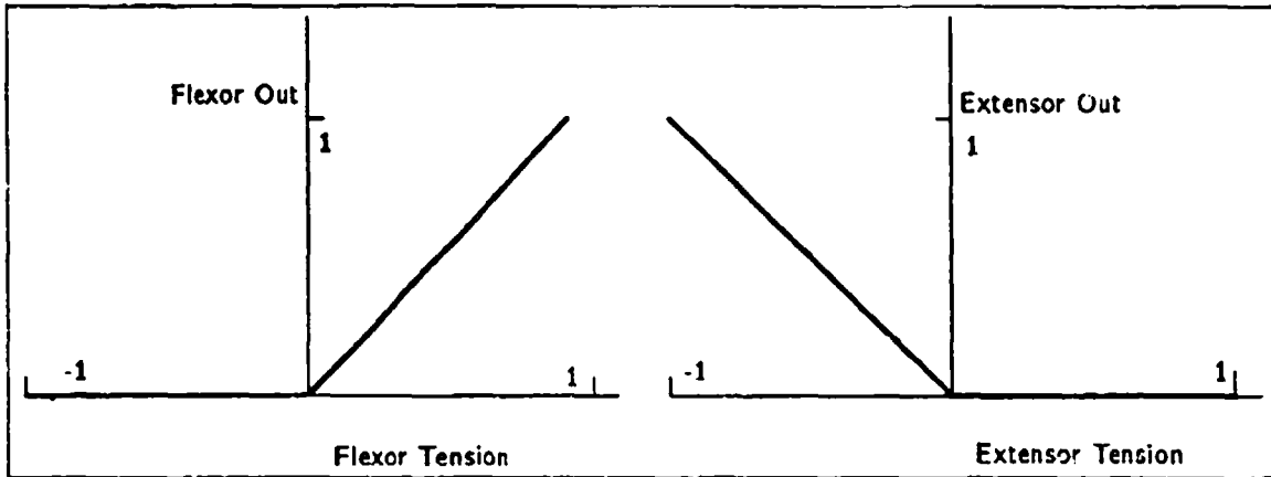
Figure 4.1: Rectification function.
