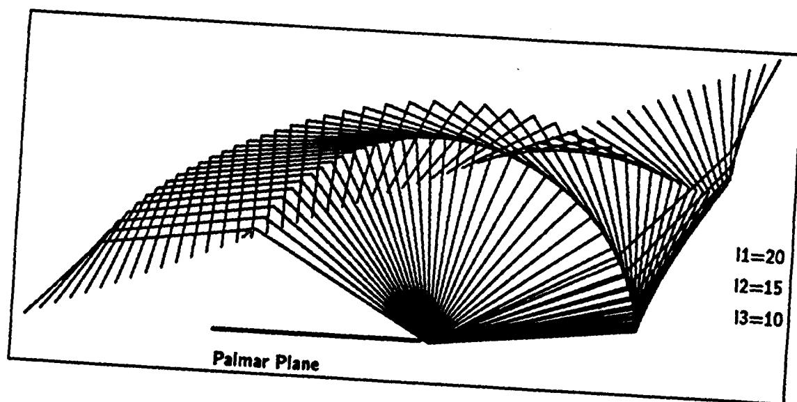
Figure 3.7: Linear trajectory using equal angles constraint.
