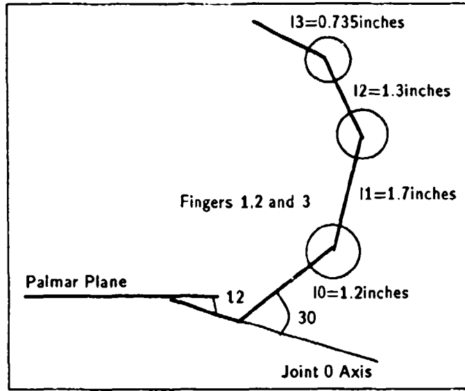
Figure A.2: Single finger - Non thumb
