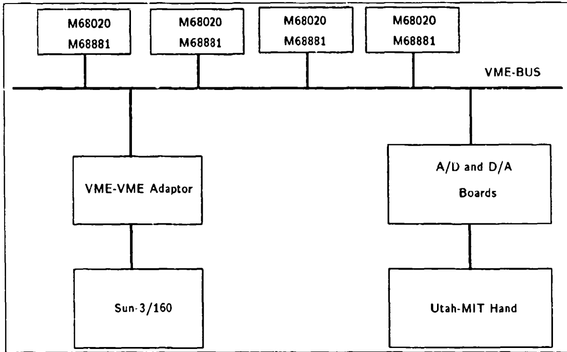
Figure 6.2: Block Diagram of Version II of the hardware.
