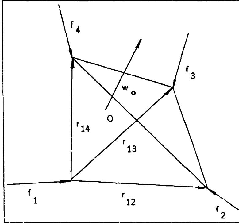
Figure 5.2: Four point contact with friction.
