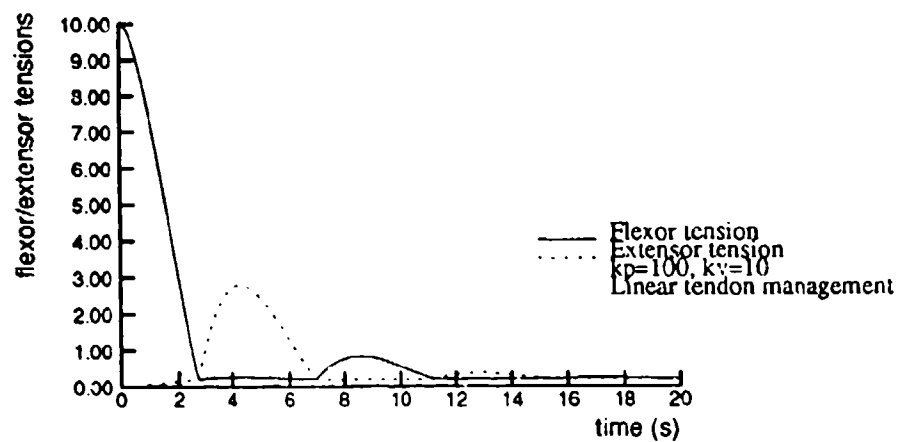
Figure 4.6: Rectification before summing.
