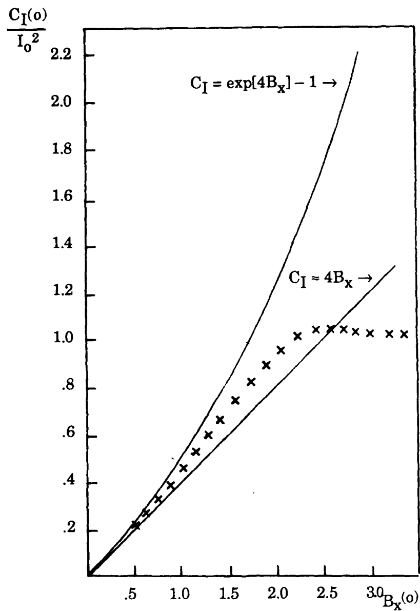
Figure 4. The Normalized Variance of Intensity Scintillations Versus the Log Amplitude Variance for Various Forms for C_I , and Experimental Data Points (x)
