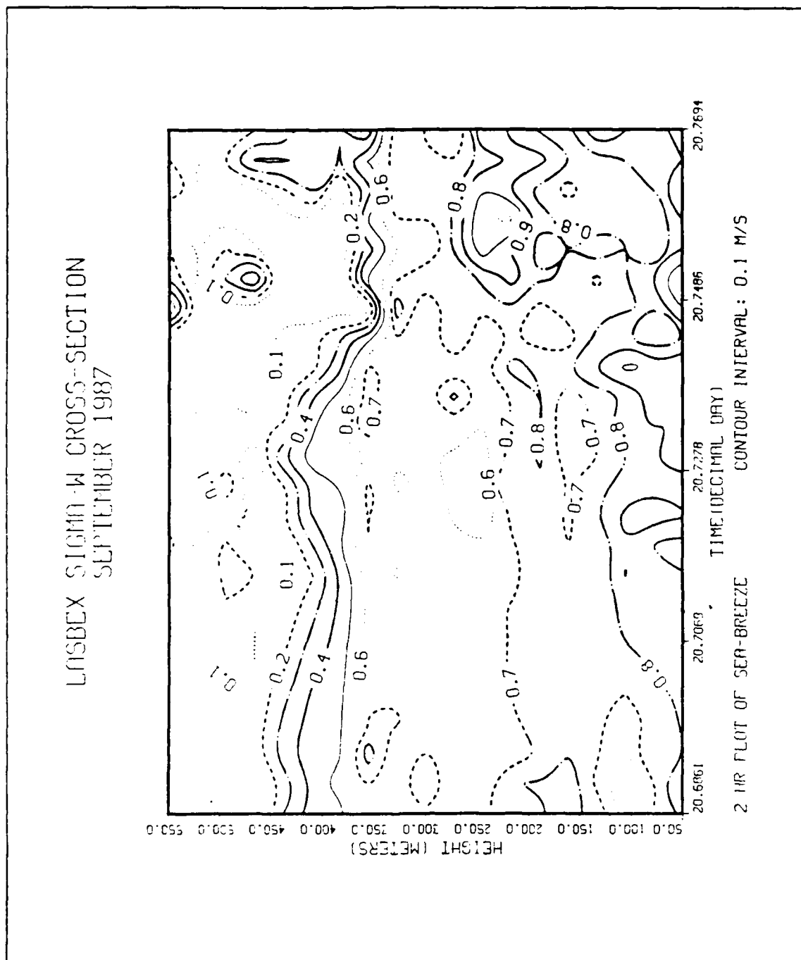
Fig. 59. Two-Hour Standard Deviation Cross Section - 20 September 1987
